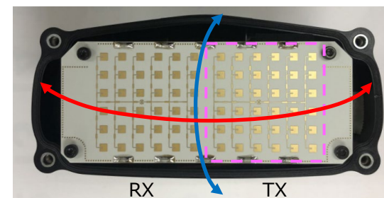
Antenna Plane (with the cover removed)
