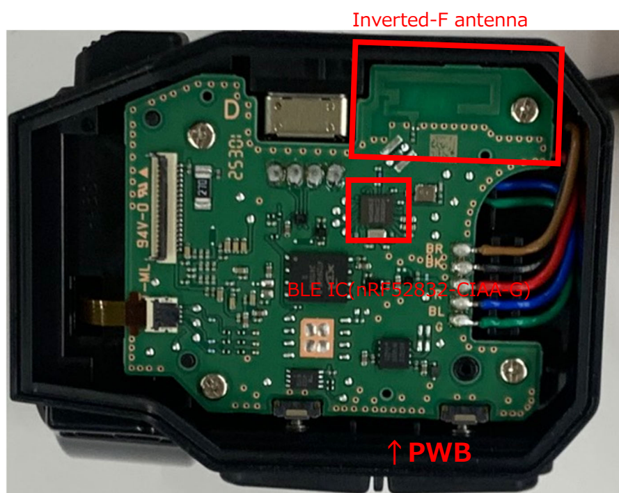
ケース内部基板写真 (Photo of the internal circuit board inside the case)
