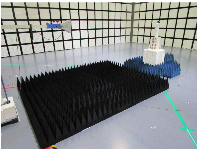
EUT antenna measurement
