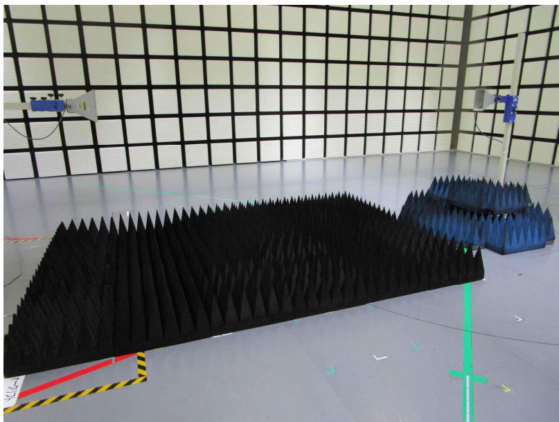
Reference antenna (ID:145501) measurement
