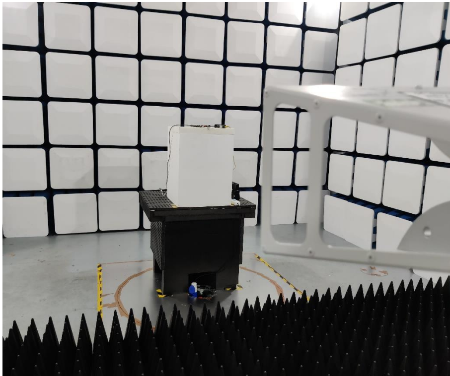
Above 1GHz
