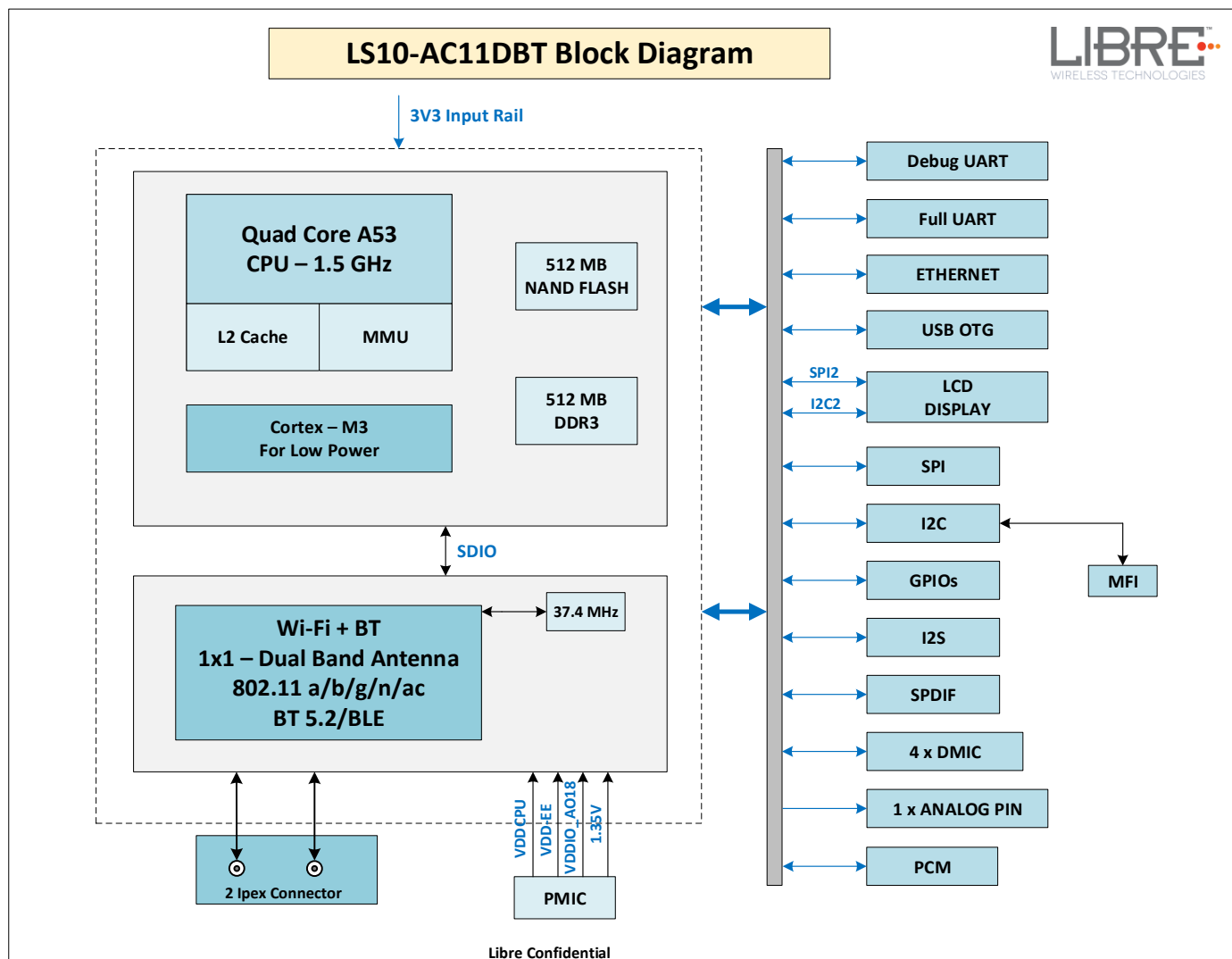
Figure 5-1: LS10 MODULE Block Diagram
