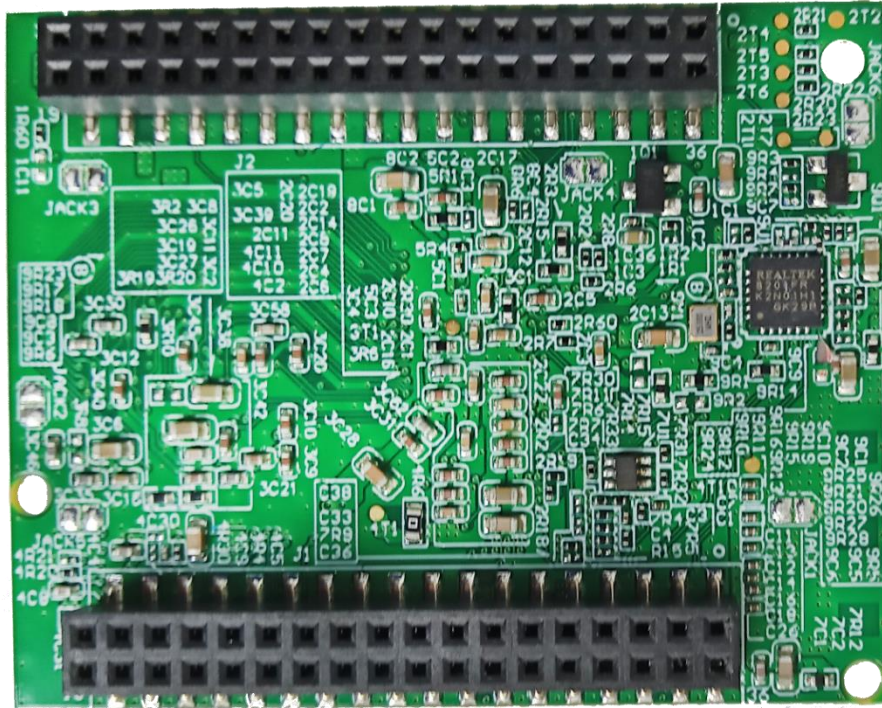
Figure 7.1-2: LS10 Module Bottom View
