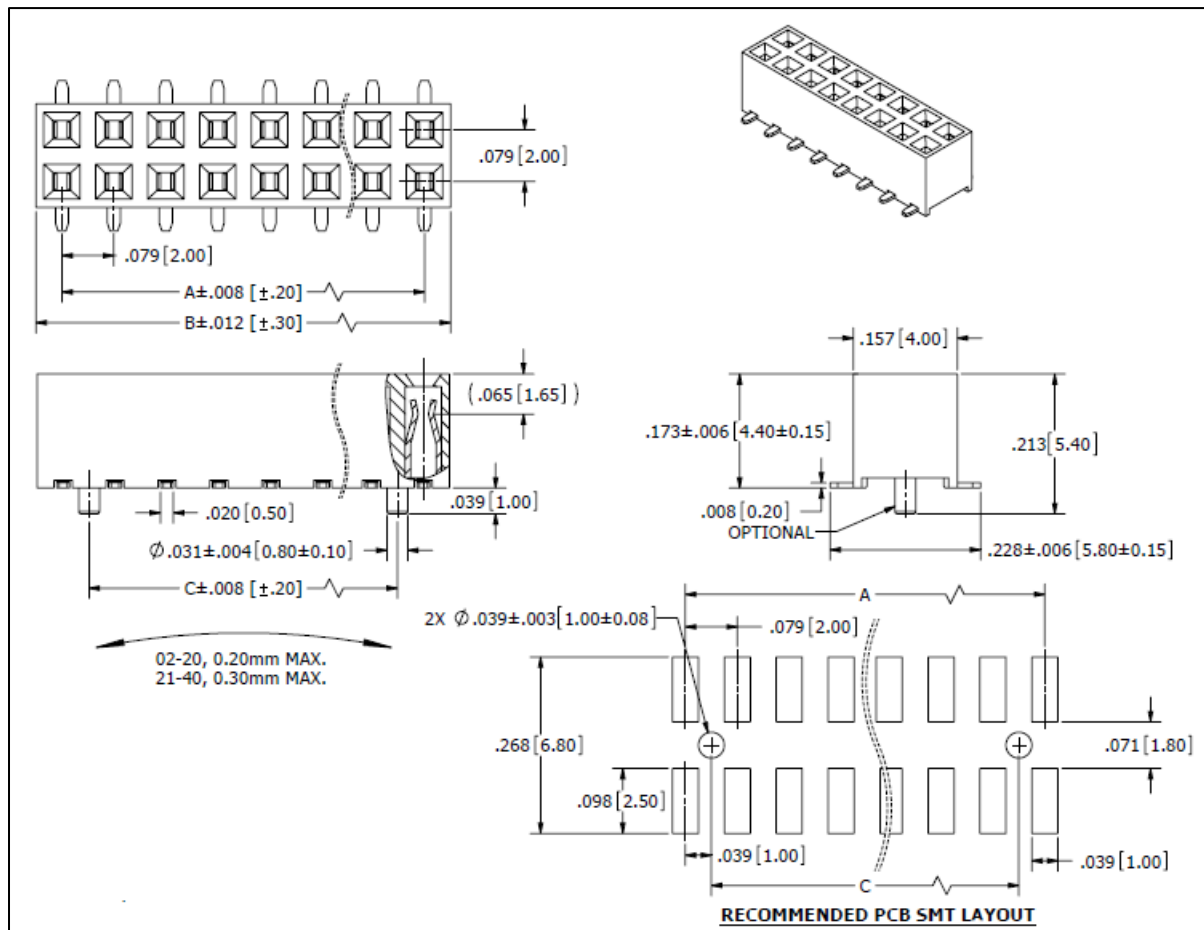
Figure 7.2-1: Media Connector
