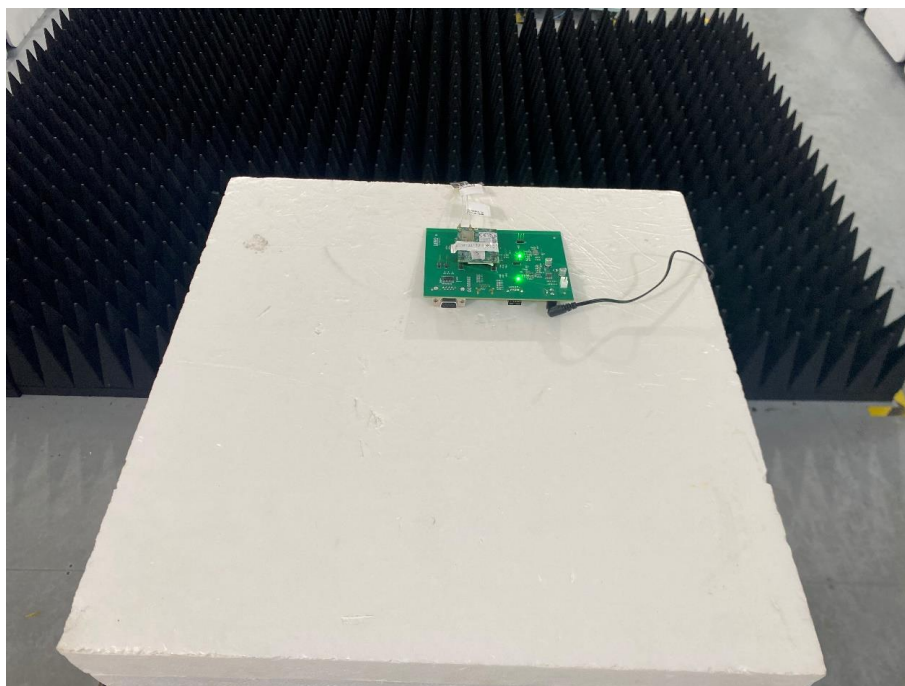
Close-up-FPC Antenna
