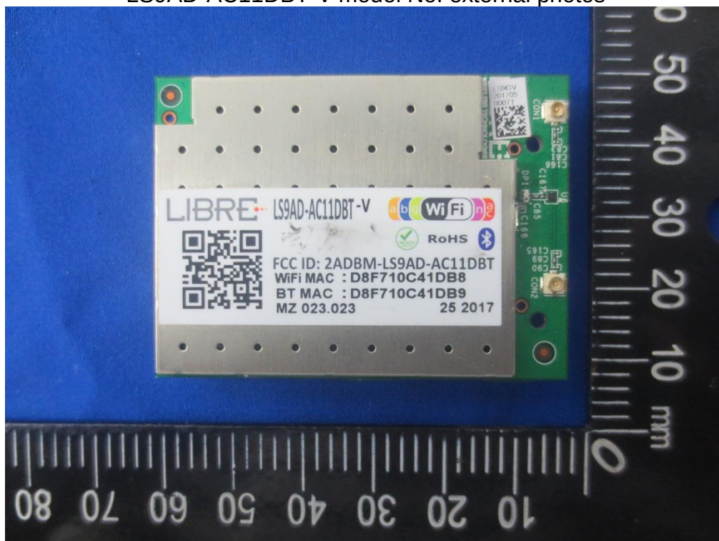
LS9AD-AC11DBT-V model No. external photos
