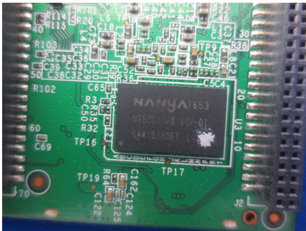
LS9AD-AC11DBT-V model No. internal photos
