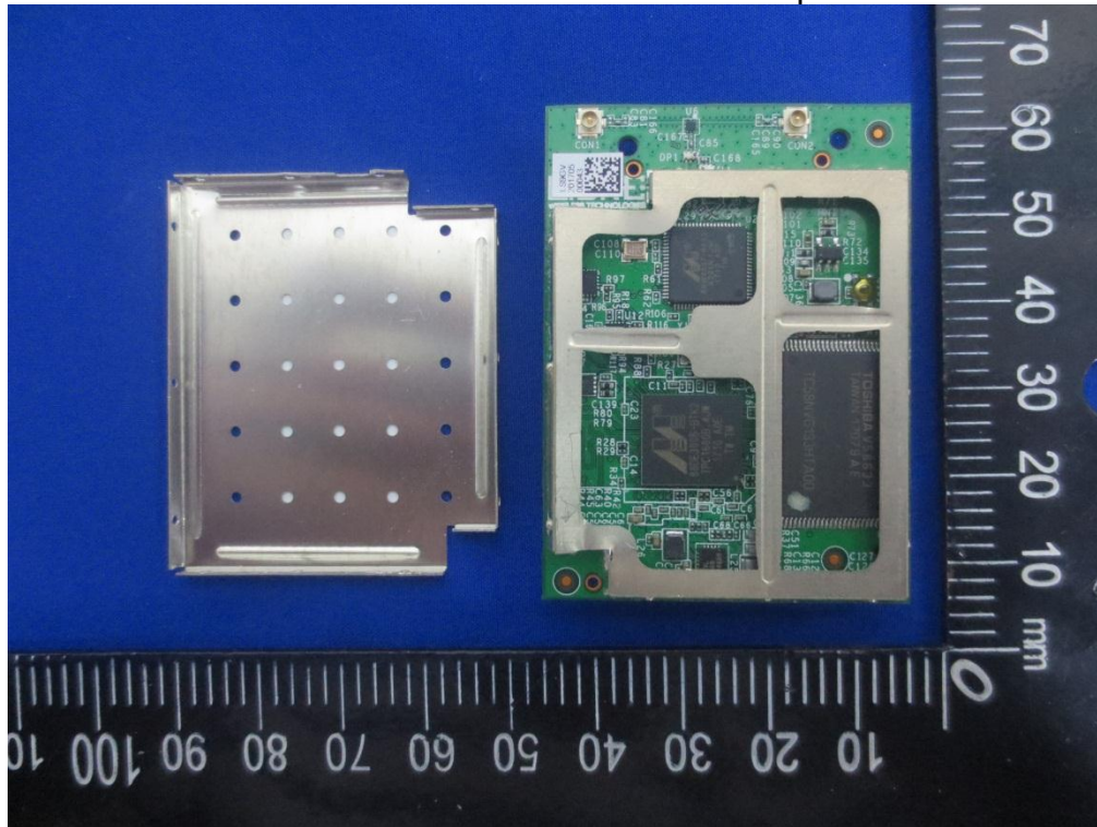
LS9AD-AC11DBT model No. internal photos
