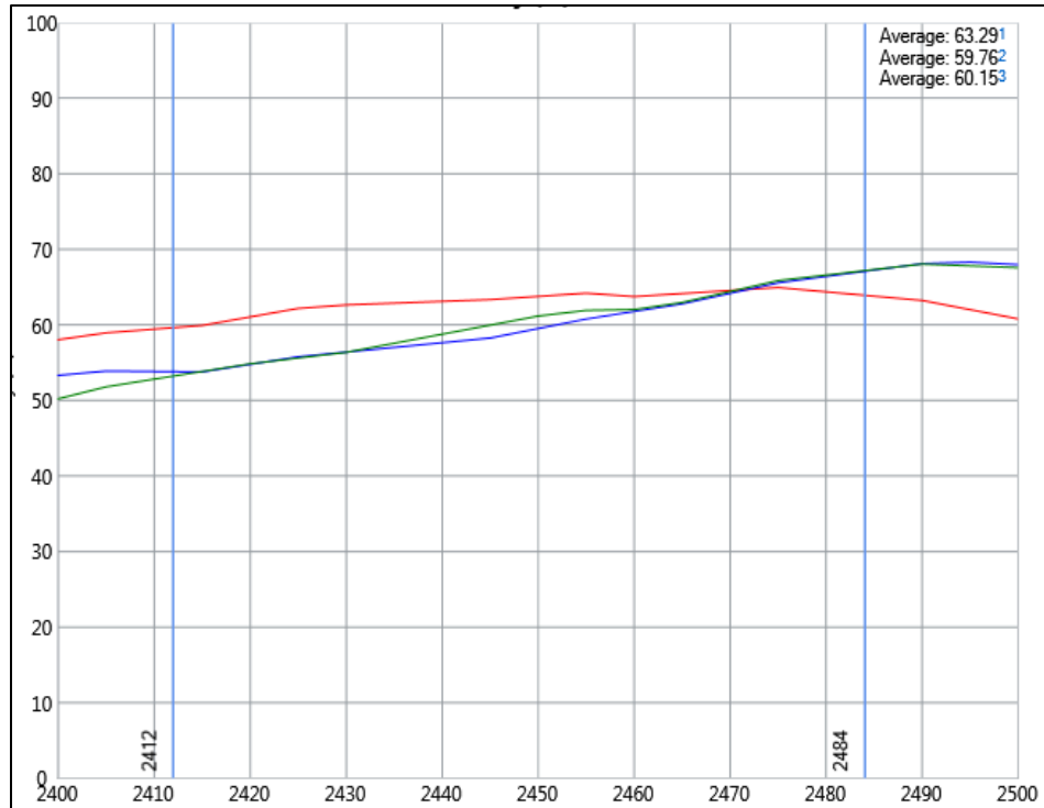
Figure 7.2.1-2 – Efficiency for Product “1B” Variant
