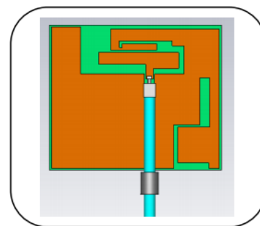
Figure 5.1-2: LSANT-1B-xx product and Simulation model
