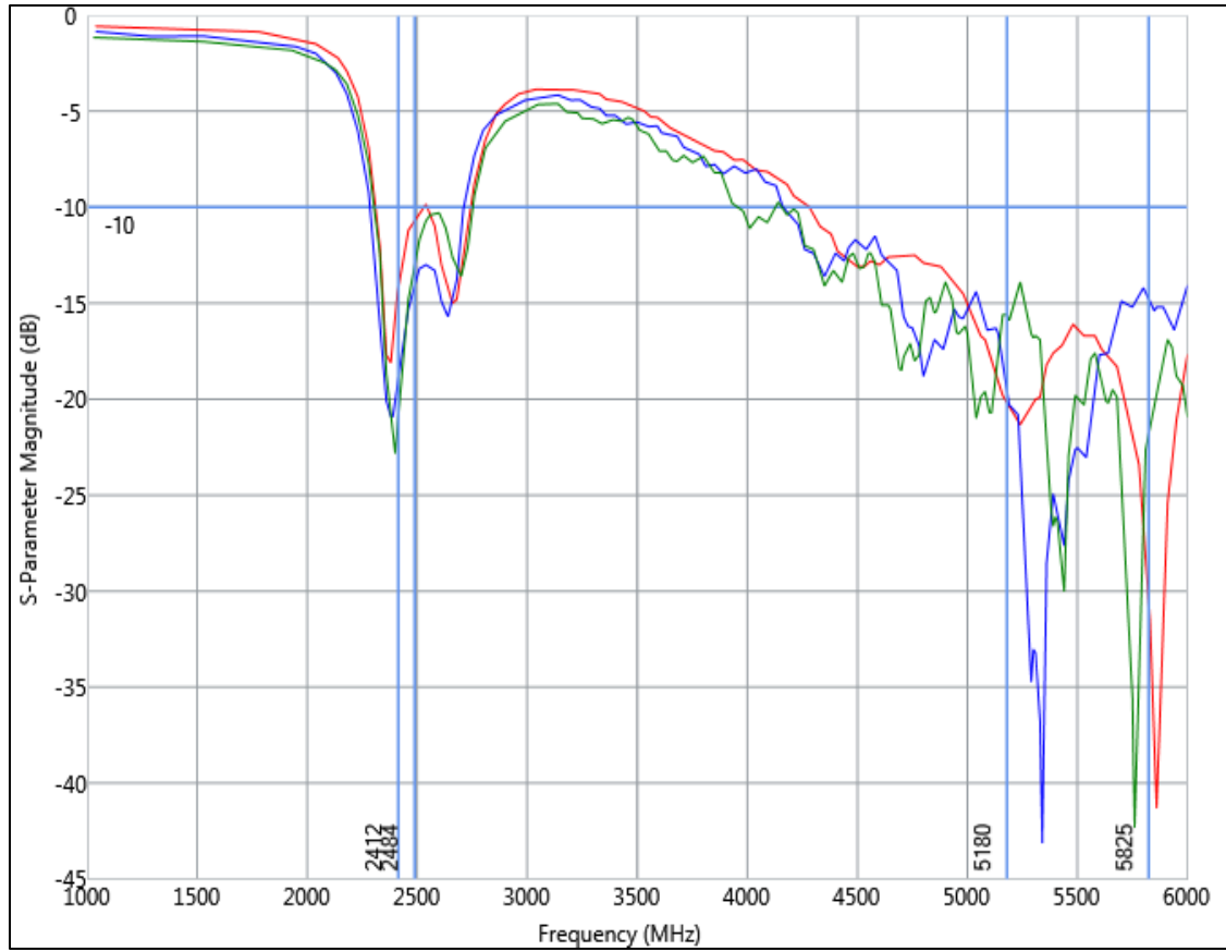
Figure 7.1-1 – Return Loss for Product “1A” Variant
