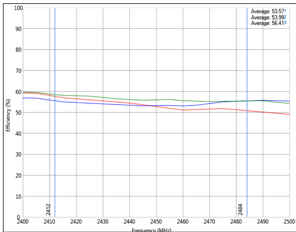
Figure 7.2.1-1 – Efficiency for Product “1A” Variant
