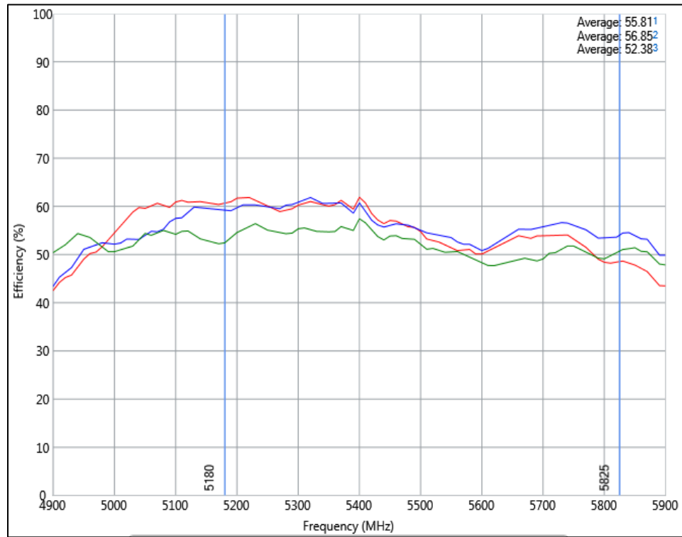
Figure 7.2.2-3 – Efficiency for Product “1C” Variant
