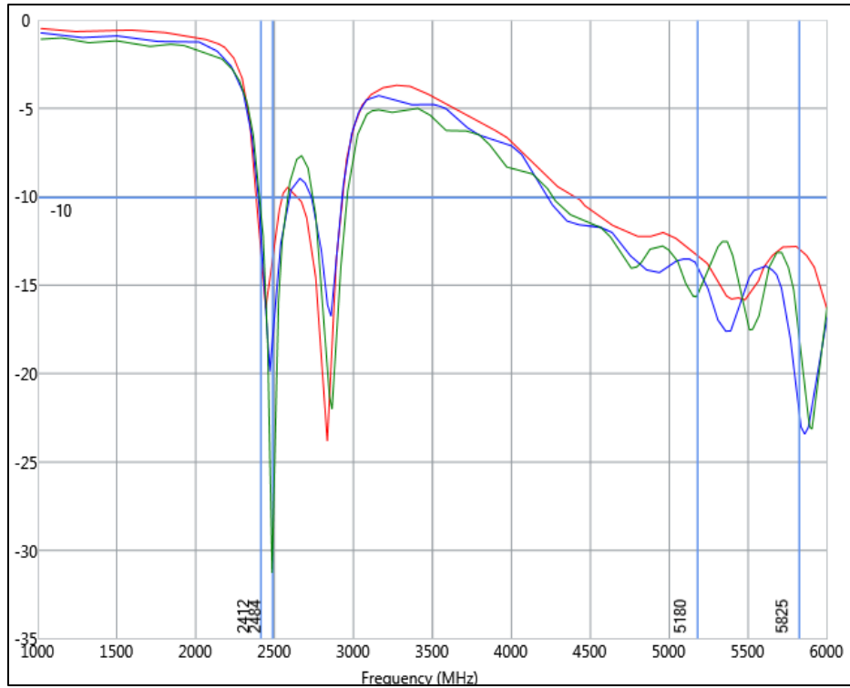
Figure 7.1-2 – Return Loss for Product “1B” Variant
