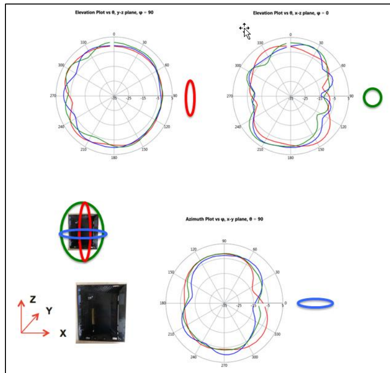
Figure 7.4-2 – Radiation Pattern for Product “1B” Variant
