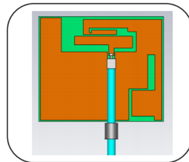
Figure 5.1-1: LSANT-1A-xx product and Simulation model
