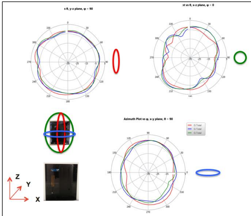
Figure 7.3-3 – Radiation Pattern for Product “1C” Variant
