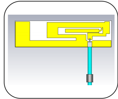
Figure 5.1-3: LSANT-1C-xx product and Simulation model
