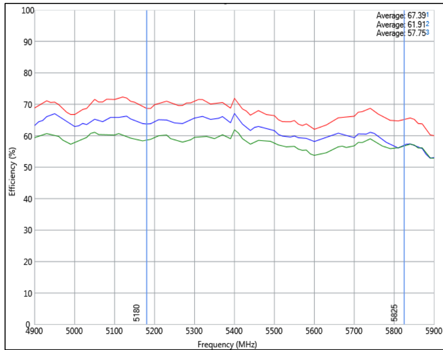
Figure 7.2.2-1 – Efficiency for Product “1A” Variant
