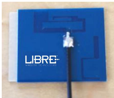
Figure 5.1-1: LSANT-1A-xx product and Simulation model
