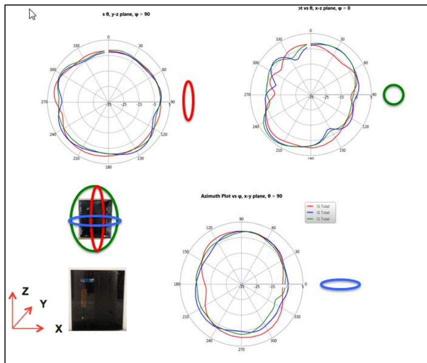
Figure 7.4-3 – Radiation Pattern for Product “1C” Variant
