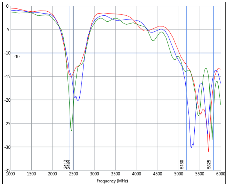
Figure 7.1-3 – Return Loss for Product “1C” Variant
