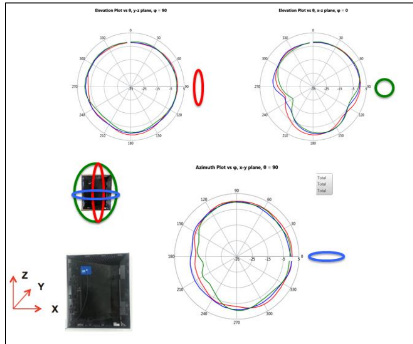
Figure 7.4-1 – Radiation Pattern for Product “1A” Variant
