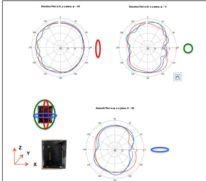
Figure 7.3-2 – Radiation Pattern for Product “1B” Variant
