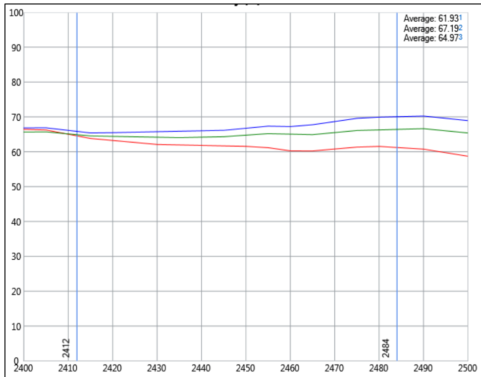
Figure 7.2.1-3 – Efficiency for Product “1C” Variant
