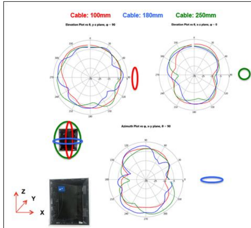
Figure 7.3-1 – Radiation Pattern for Product “1A” Variant
