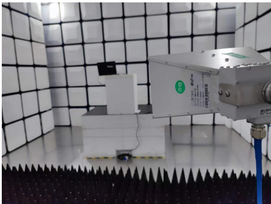
Above 1GHz-BLE
