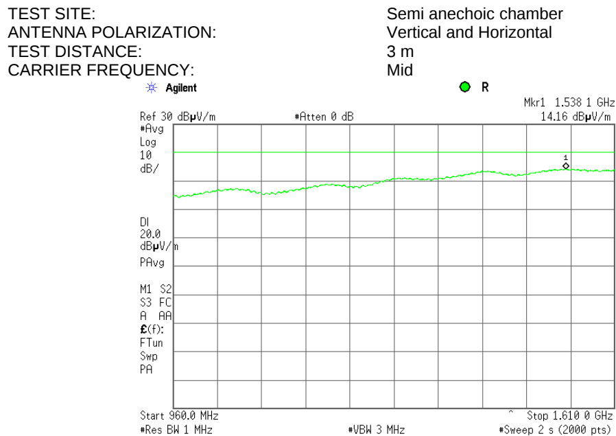
Plot 7.3.5 Radiated emission measurements in 960 – 1610 MHz range
