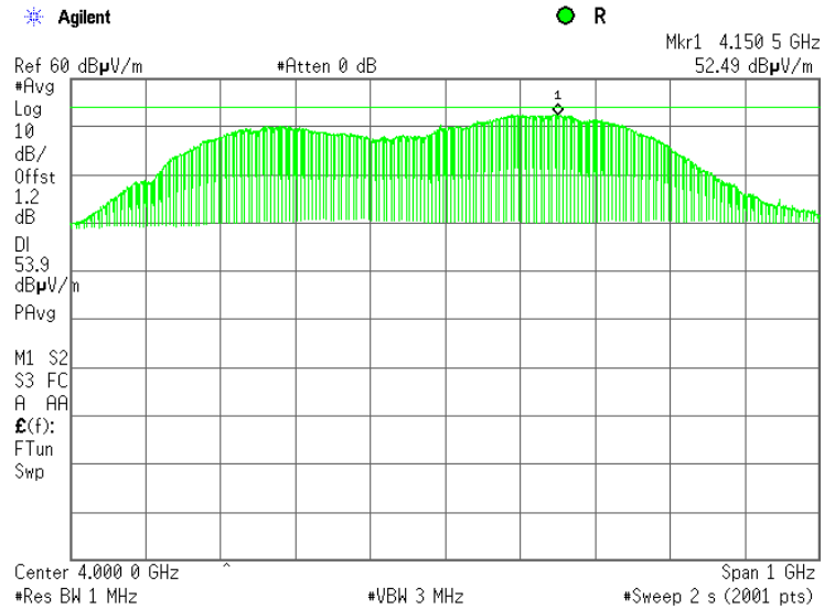
Plot 7.1.2 Power spectral density at mid frequency
