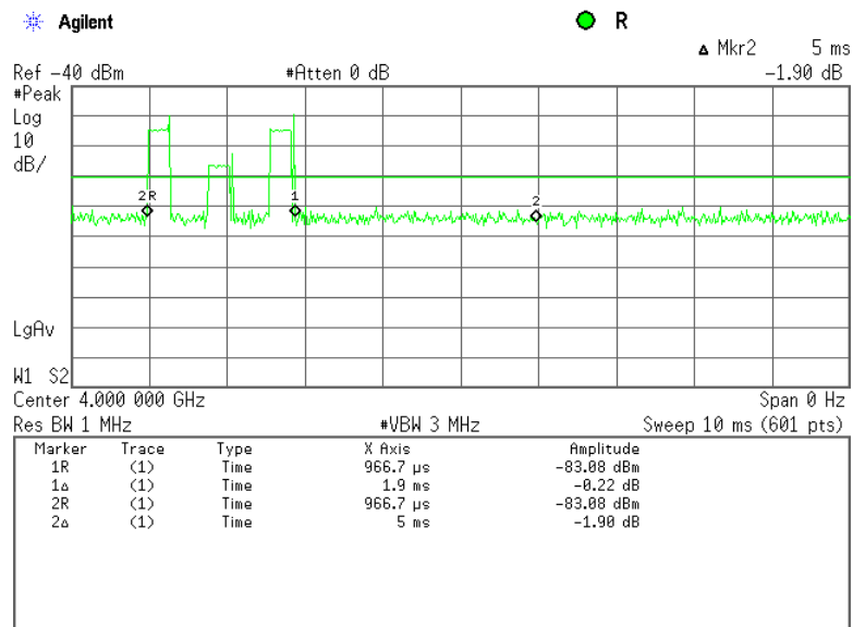
Plot 7.5.2 RF transmission period
