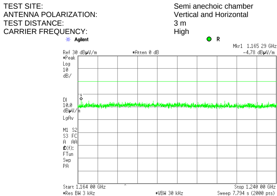
Plot 7.3.9 Radiated emission measurements in 1164 – 1240 MHz range
