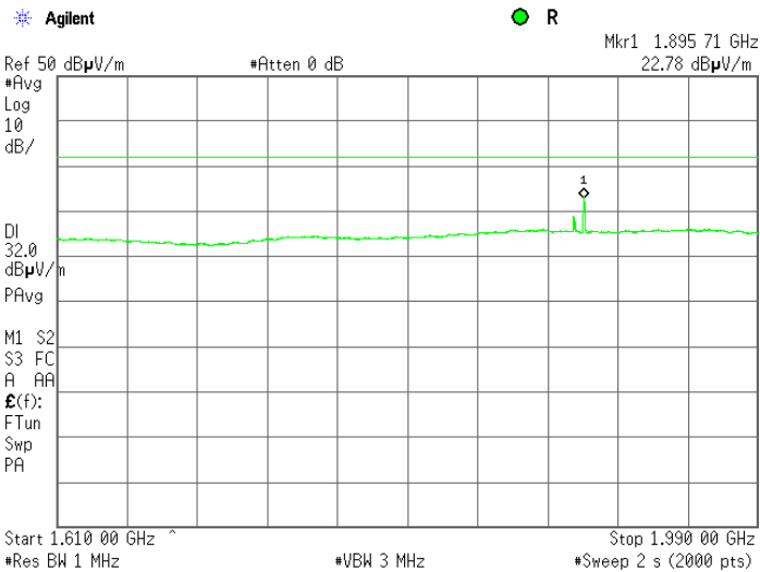
Plot 7.3.15 Radiated emission measurements in 1610 – 1990 MHz range
