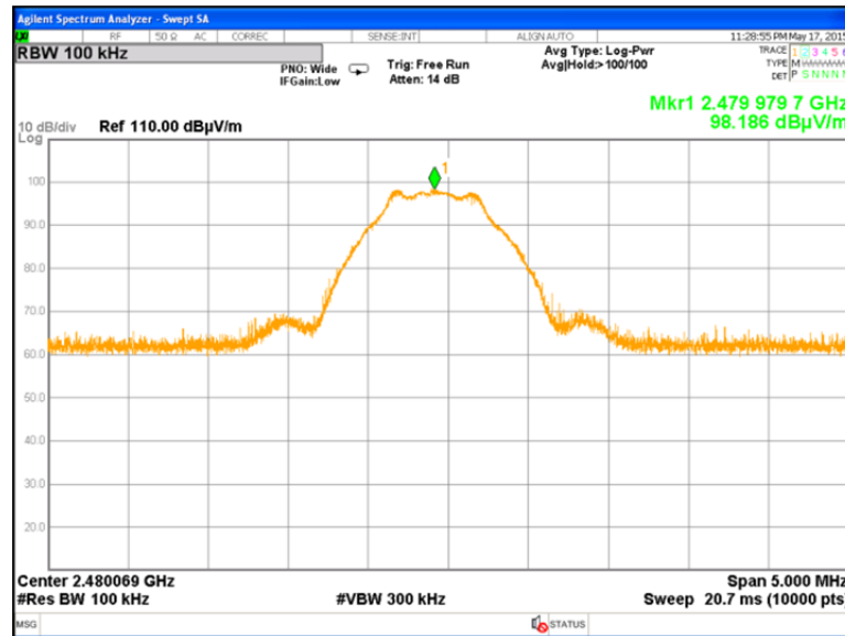
Plot 7.5.3 Peak spectral power density at high frequency zoomed at the peak
