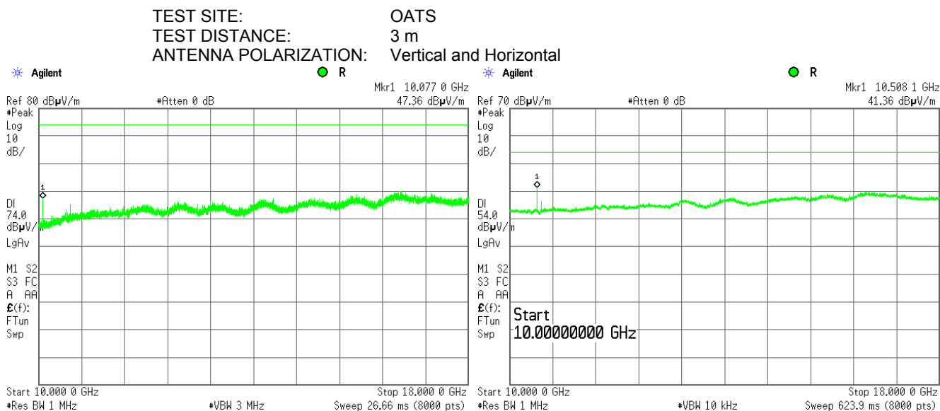
Plot 7.3.14 Radiated emission measurements from 10000 to 18000 MHz at the mid carrier frequency
