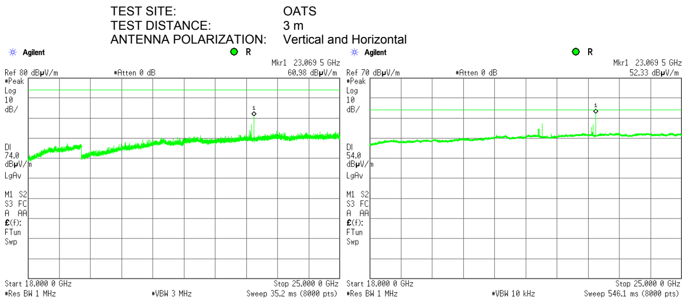
Plot 7.3.16 Radiated emission measurements from 18000 to 25000 MHz at the low carrier frequency
