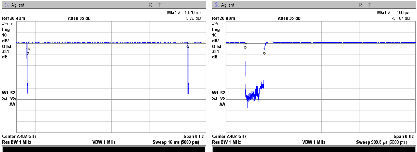
Plot 7.3.19 Transmission pulse duration
