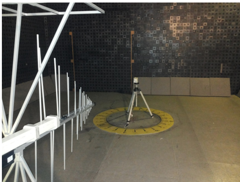
Photograph 8.1.2 Setup for radiated emission measurements in the anechoic chamber
