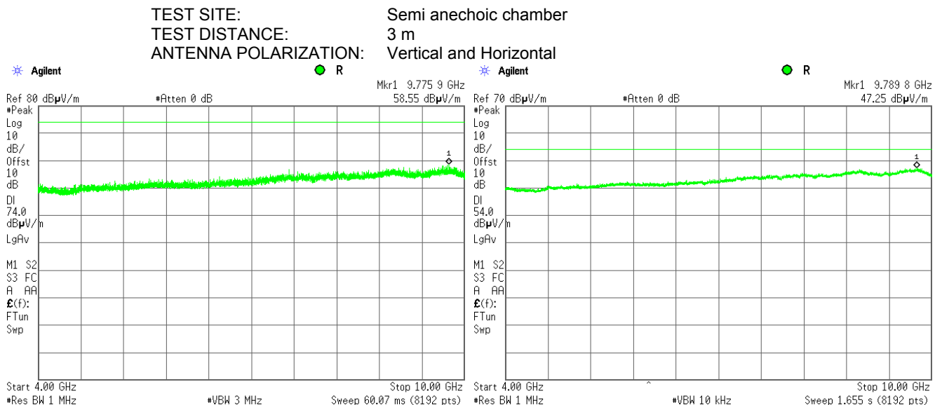
Plot 7.3.11 Radiated emission measurements from 4000 to 10000 MHz at the mid carrier frequency
