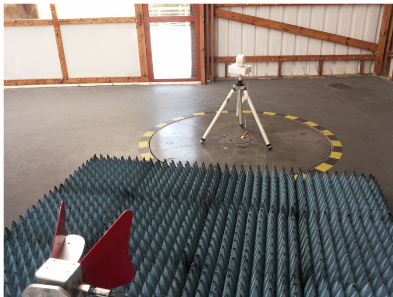
Photograph 8.1.4 Setup for final radiated emission measurements at the OATS
