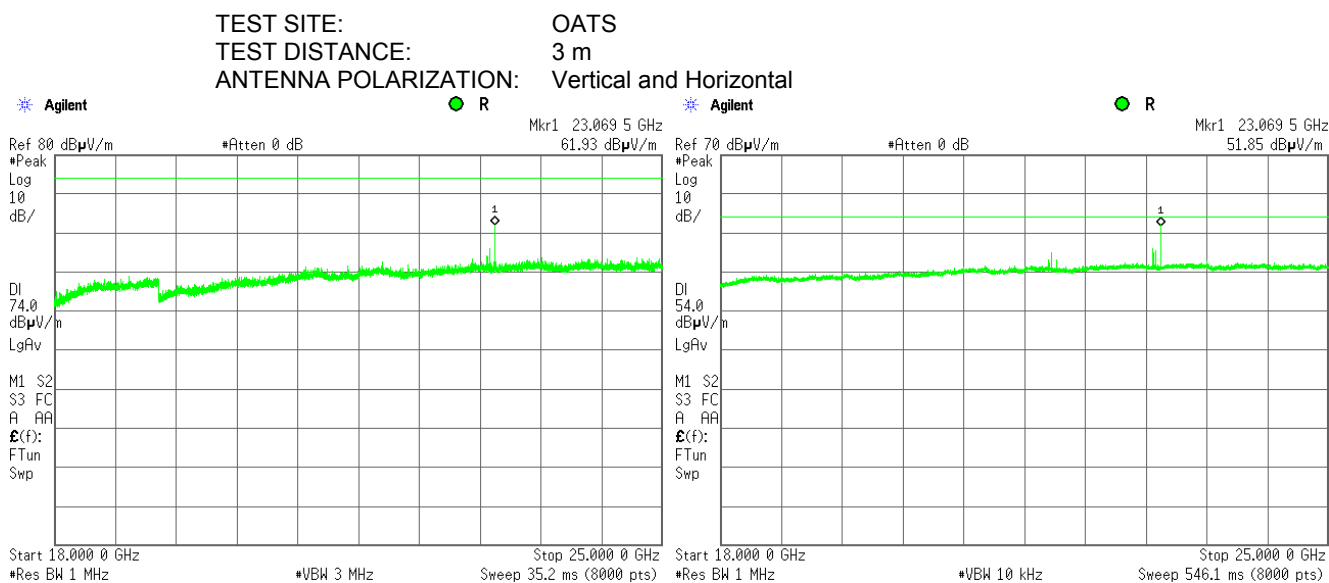
Plot 7.3.17 Radiated emission measurements from 18000 to 25000 MHz at the mid carrier frequency
