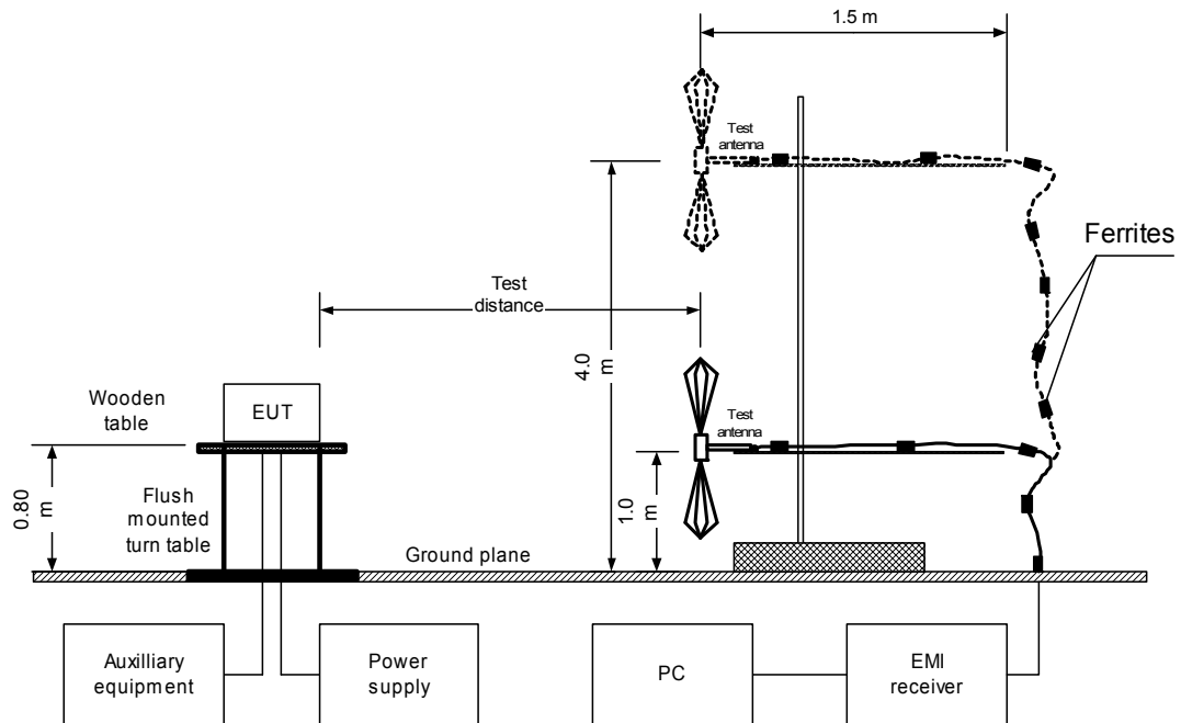
Figure 8.1.2 Setup for radiated emission measurements at OATS, table-top EUT
