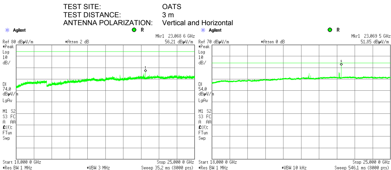
Plot 7.3.18 Radiated emission measurements from 18000 to 25000 MHz at the high carrier frequency
