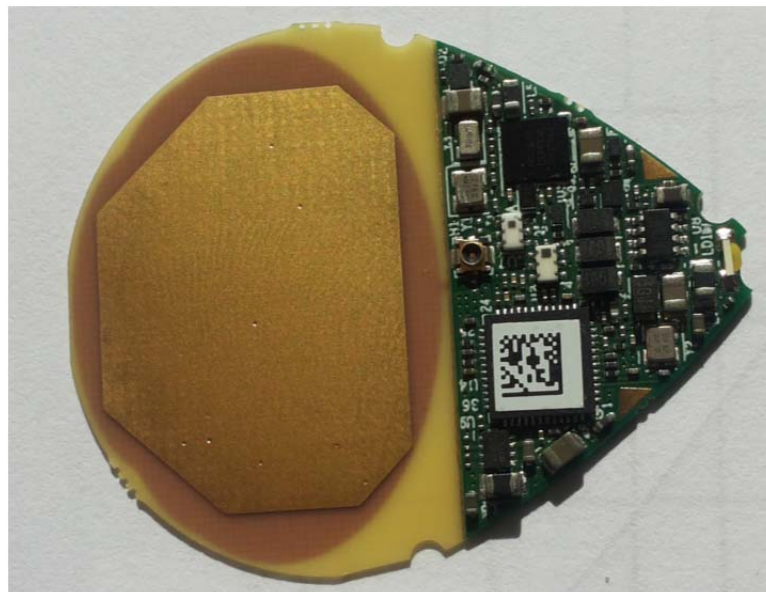
Photograph 7.6.1 Antenna assembly
