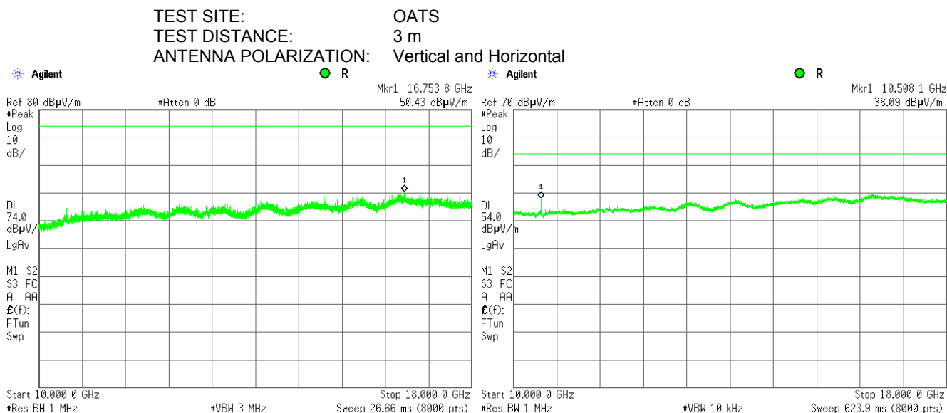
Plot 7.3.15 Radiated emission measurements from 10000 to 18000 MHz at the high carrier frequency
