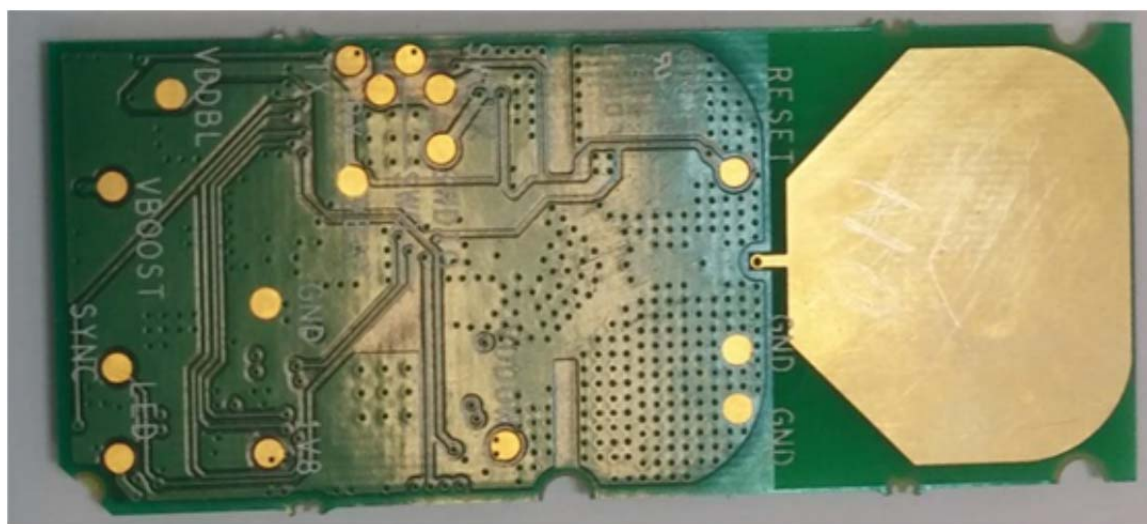
Photograph 7.6.1 Antenna view
