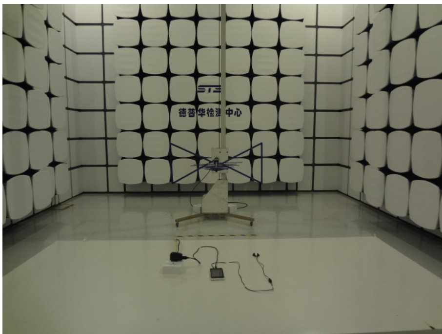
Part 15C radiation L
