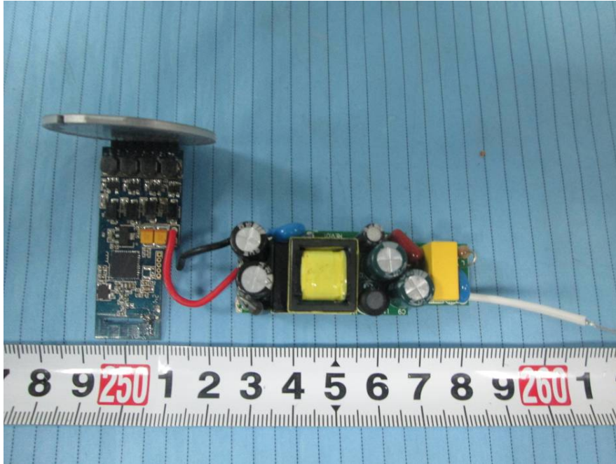
EUT – Main Board All View
