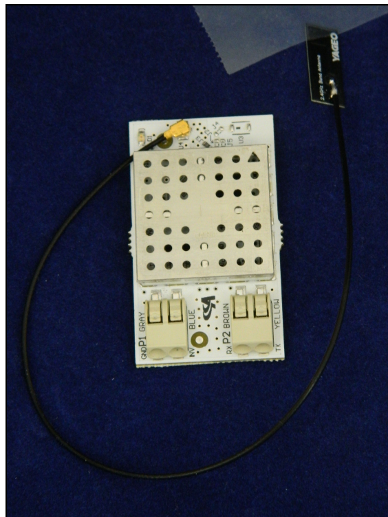
Figure 4: External Photo – PIFA
