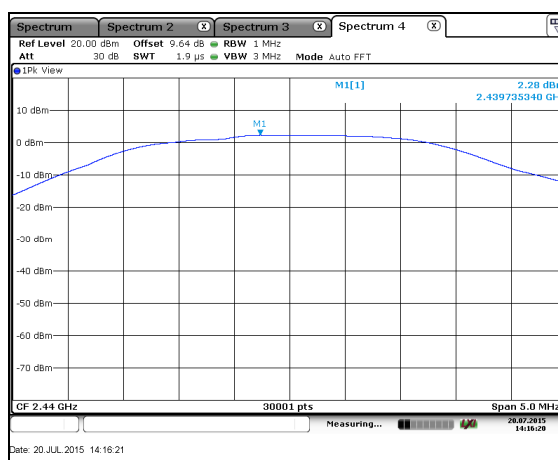
Figure 7.4.2-2: Peak Output Power – MCH
