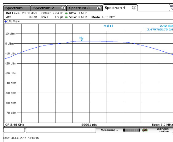
Figure 7.4.2-3: Peak Output Power – HCH
