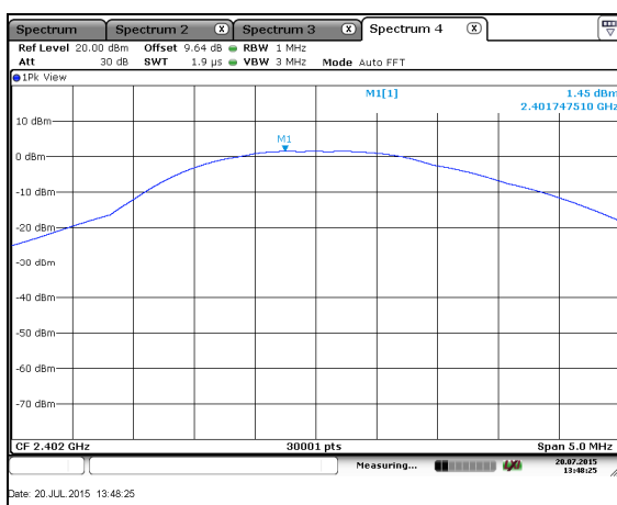
Figure 7.4.2-1: Peak Output Power – LCH
