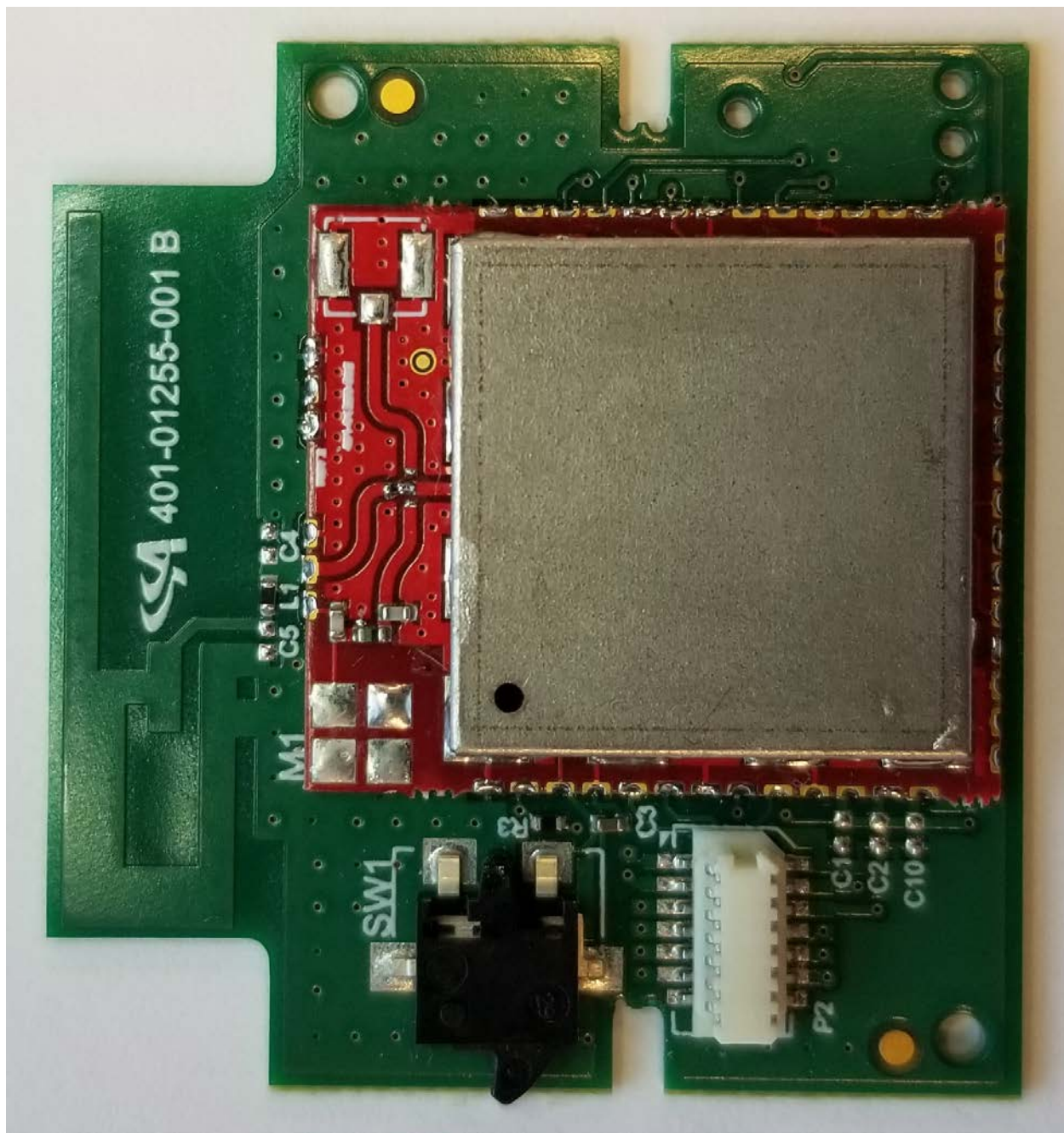
Figure 1: BMODIT Module with PIFA Antenna
