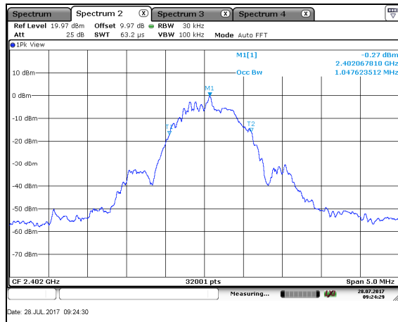
Figure 7.3.2-4: 99% OBW – LCH
