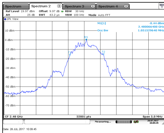
Figure 7.3.2-6: 99% OBW – HCH
