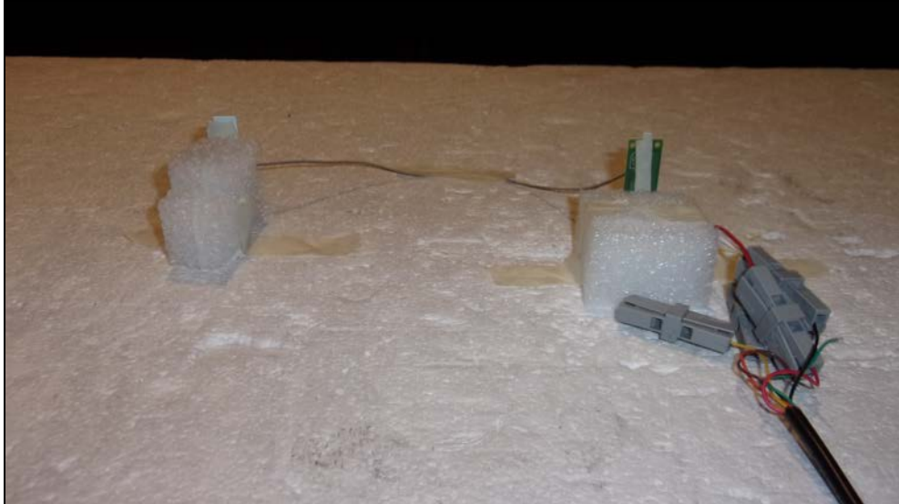
Figure 8: Radiated Emissions – External Antenna XPOS
