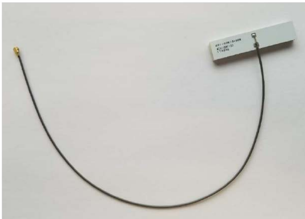
Figure 2: Flag Antenna
