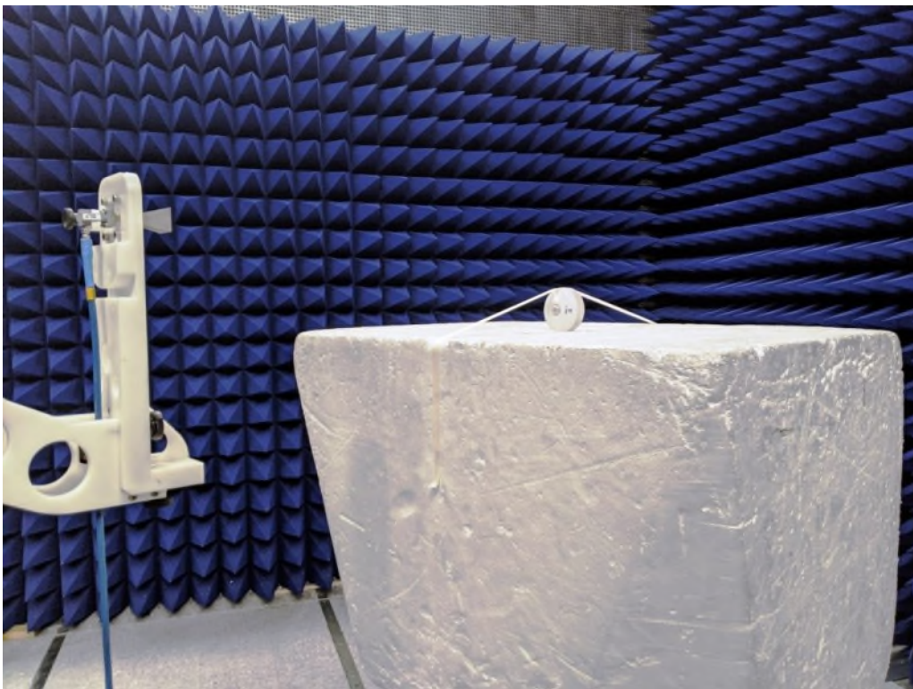
Figure 8: Equipment Under Test – Radiated Emissions >18GHz
