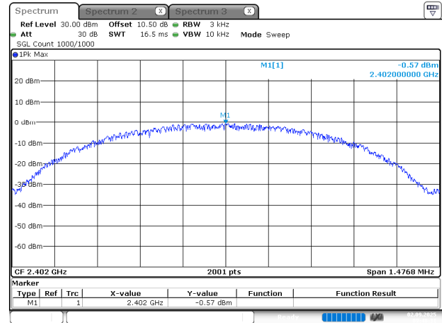
BLE_1M_Low_Channel
