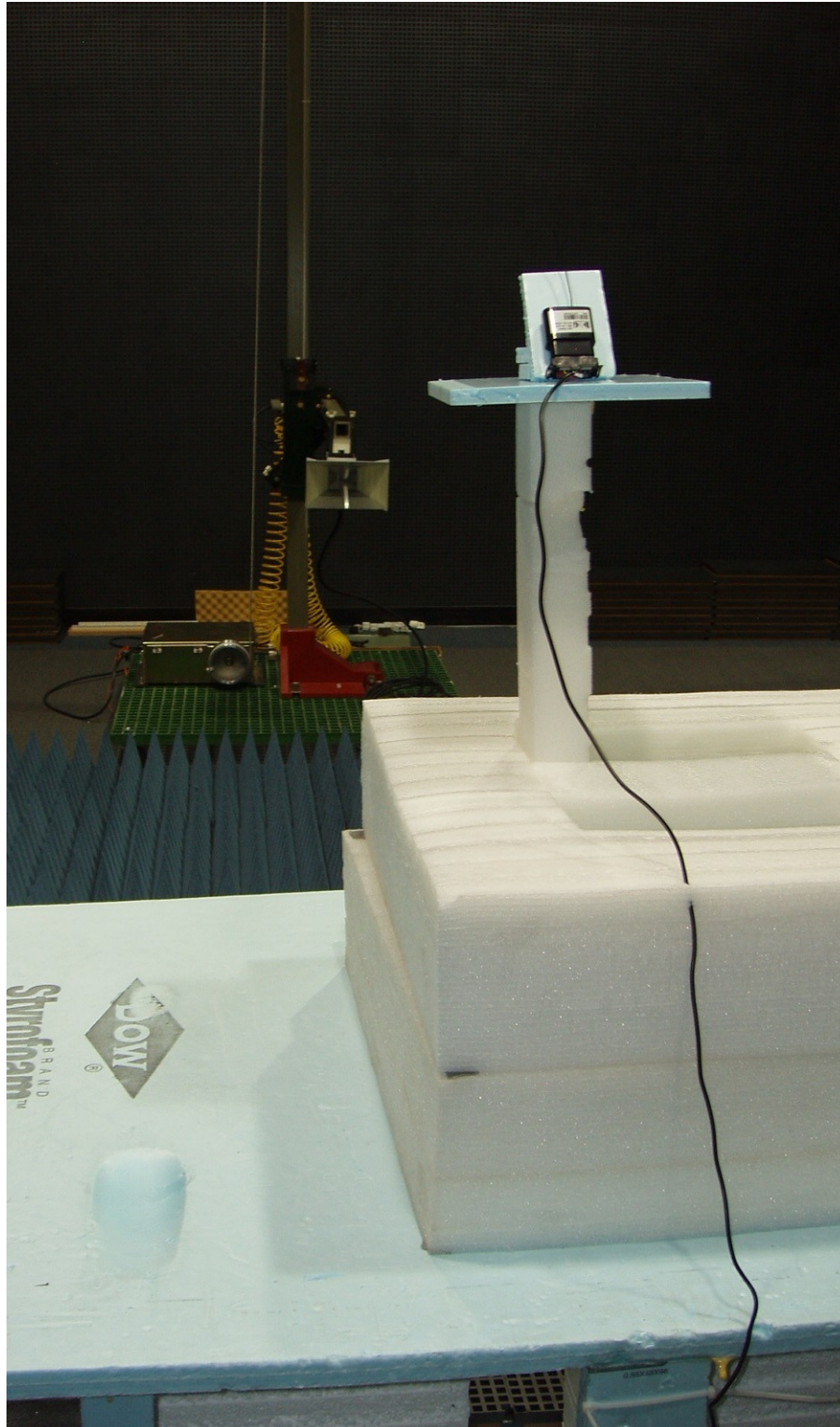
Photo 4 – Rear View of the Radiated Emissions Test Set-up above 1 GHz
