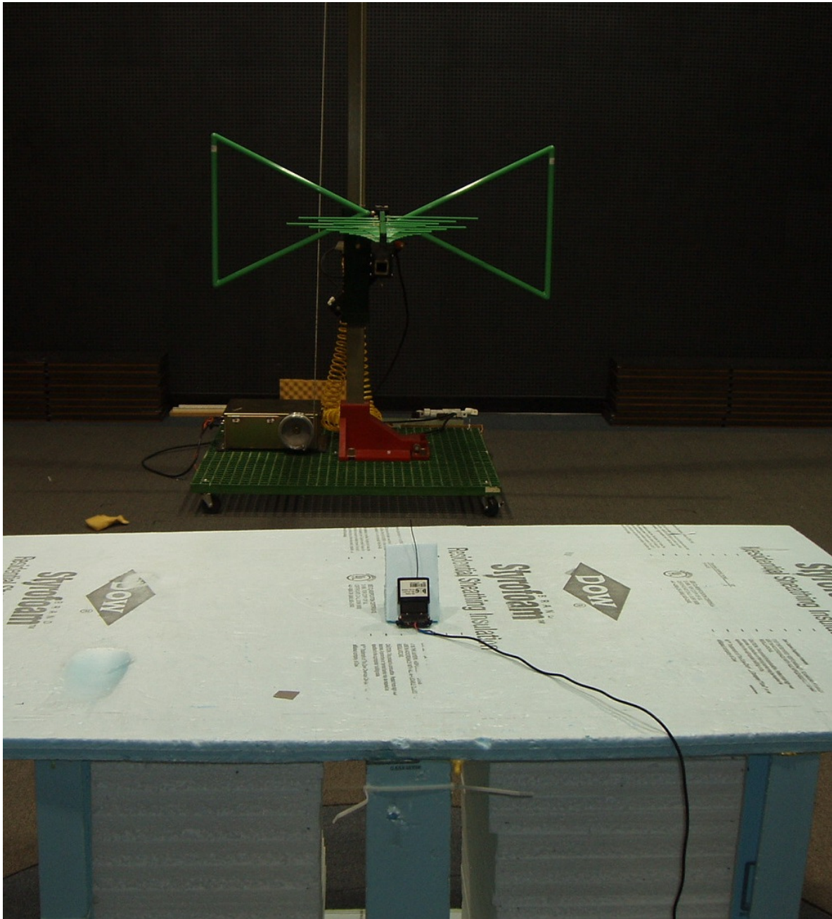
Photo 2 – Rear View of the Radiated Emissions Test Set-up 30 - 1000 MHz
