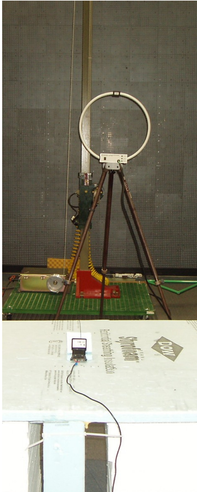
Photo 5 - Rear View of the Radiated Emissions Test Set-up 20 - 30 MHz
