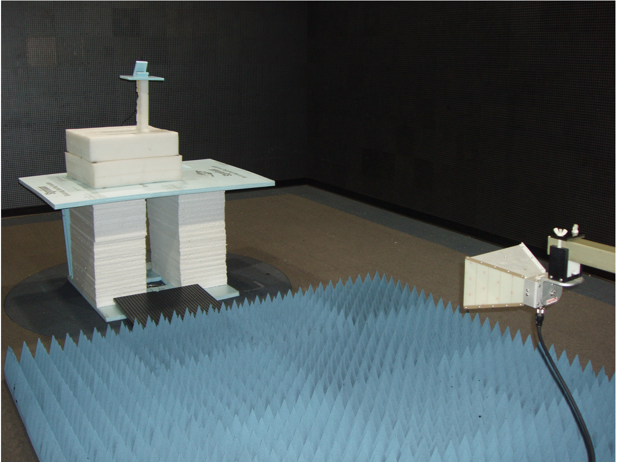
Photo 3 – Front View of the Radiated Emissions Test Set-up above 1 GHz
