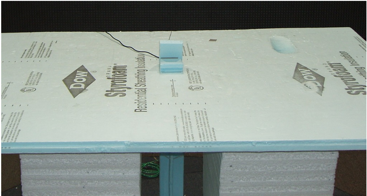
Photo 1 – Front View of the 30 – 1000 MHz Radiated Emissions Test Set-up
