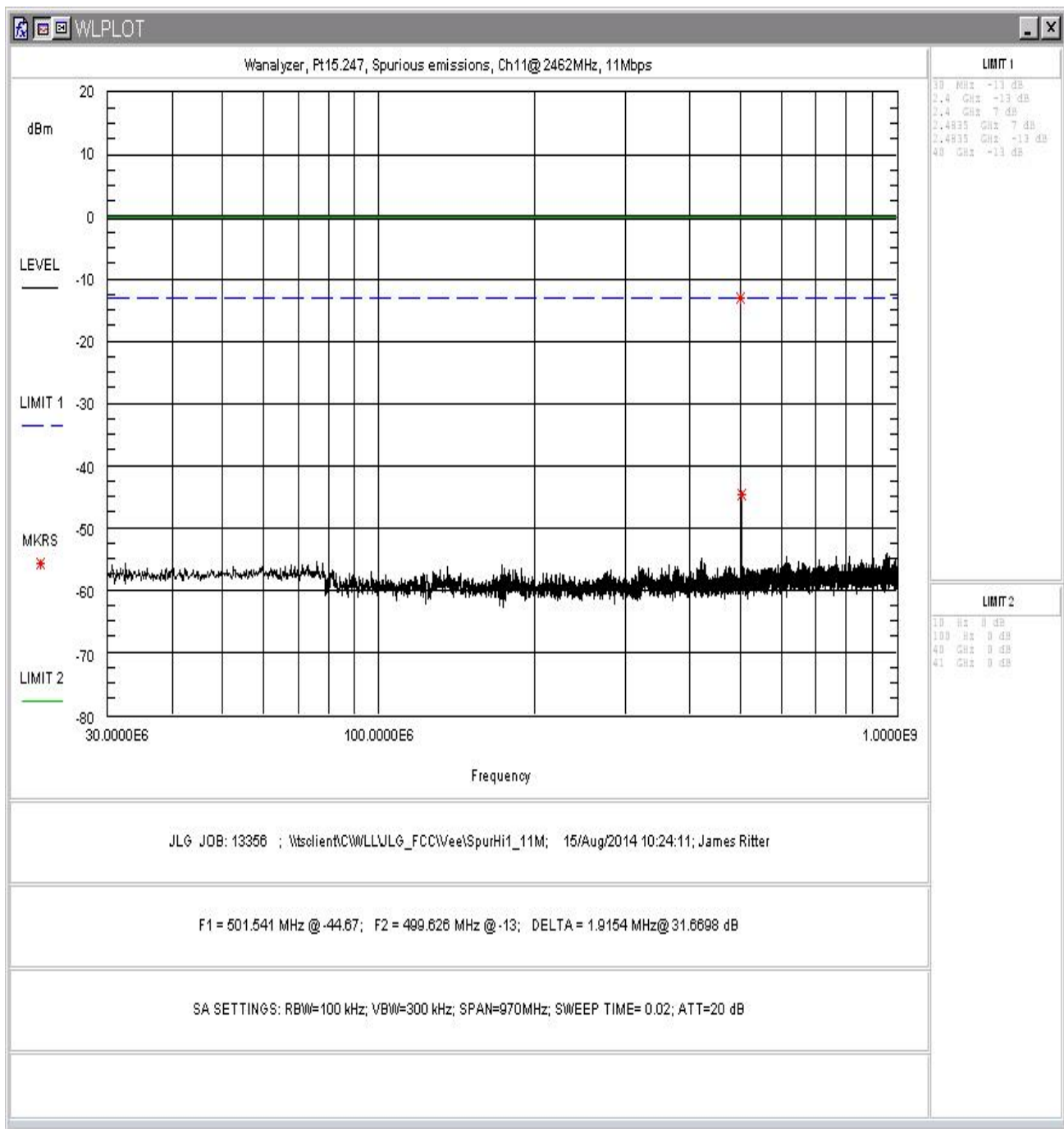
Figure 41: Conducted Spurious Emissions, Channel 11, 11Mbps, 30 - 1000MHz
