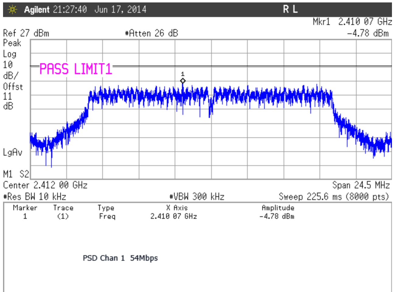
Figure 16: Power Spectral Density, 802.11g, 54Mbps, Channel 1
