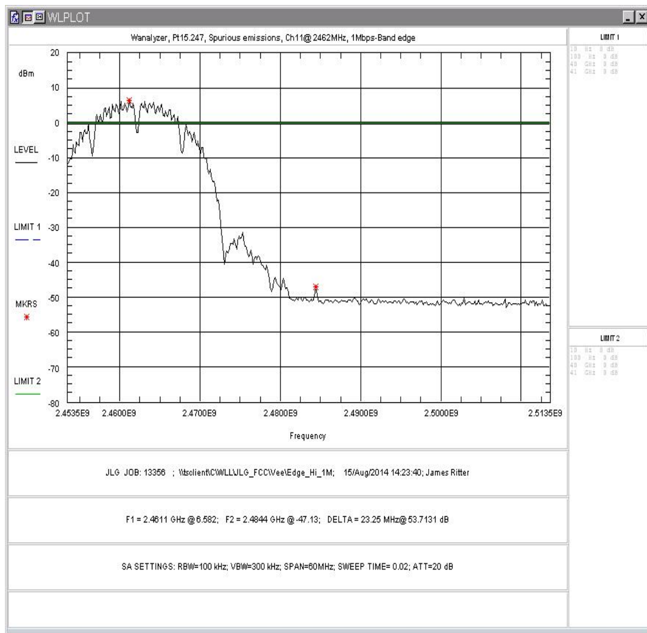
Figure 53: Upper Band-edge, Channel 11, 802.11b, 1Mbps
