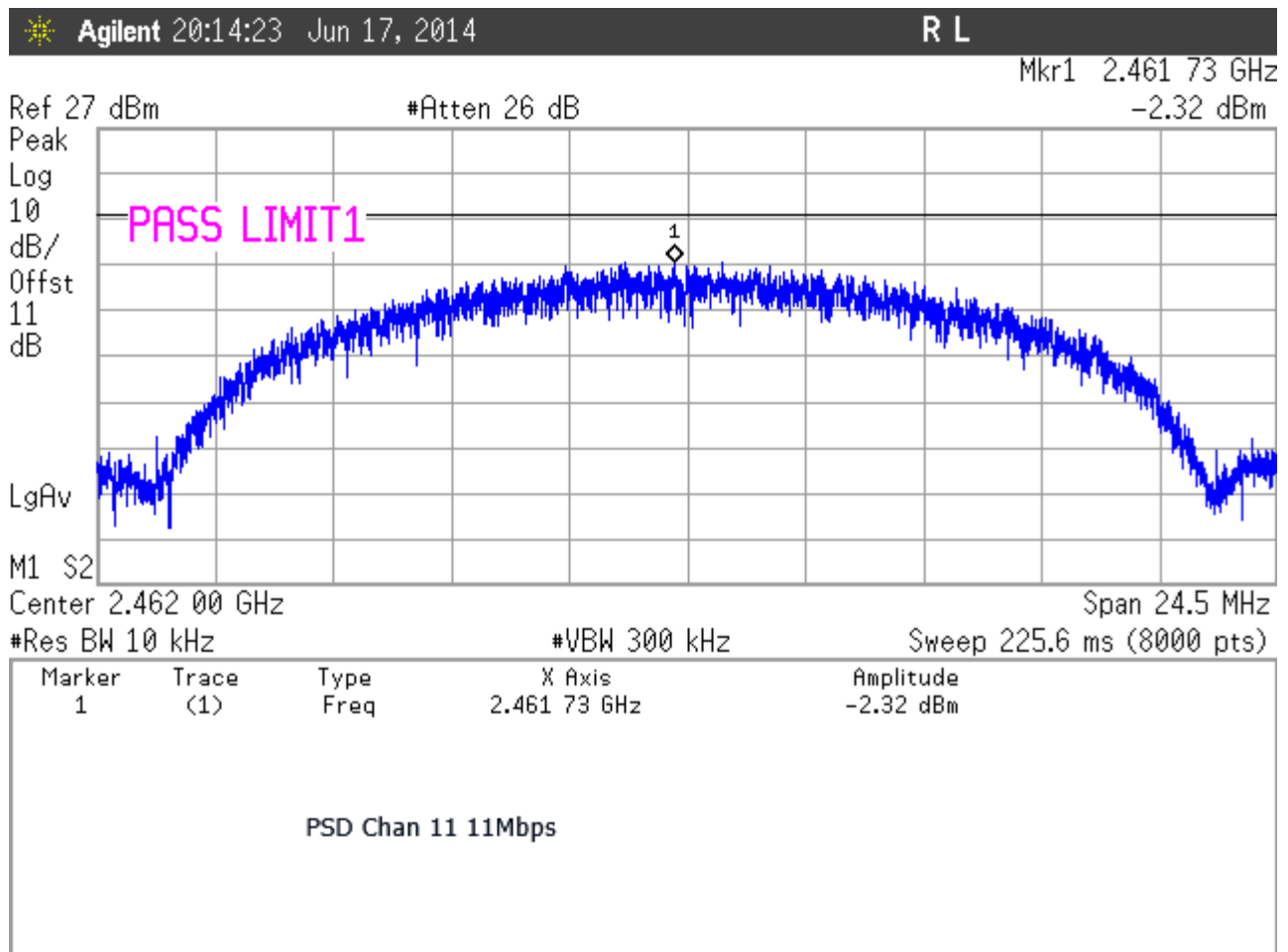
Figure 22: Power Spectral Density, 802.11b, 11Mbps, Channel 11
