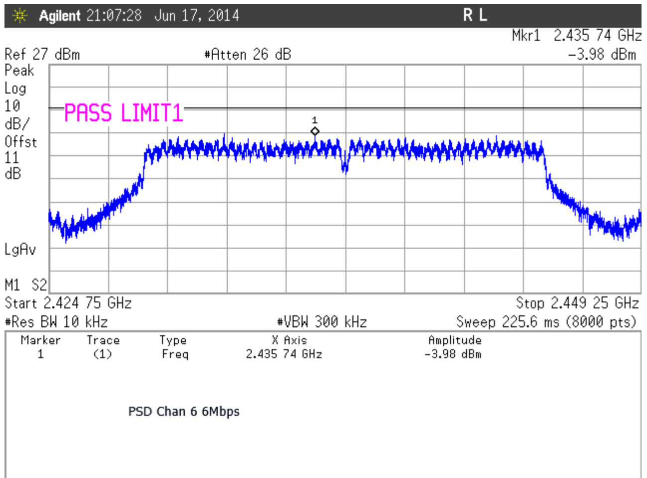
Figure 19: Power Spectral Density, 802.11g, 6Mbps, Channel 6
