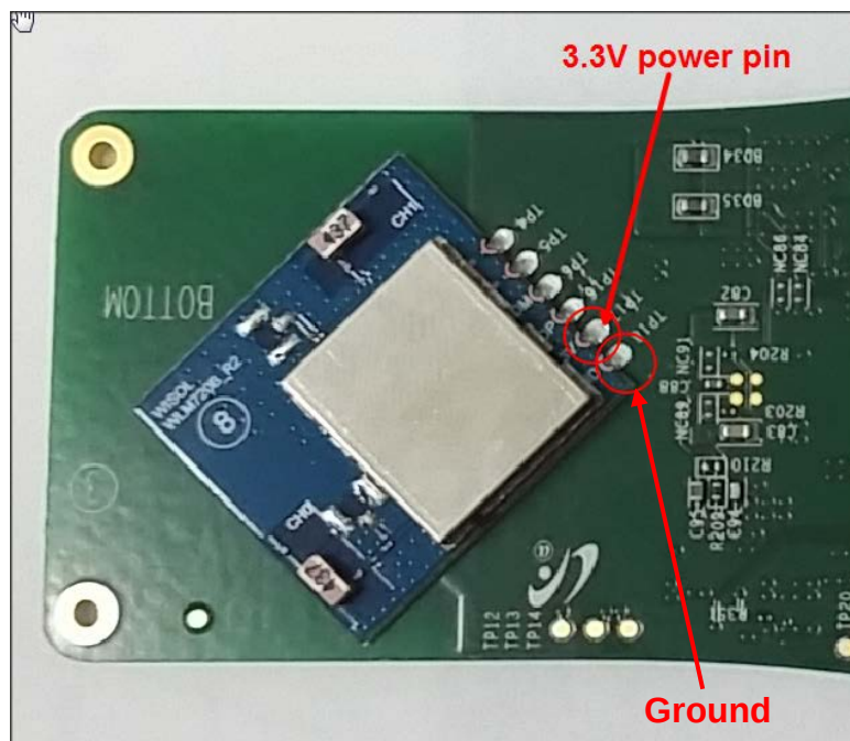
3.3V power for WLM720B is supplied from main PCB.
