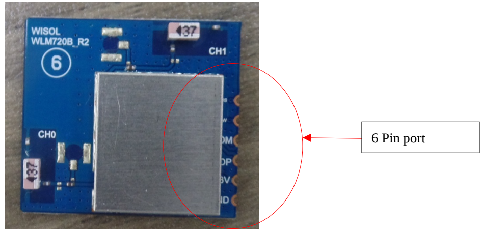
WLM720B wifi Module
