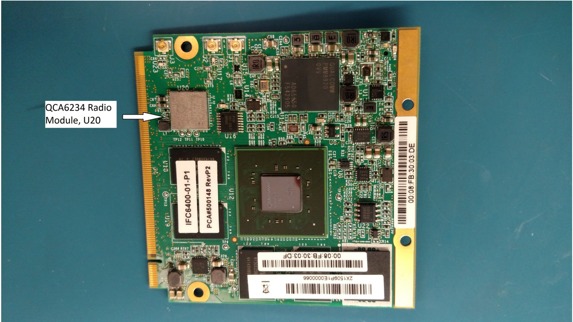
Top of P2077-03, InForce IFC6400-01-P3
