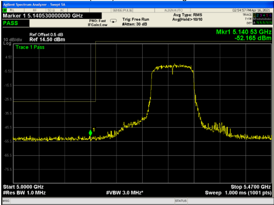
802.11ac (HT80) U-NII-2A Band edge-left side
