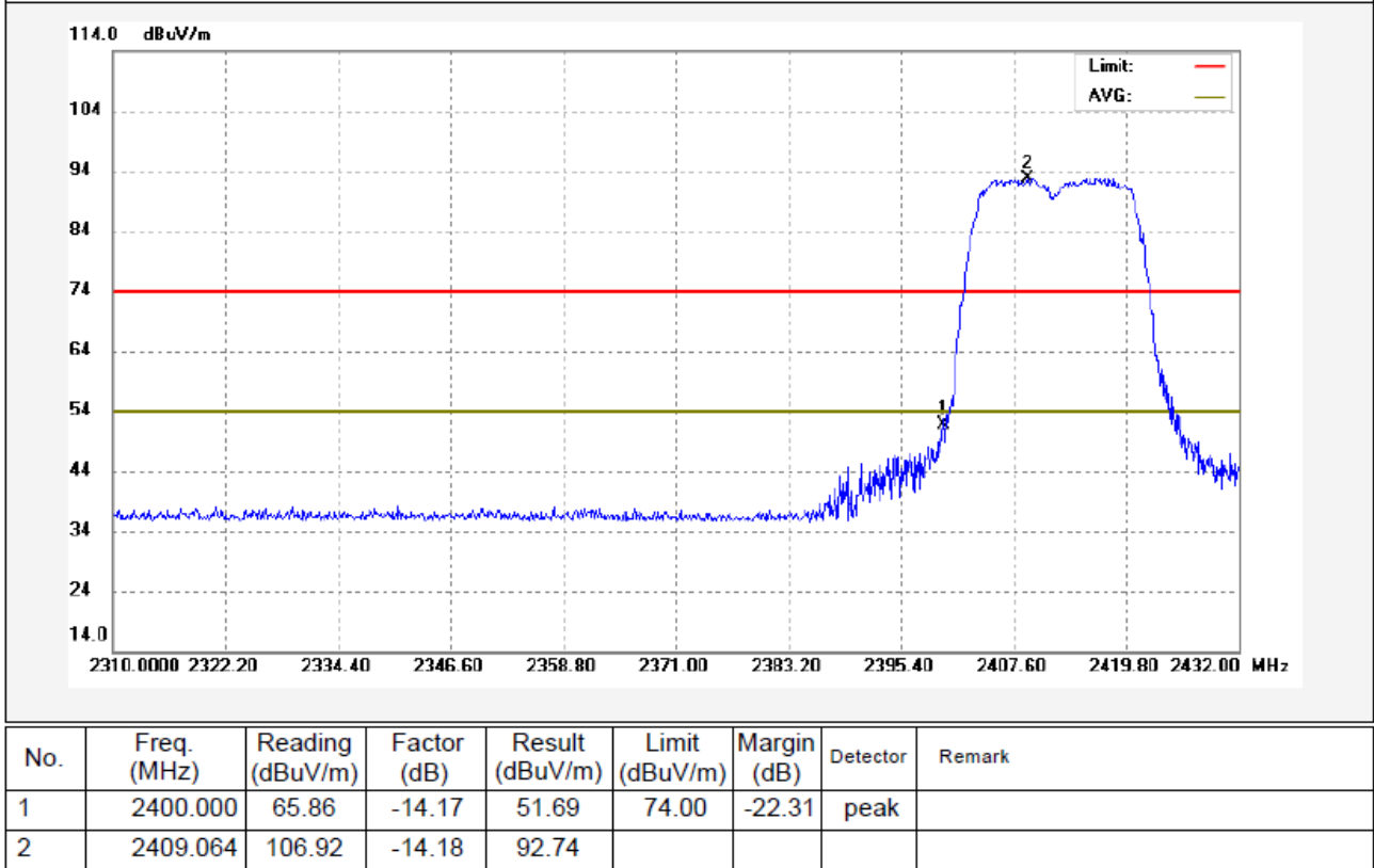
TX 11n HT20: Band edge-left side Vertical
