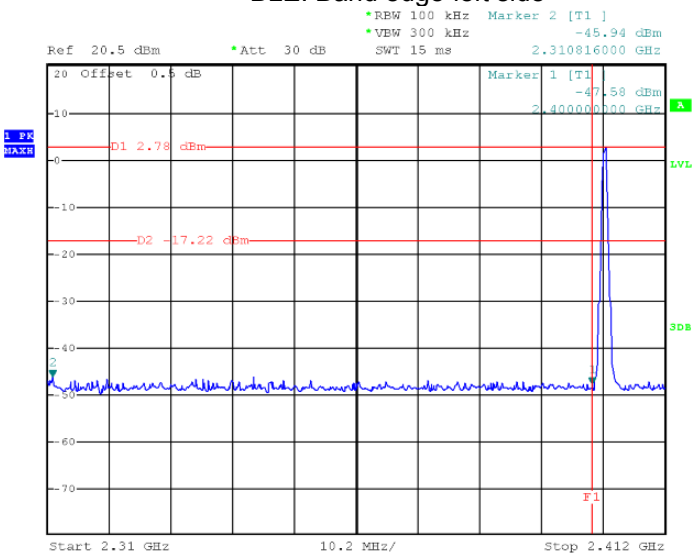
BLE: Band edge-left side
