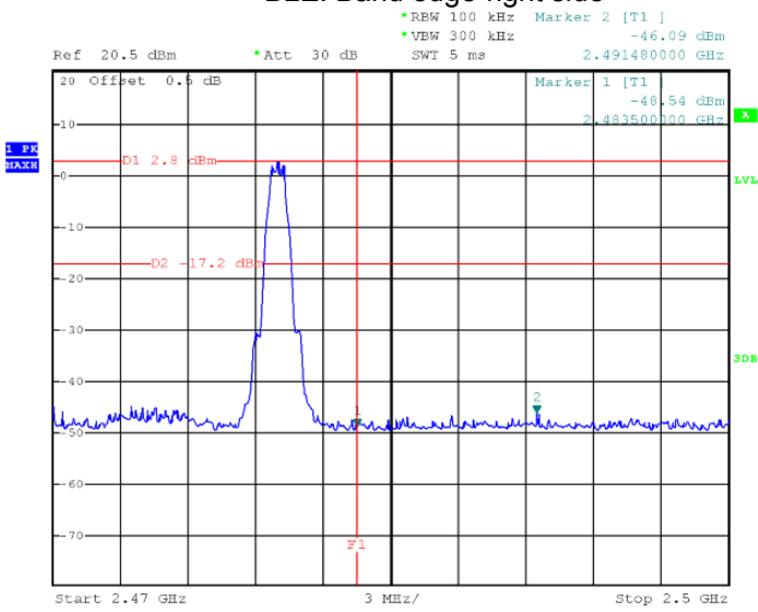
BLE: Band edge-right side
