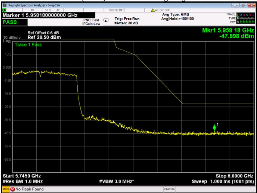
802.11ac(HT80) U-NII-3 Band edge- right side
