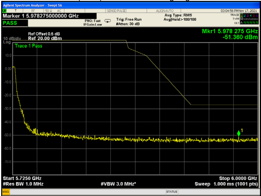
802.11a(HT20) U-NII-3 144 CH edge-right side
