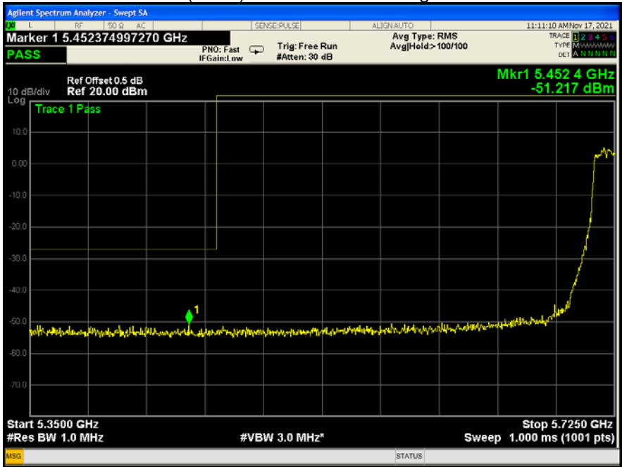
802.11a (HT20) U-NII-2C 144 CH edge-left side
