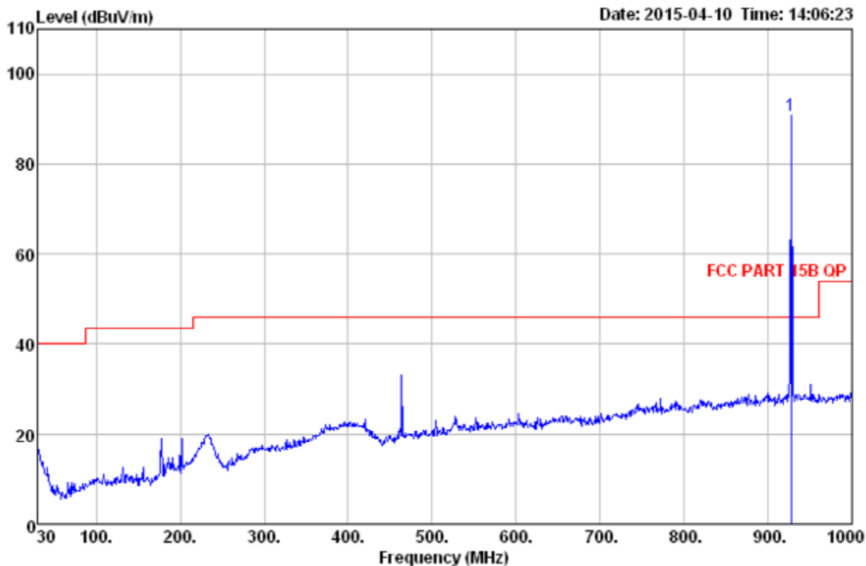
Quasi-peak measurement
