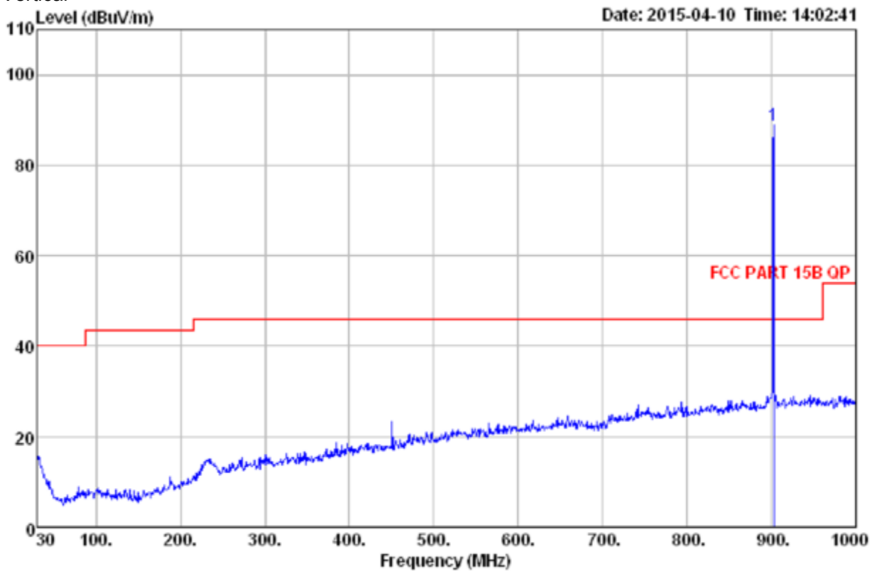
Quasi-peak measurement
