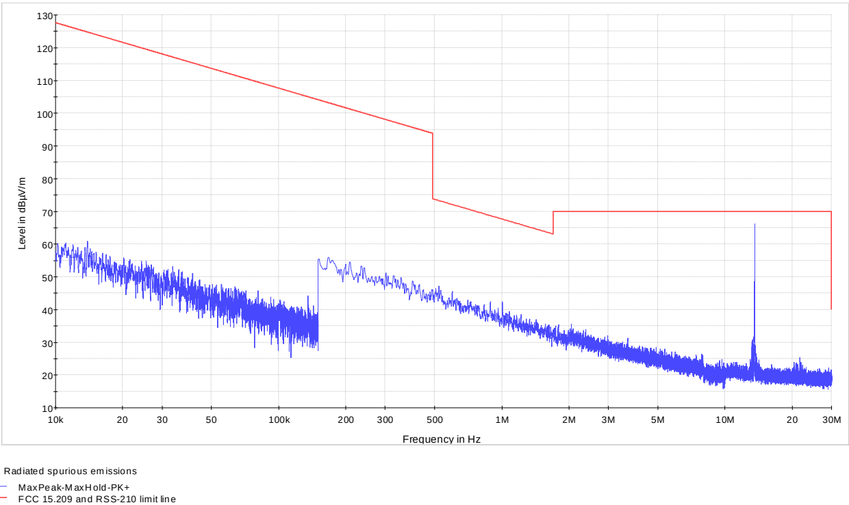
Figure 8.4-1: Field strength of spurious emissions – 10 kHz to 30 MHz
