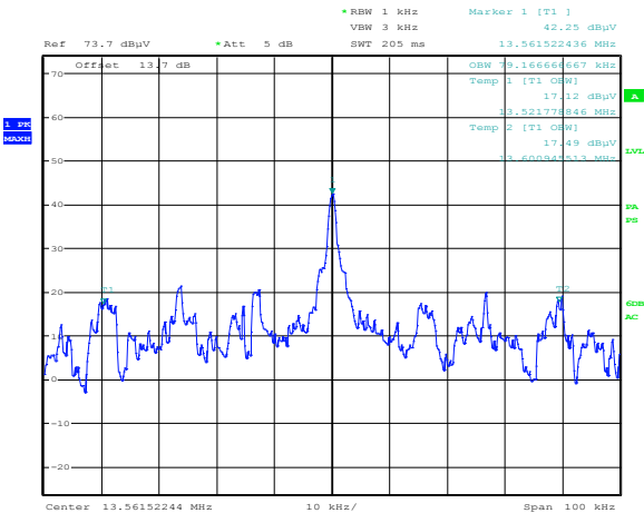
Figure 8.2-2: 99 % occupied bandwidth spectrum plot
