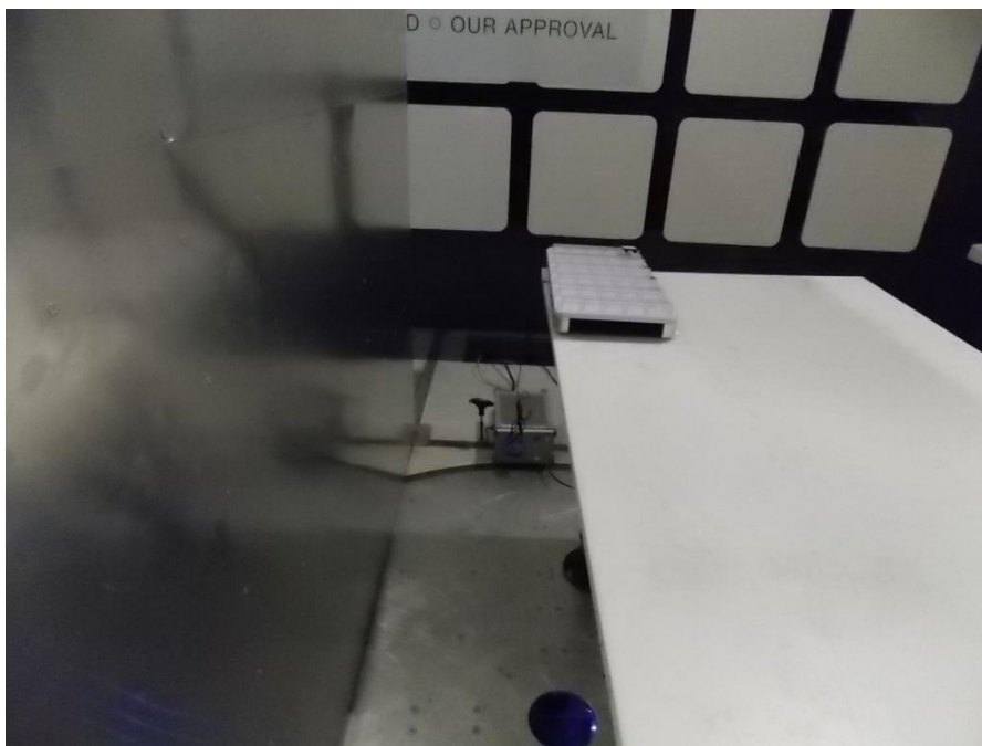
Figure 8.1-2: AC power line conducted emissions limits setup photo
