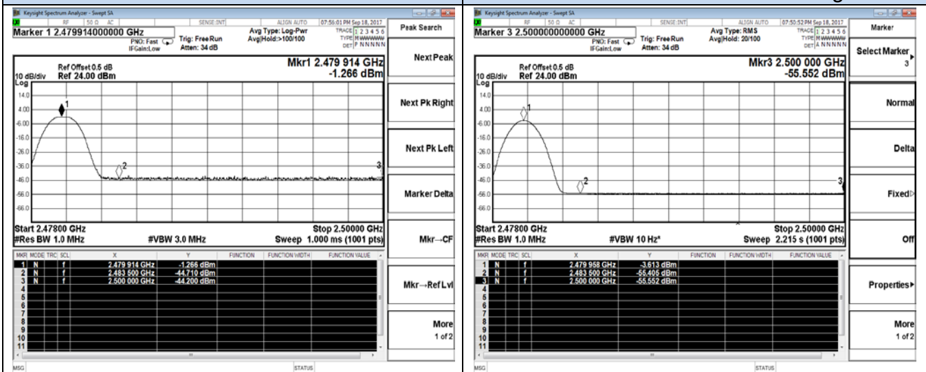
Channel 39 / 2480 MHz – Peak
