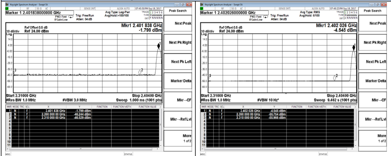
Channel 0 / 2402 MHz – Peak
