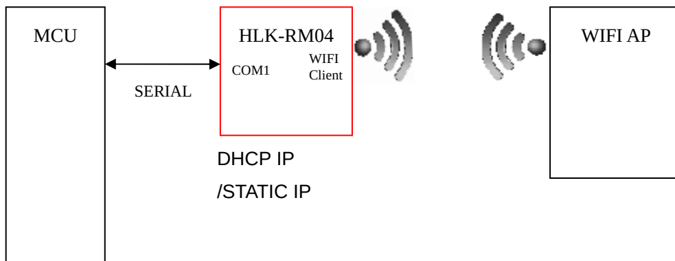
Fig6.2..Serial to WIFI CLIENT model
