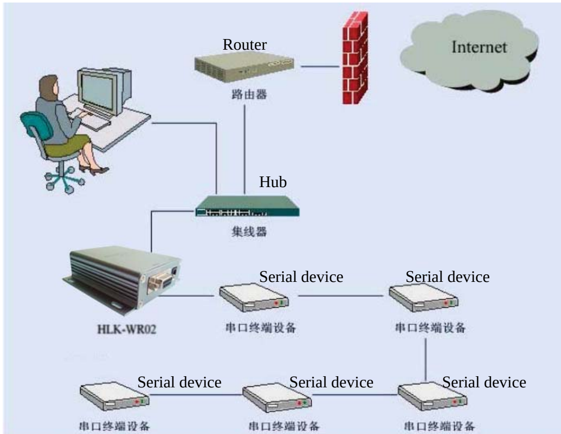
Fig 2-7 Bus Networking structure
