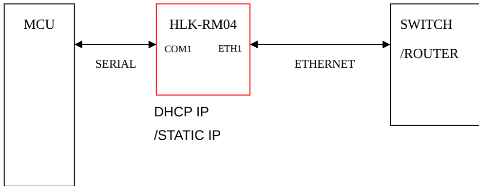
Fig6.1.serial to Ethernet model
