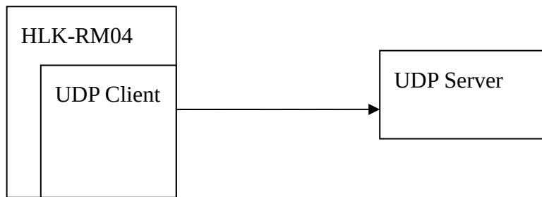
Fig6.4.4..UDP Client
