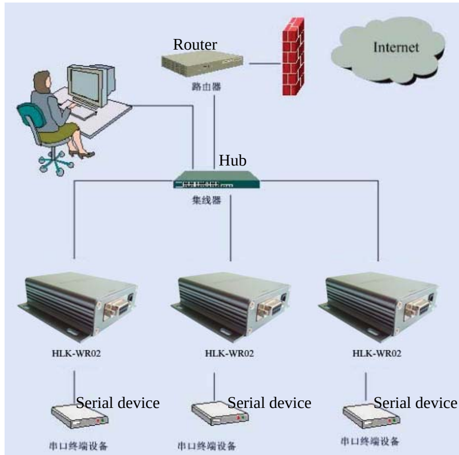
Fig 2-6 Starlike Networking
