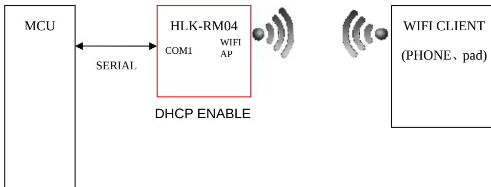
Fig6.3.. Serial to WIFI AP model
