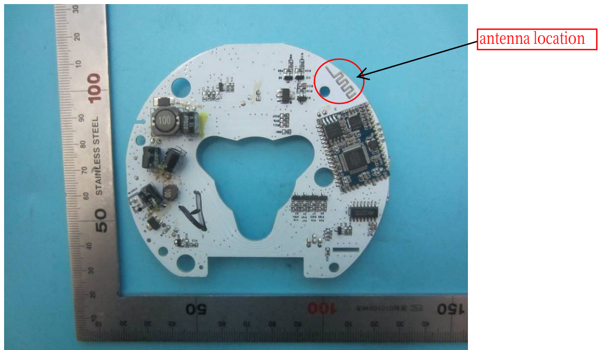
INTERNAL PHOTO OF SAMPLE – 3
