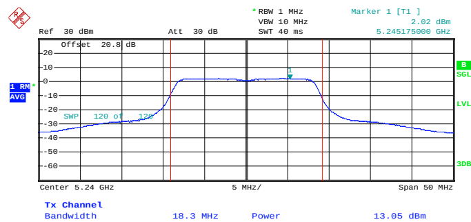
Figure 7.3.2-2: RF Output Power - Middle Channel – 802.11a
