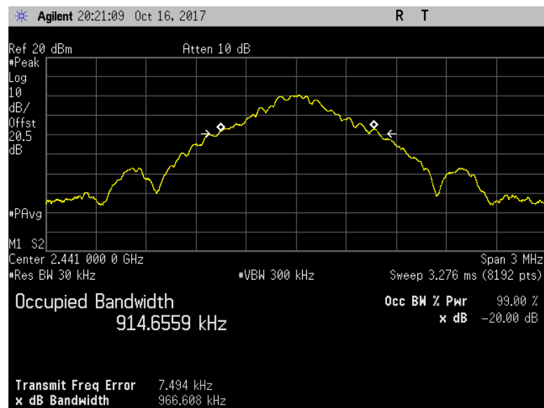
Figure 7.3.4.2-2: 20 dB / 99% BW – Middle Channel (GFSK)
