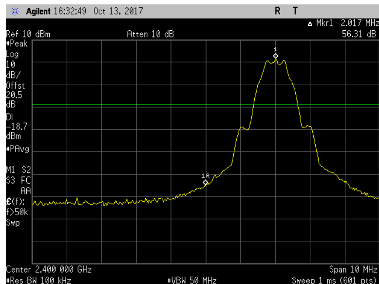
Figure 7.4.1.2-1: Lower Band-edge
