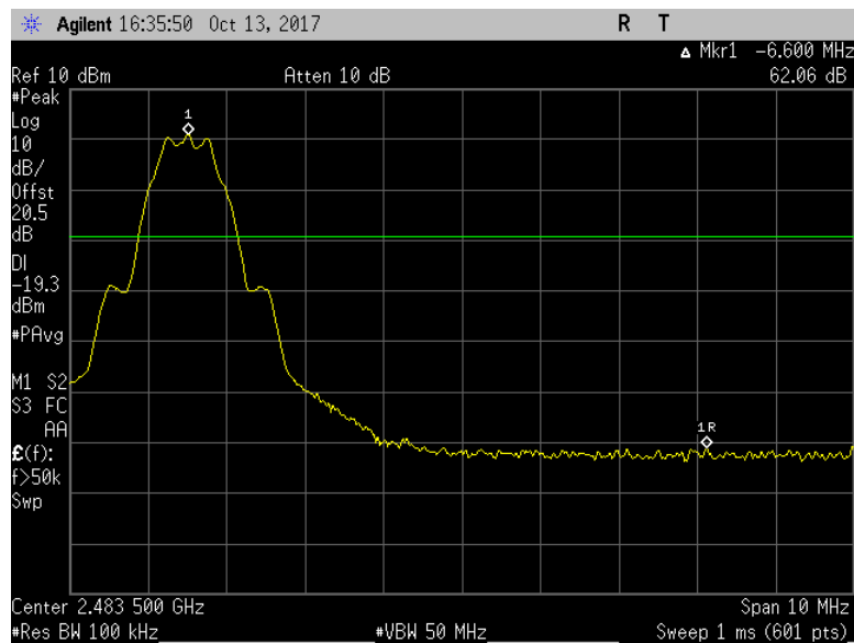
Figure 7.4.1.2-2: Upper Band-edge
