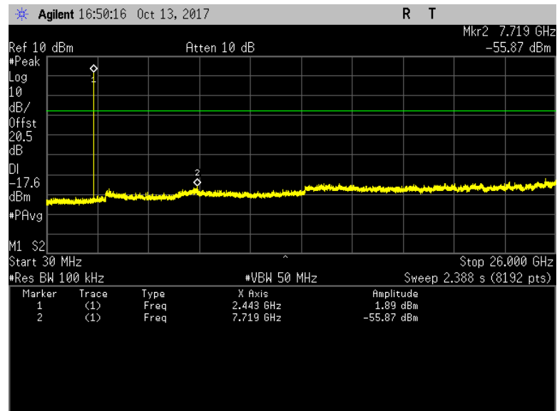
Figure 7.4.2.2-2: 30 MHz – 26 GHz – Middle Channel
