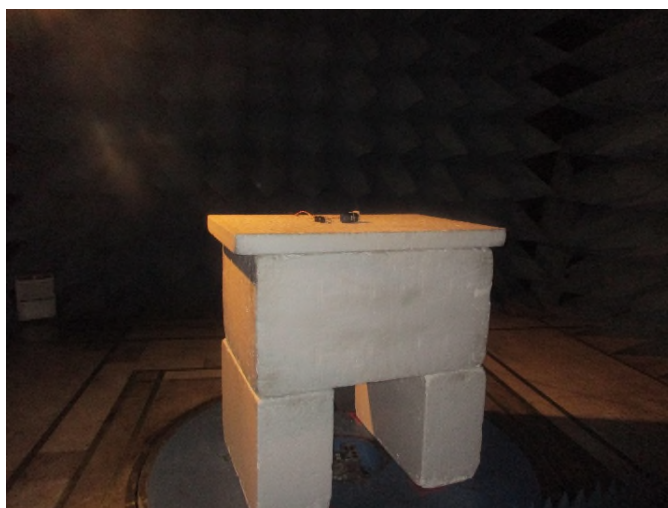
Figure 11: Radiated Emissions – above 1 GHz – Front View – EUT on Side
