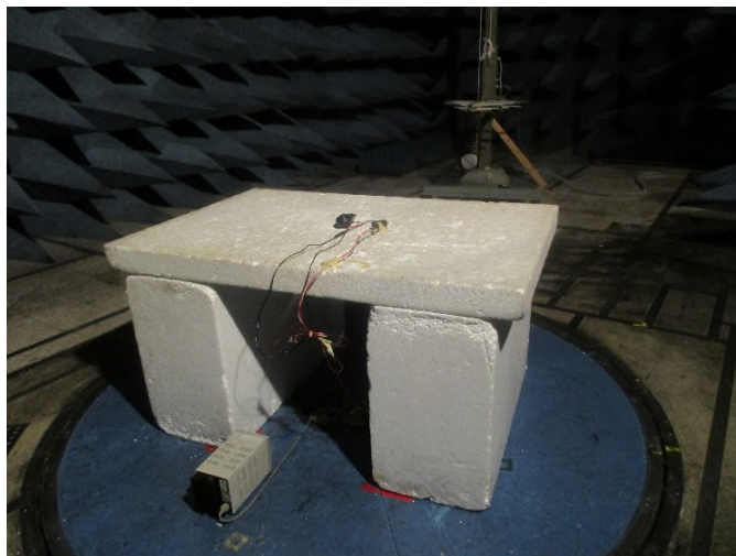
Figure 4: Radiated Emissions – 200 MHz – 1 GHz – Rear View – EUT Flat
