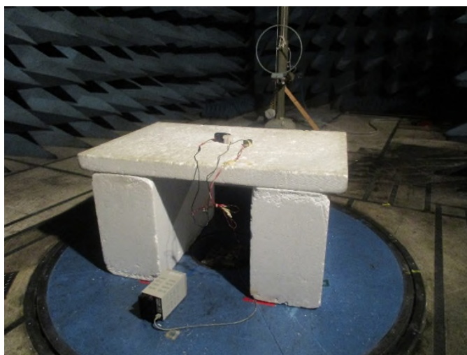
Figure 8: Radiated Emissions – 9 kHz – 30 MHz – Rear View – EUT on Side
