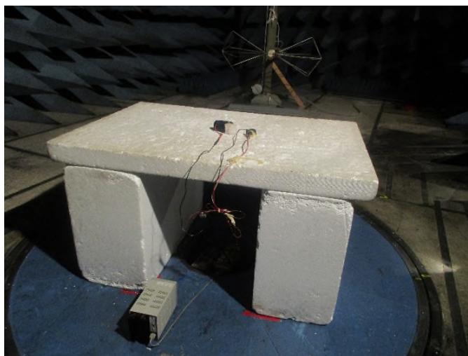
Figure 9: Radiated Emissions – 30 MHz – 200 MHz – Rear View – EUT on Side
