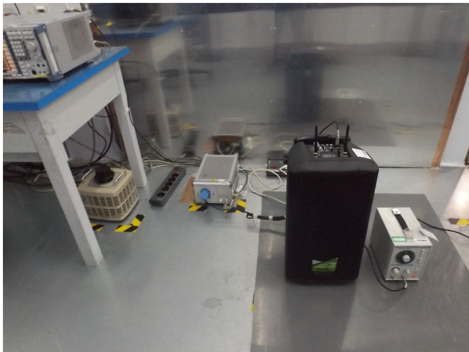
Photograph 4: Set-up for Conducted Emission on AC Mains
