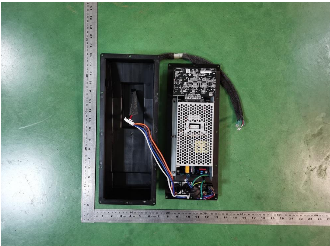
Picture 2. main board with fire enclosure cover
