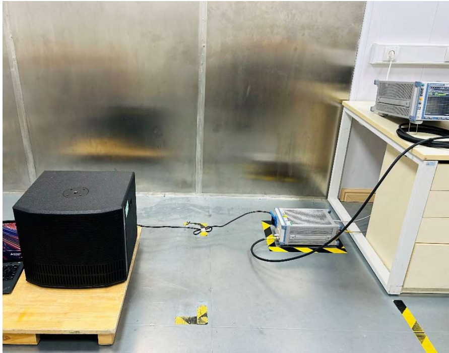
Photograph 3: Set-up for Conducted Emission on AC Mains
