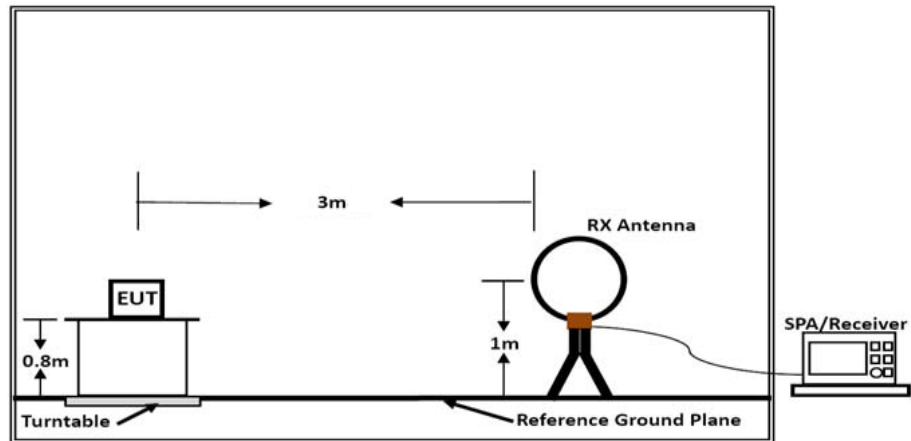
Below 30MHz
