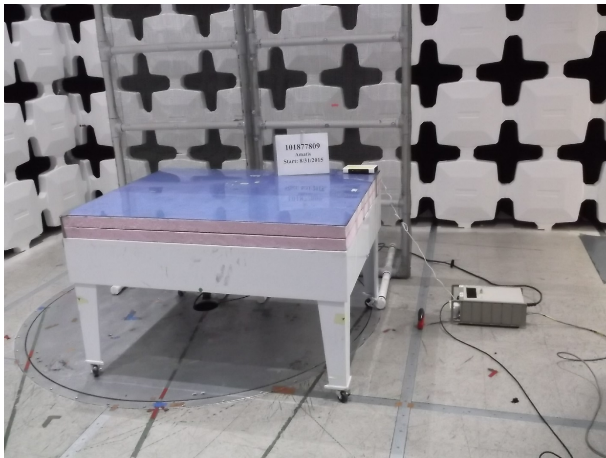
Test Setup – Conducted Emissions (Front View)
