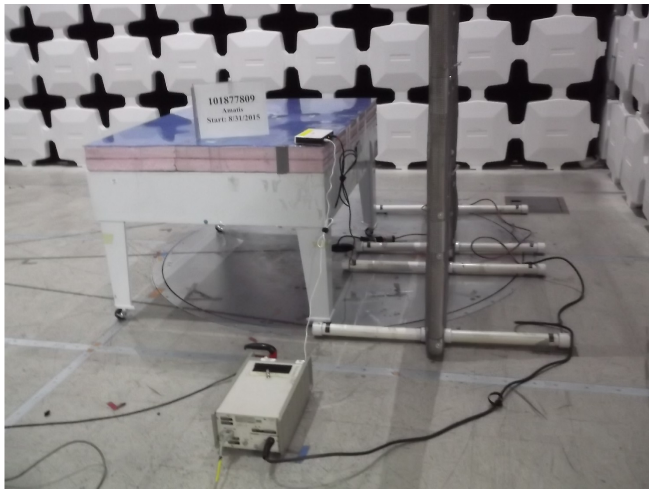
Test Setup – Conducted Emissions (Side View)
