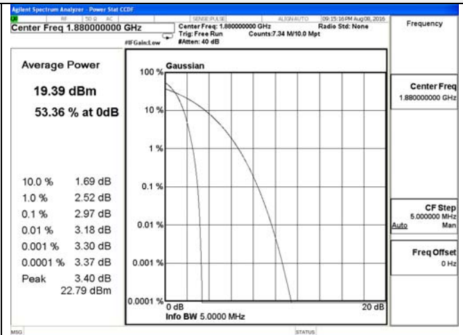
Channel 9400 / 1880.0 MHz
