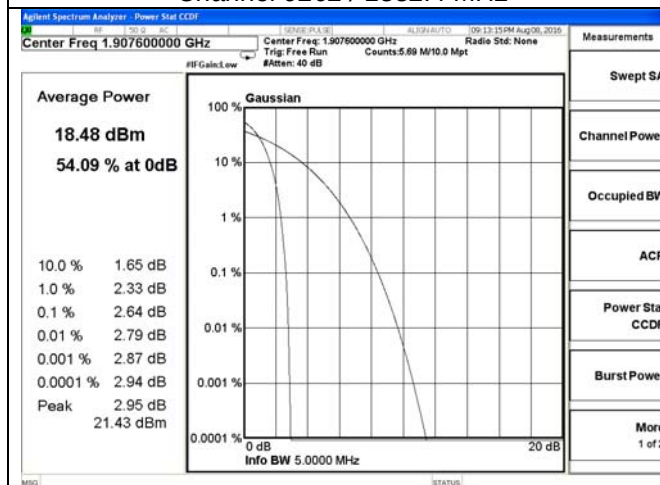
Channel 9538 / 1907.6 MHz
