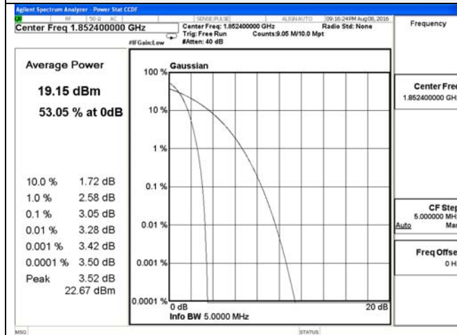
Channel 9262 / 1852.4 MHz
