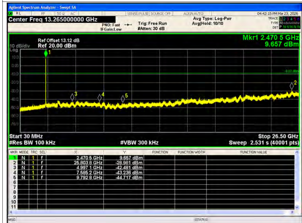
Tx. Spurious NVNT ax20 106@53 2472MHz Ant2 Emission
