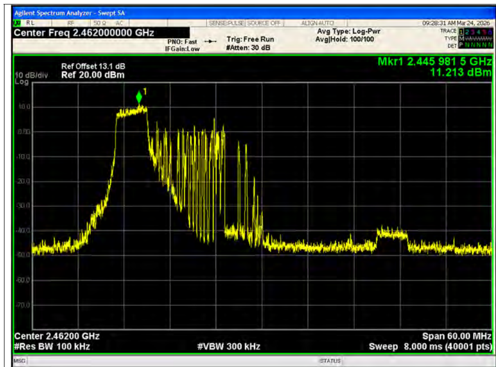
Tx. Spurious NVNT ax40 52@37 2462MHz Ant1 Ref
