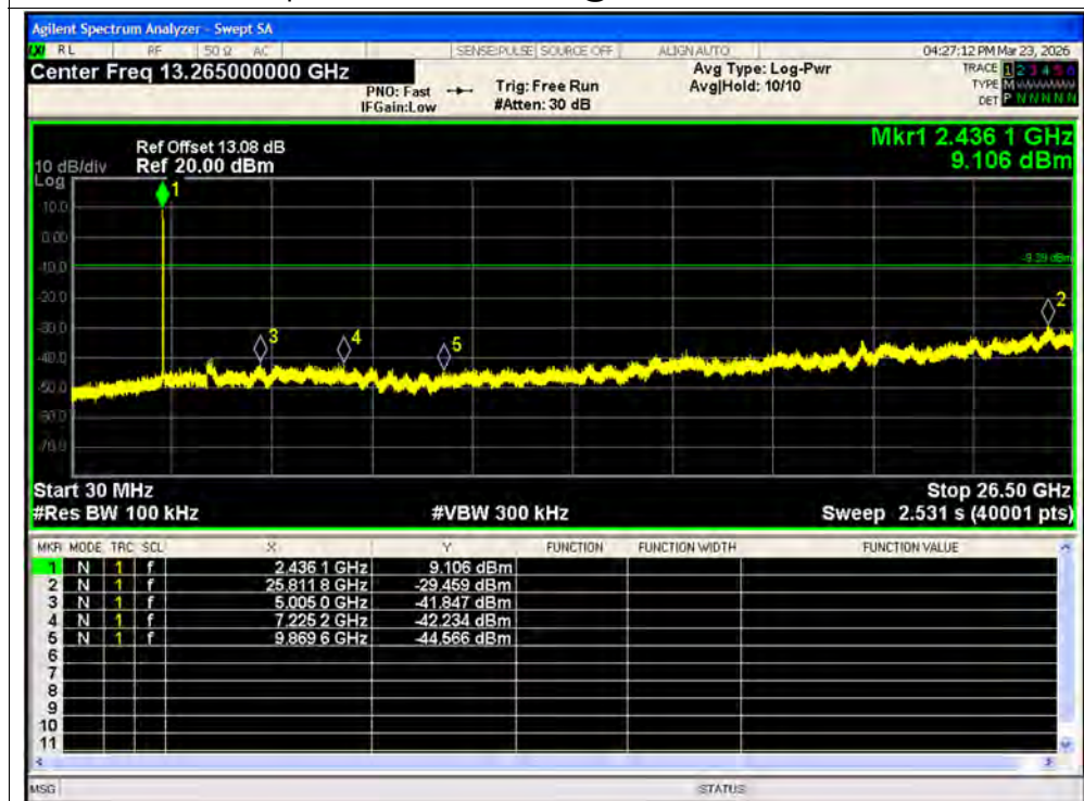
Tx. Spurious NVNT ax20 52@37 2442MHz Ant2 Emission
