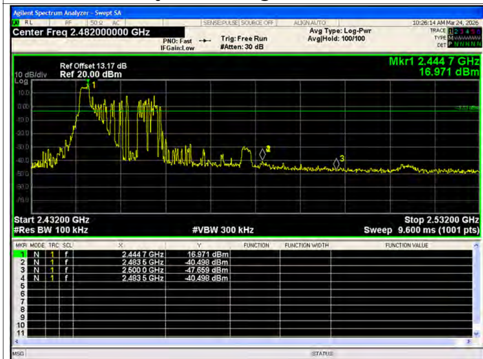
Band Edge NVNT ax40 26@0 2462MHz Ant2 Emission
