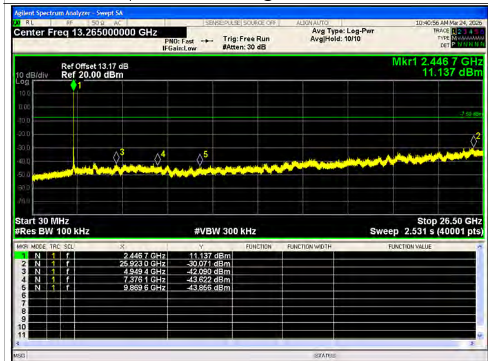
Tx. Spurious NVNT ax40 52@37 2462MHz Ant2 Emission
