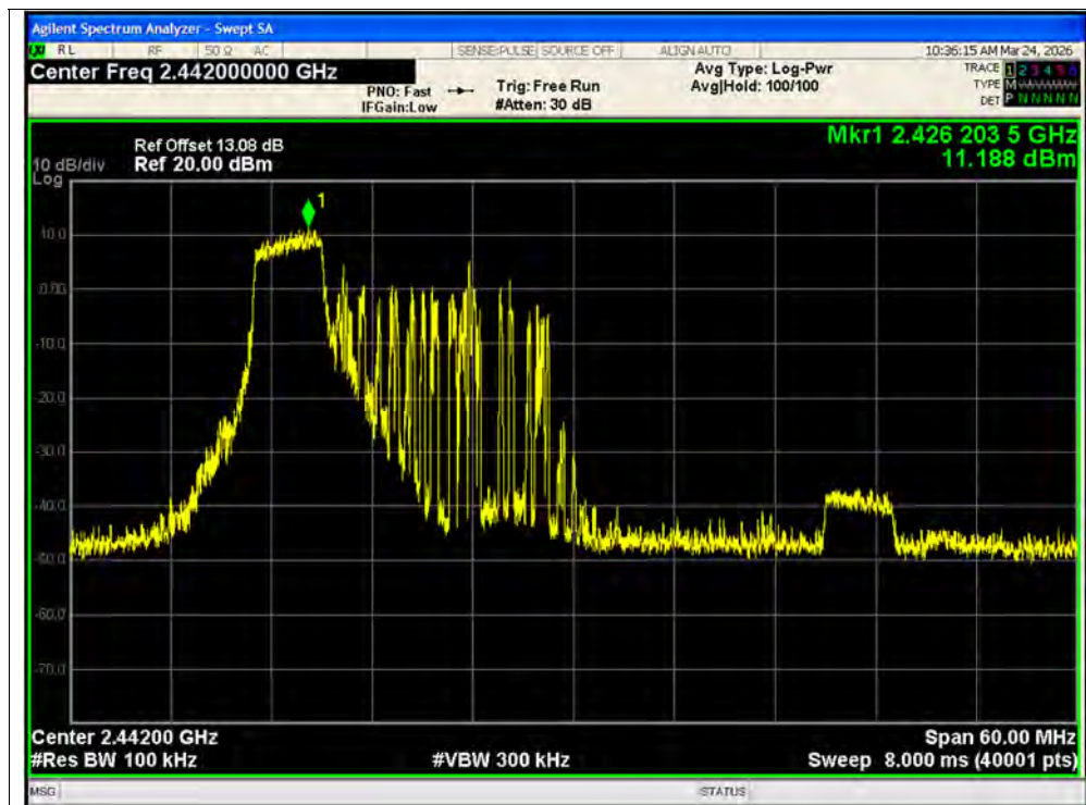
Tx. Spurious NVNT ax40 52@37 2442MHz Ant2 Ref
