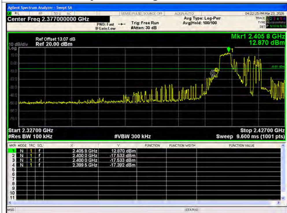
Band Edge NVNT ax20 52@37 2412MHz Ant2 Emission
