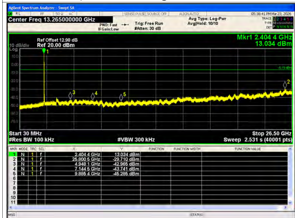
Tx. Spurious NVNT ax40 26@0 2422MHz Ant1 Emission
