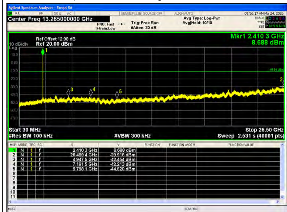
Tx. Spurious NVNT ax40 106@53 2422MHz Ant1 Emission
