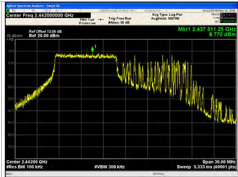
Tx. Spurious NVNT ax20 106@53 2442MHz Ant2 Ref
