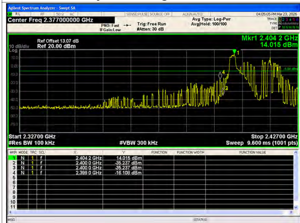
Band Edge NVNT ax20 26@0 2412MHz Ant2 Emission
