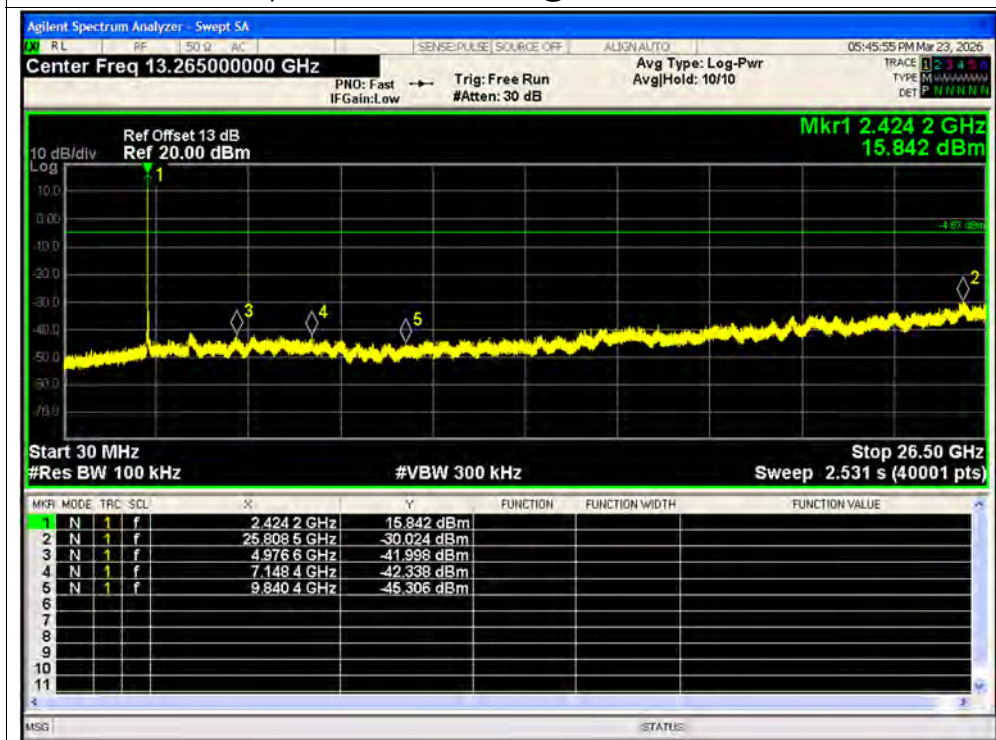
Tx. Spurious NVNT ax40 26@0 2442MHz Ant1 Emission
