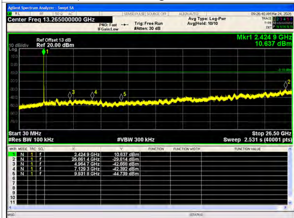
Tx. Spurious NVNT ax40 52@37 2442MHz Ant1 Emission
