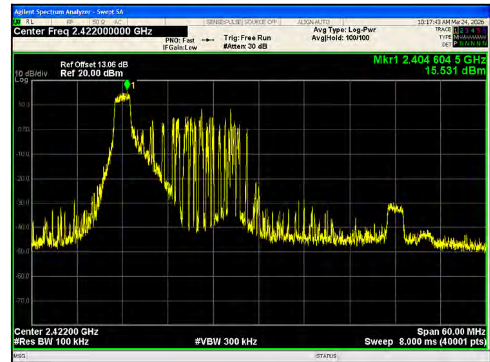
Tx. Spurious NVNT ax40 26@0 2422MHz Ant2 Ref
