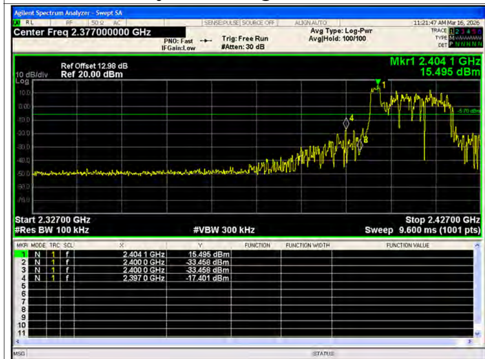
Band Edge NVNT ax20 26@0 2412MHz Ant1 Emission
