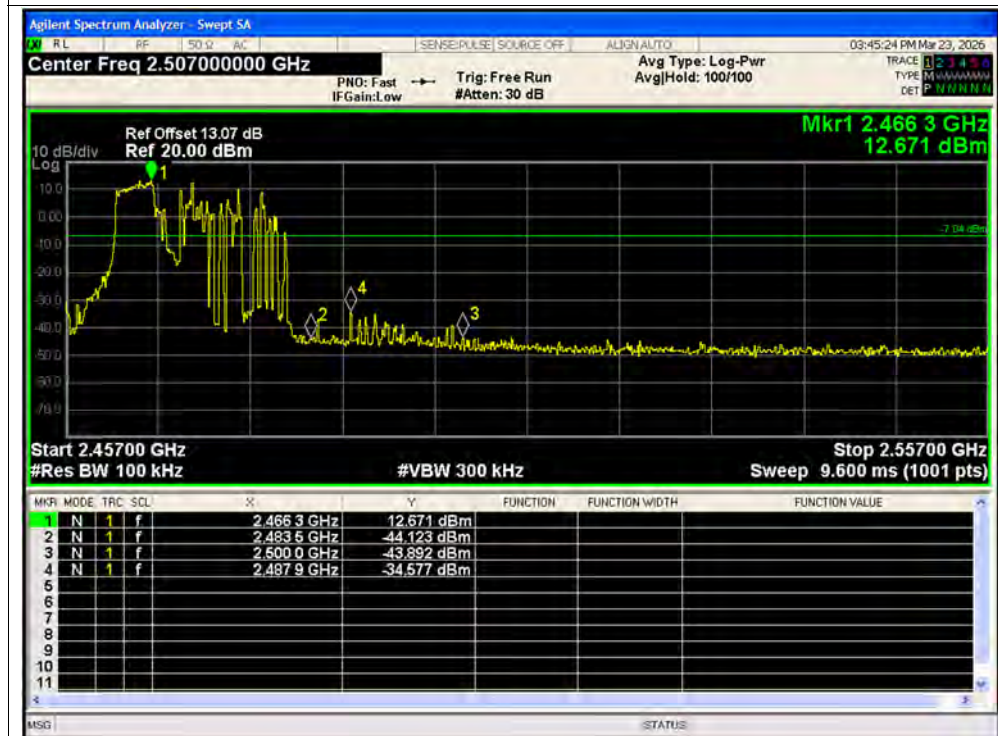
Band Edge NVNT ax20 52@37 2472MHz Ant1 Emission
