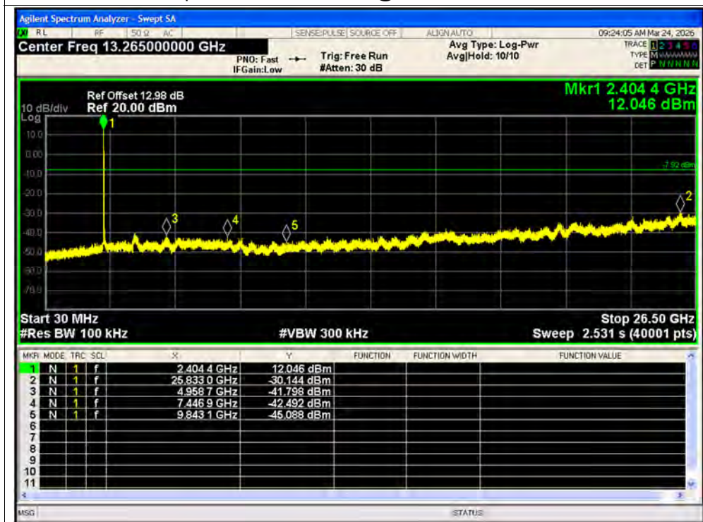
Tx. Spurious NVNT ax40 52@37 2422MHz Ant1 Emission
