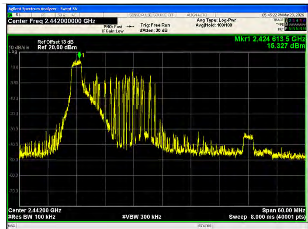
Tx. Spurious NVNT ax40 26@0 2442MHz Ant1 Ref
