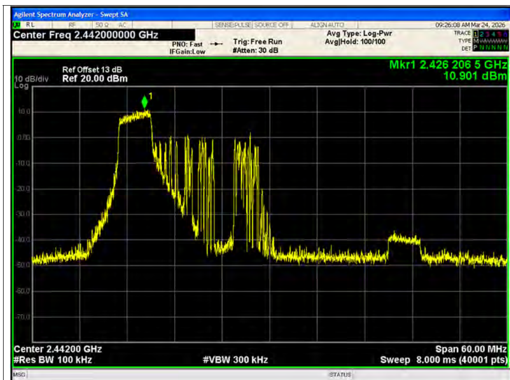
Tx. Spurious NVNT ax40 52@37 2442MHz Ant1 Ref
