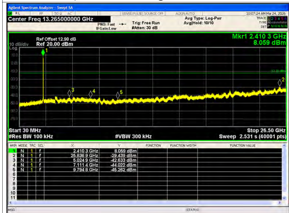
Tx. Spurious NVNT ax40 242@61 2422MHz Ant1 Emission
