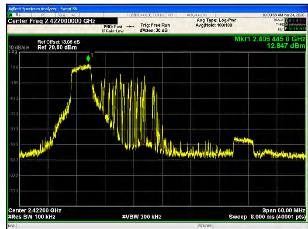
Tx. Spurious NVNT ax40 52@37 2422MHz Ant2 Ref
