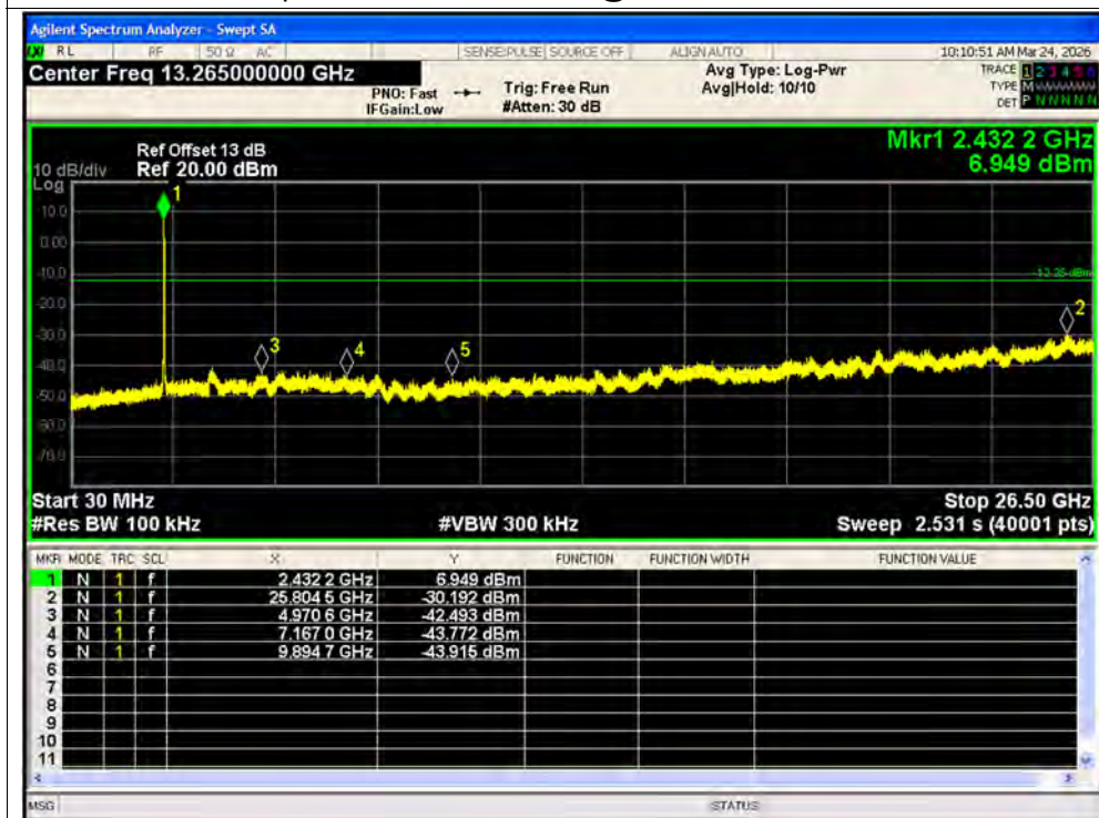
Tx. Spurious NVNT ax40 242@61 2442MHz Ant1 Emission
