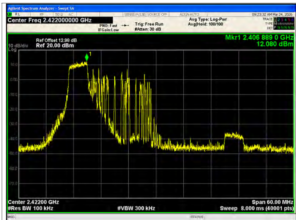
Tx. Spurious NVNT ax40 52@37 2422MHz Ant1 Ref
