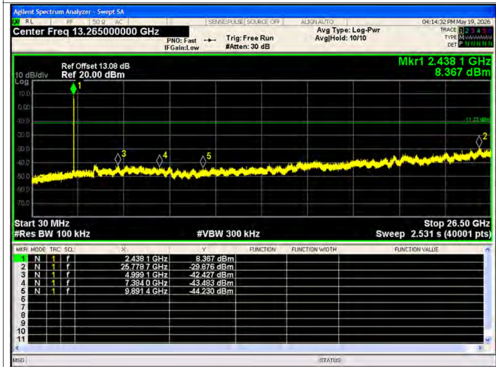
Tx. Spurious NVNT ax20 106@53 2442MHz Ant2 Emission
