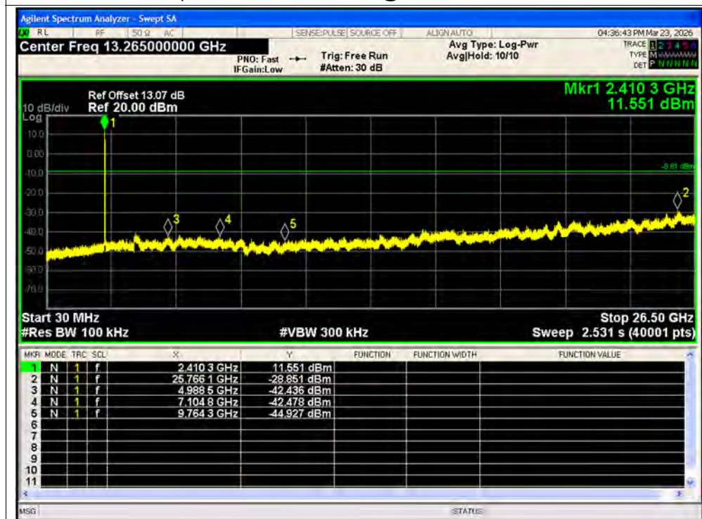
Tx. Spurious NVNT ax20 106@53 2412MHz Ant2 Emission
