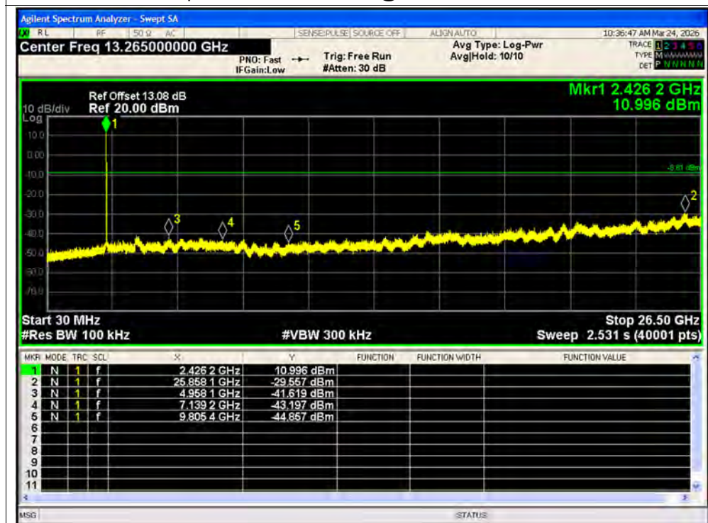
Tx. Spurious NVNT ax40 52@37 2442MHz Ant2 Emission
