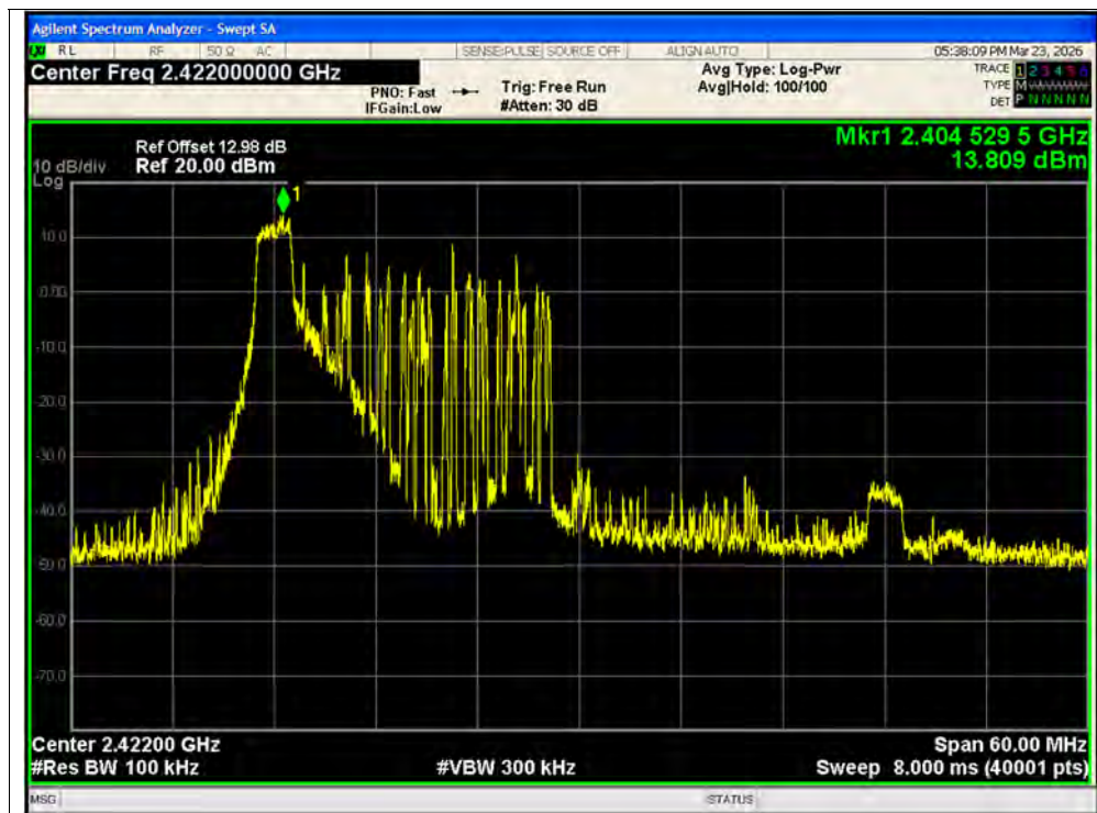
Tx. Spurious NVNT ax40 26@0 2422MHz Ant1 Ref
