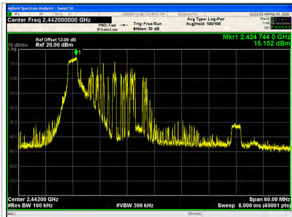
Tx. Spurious NVNT ax40 26@0 2442MHz Ant2 Ref
