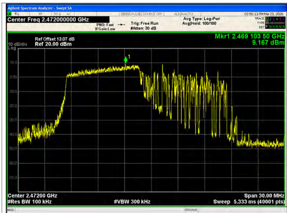
Tx. Spurious NVNT ax20 106@53 2472MHz Ant1 Ref
