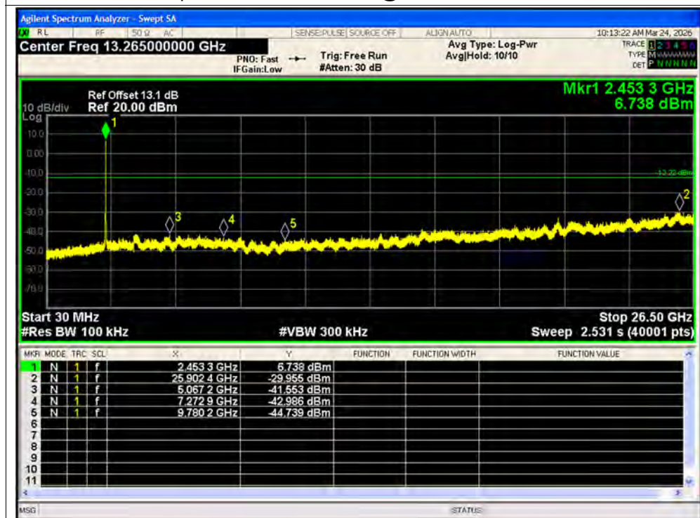
Tx. Spurious NVNT ax40 242@61 2462MHz Ant1 Emission
