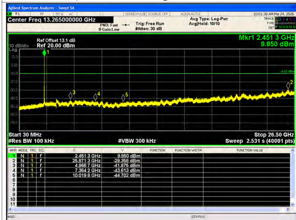
Tx. Spurious NVNT ax40 106@53 2462MHz Ant1 Emission
