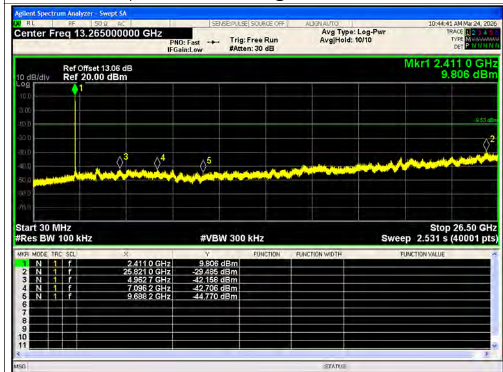
Tx. Spurious NVNT ax40 106@53 2422MHz Ant2 Emission
