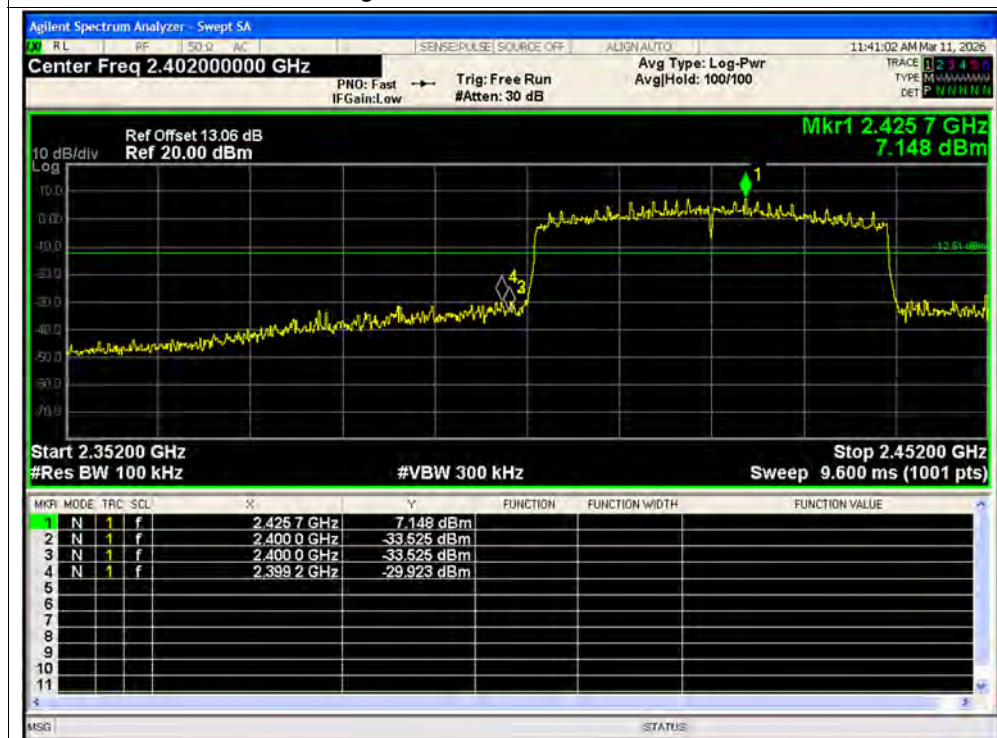
Band Edge NVNT ax40 2422MHz Ant2 Emission
