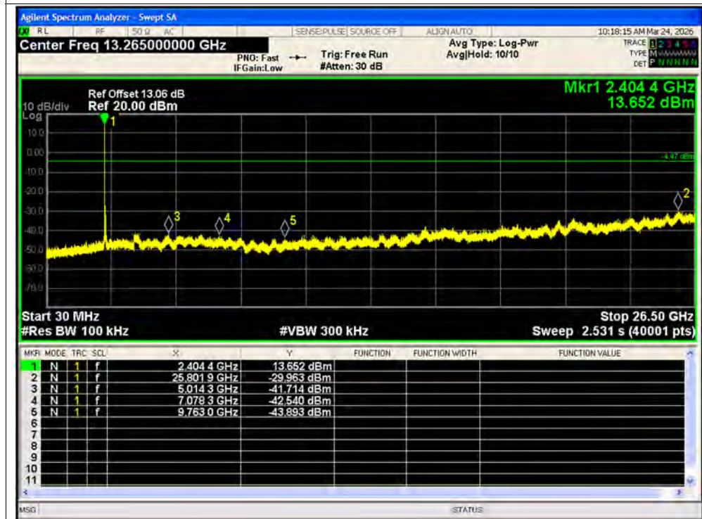
Tx. Spurious NVNT ax40 26@0 2422MHz Ant2 Emission
