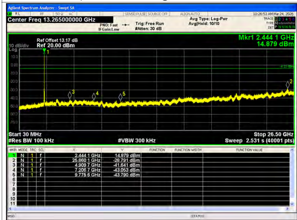
Tx. Spurious NVNT ax40 26@0 2462MHz Ant2 Emission
