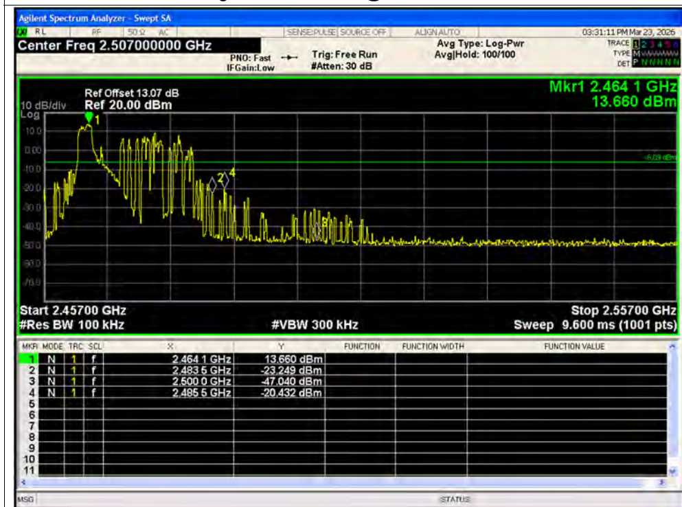
Band Edge NVNT ax20 26@0 2472MHz Ant1 Emission
