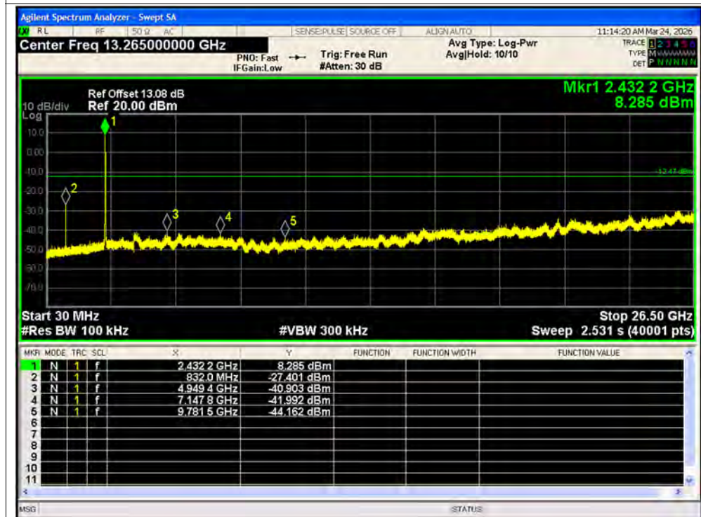
Tx. Spurious NVNT ax40 242@61 2442MHz Ant2 Emission
