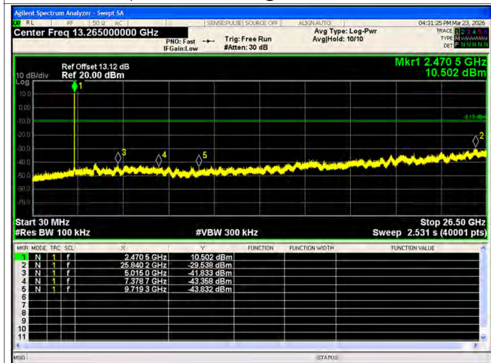
Tx. Spurious NVNT ax20 52@37 2472MHz Ant2 Emission
