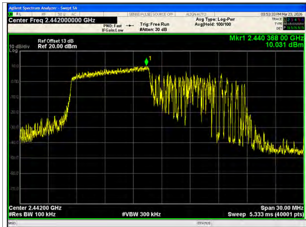
Tx. Spurious NVNT ax20 106@53 2442MHz Ant1 Ref
