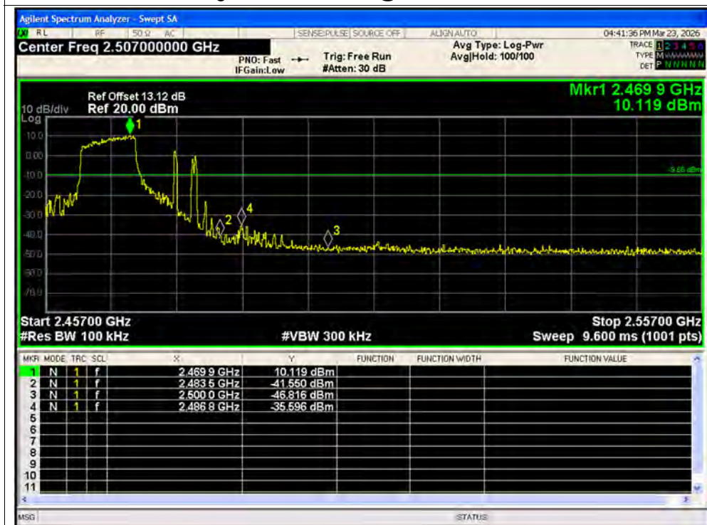
Band Edge NVNT ax20 106@53 2472MHz Ant2 Emission
