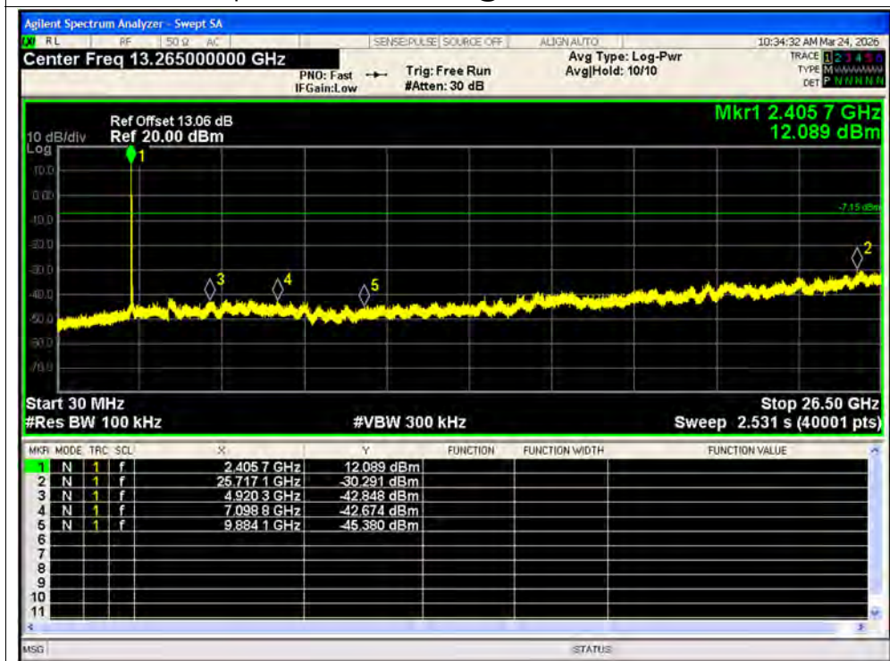
Tx. Spurious NVNT ax40 52@37 2422MHz Ant2 Emission
