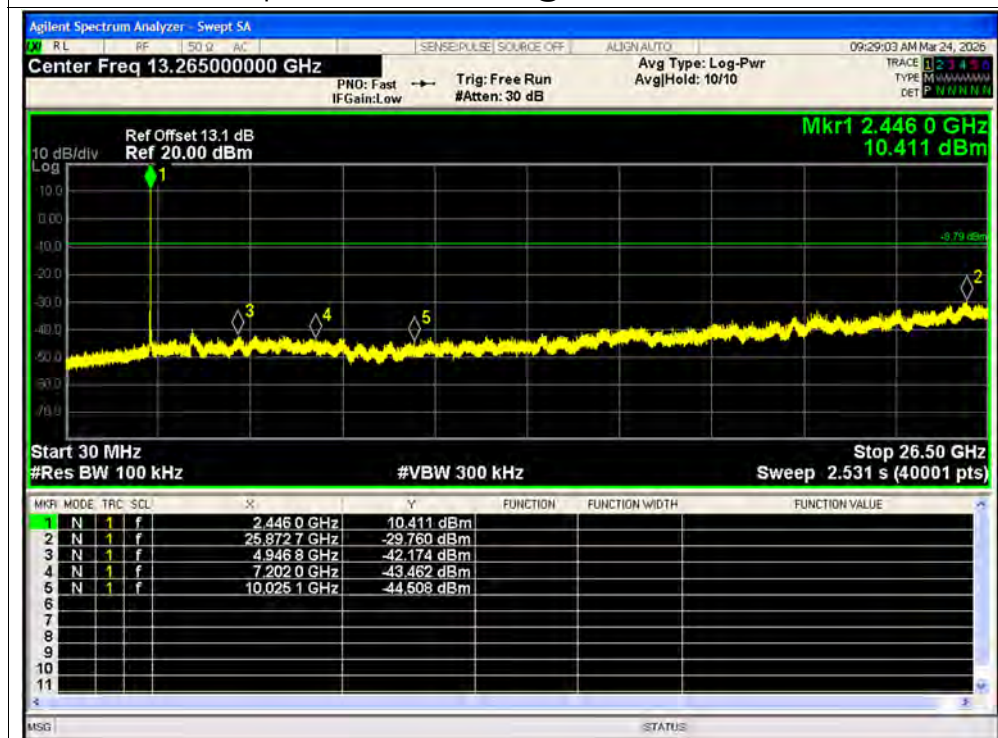
Tx. Spurious NVNT ax40 52@37 2462MHz Ant1 Emission
