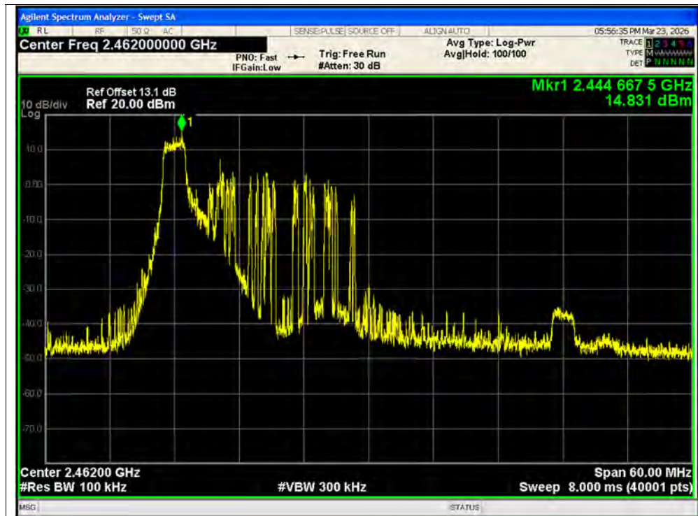
Tx. Spurious NVNT ax40 26@0 2462MHz Ant1 Ref
