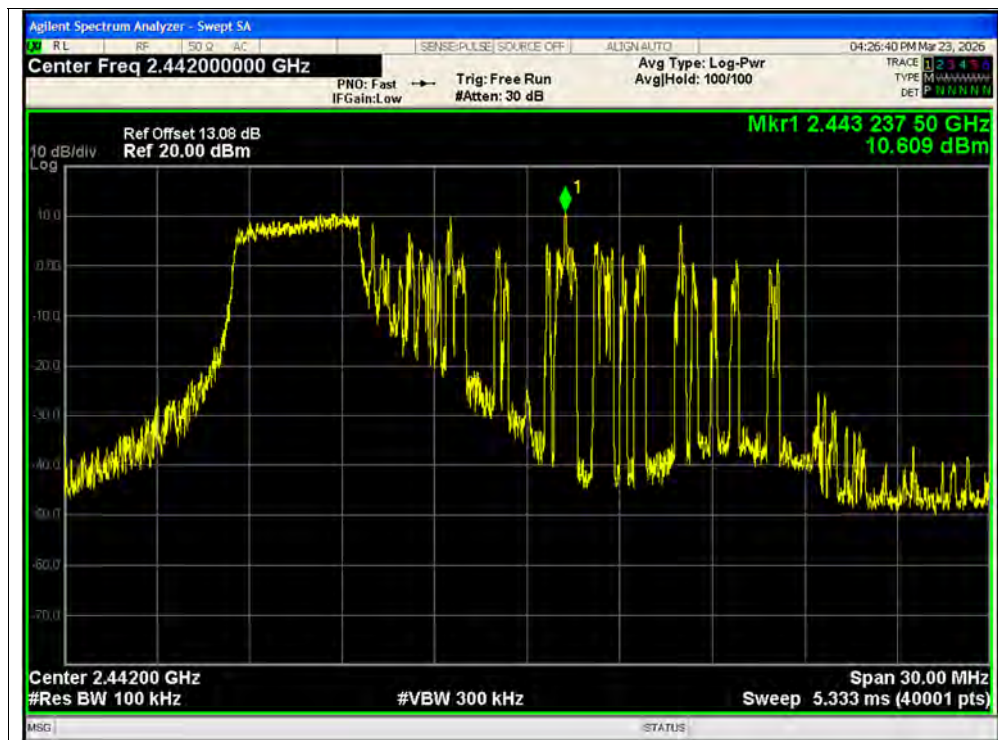
Tx. Spurious NVNT ax20 52@37 2442MHz Ant2 Ref
