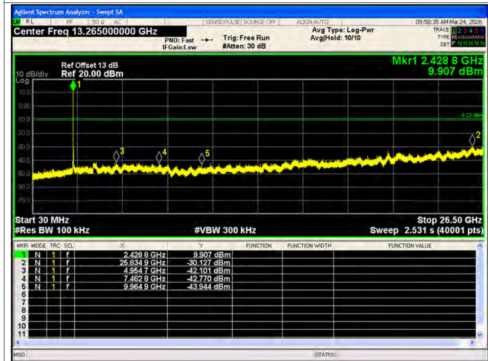
Tx. Spurious NVNT ax40 106@53 2442MHz Ant1 Emission
