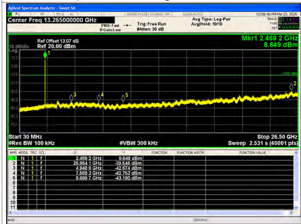
Tx. Spurious NVNT ax20 106@53 2472MHz Ant1 Emission
