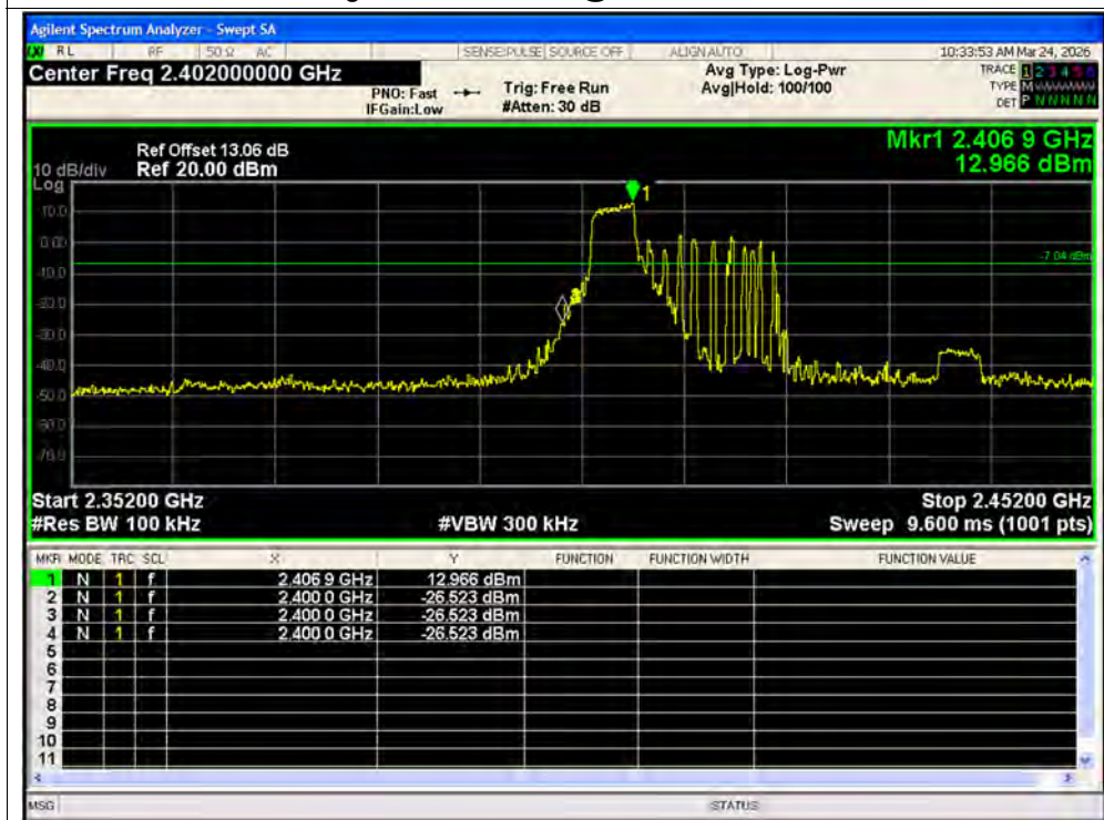
Band Edge NVNT ax40 52@37 2422MHz Ant2 Emission
