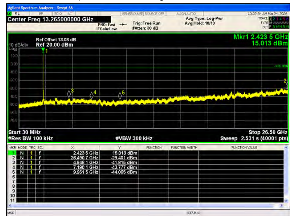
Tx. Spurious NVNT ax40 26@0 2442MHz Ant2 Emission
