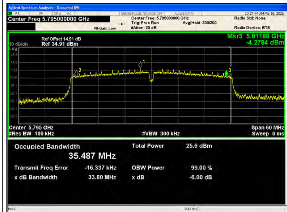
-6dB Bandwidth NVNT ac40 5795MHz Ant2 SISO
