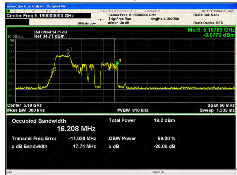
-26dB Bandwidth NVNT ax40 52@1 5190MHz Ant2 MIMO
