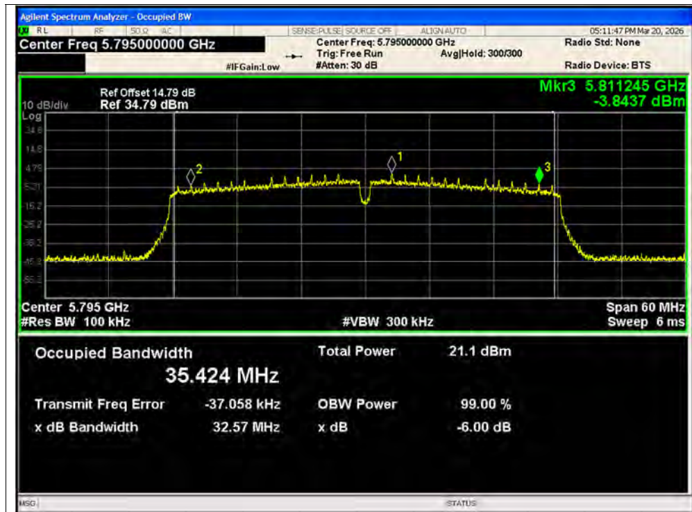
-6dB Bandwidth NVNT ac40 5795MHz Ant1 MIMO
