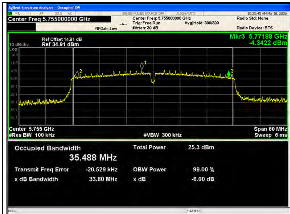
-6dB Bandwidth NVNT ac40 5755MHz Ant2 SISO
