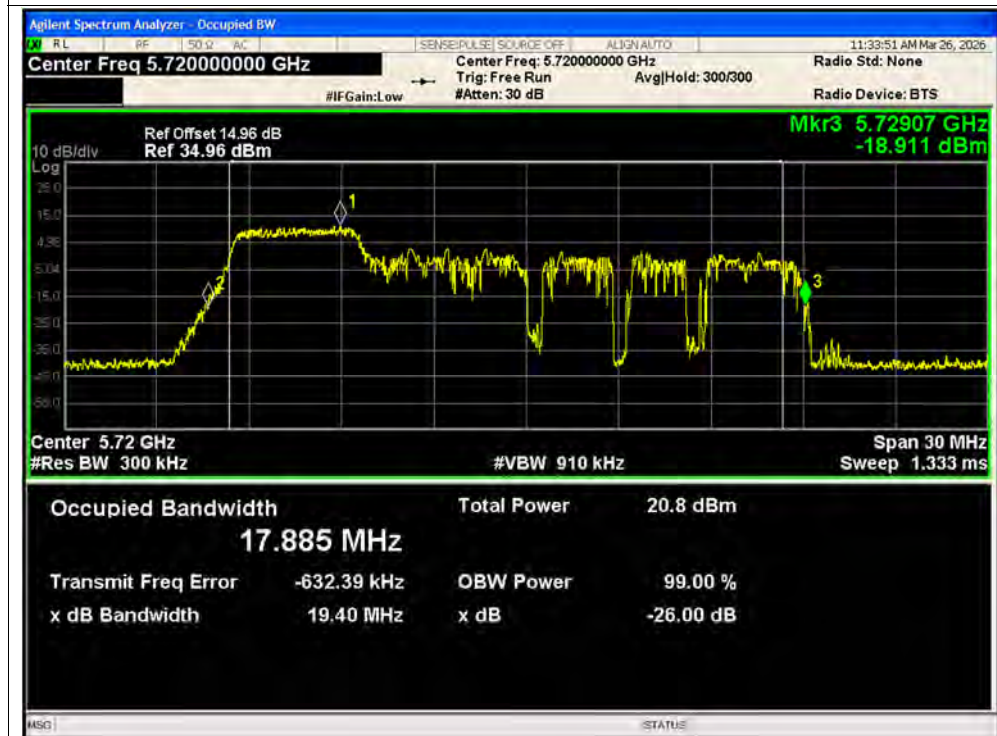
-26dB Bandwidth NVNT ax20 52@1 5720MHz Ant2 MIMO
