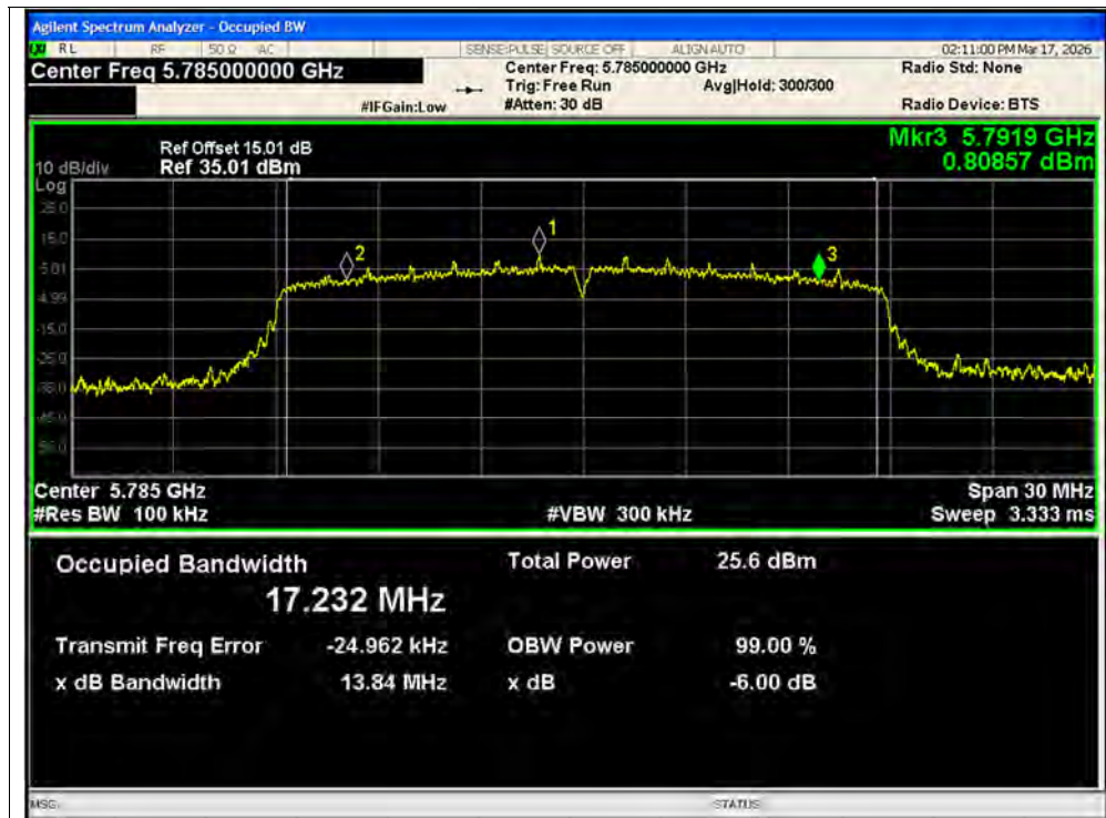
-6dB Bandwidth NVNT n20 5785MHz Ant2 SISO
