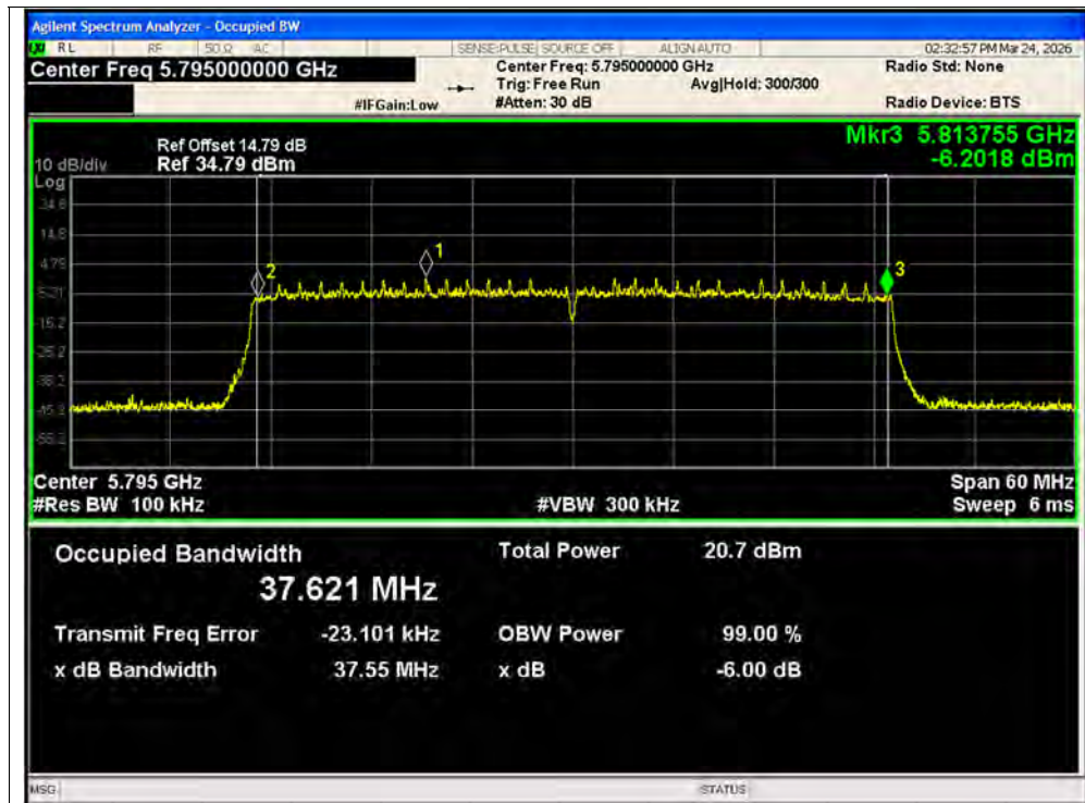
-6dB Bandwidth NVNT ax40 5795MHz Ant1 MIMO
