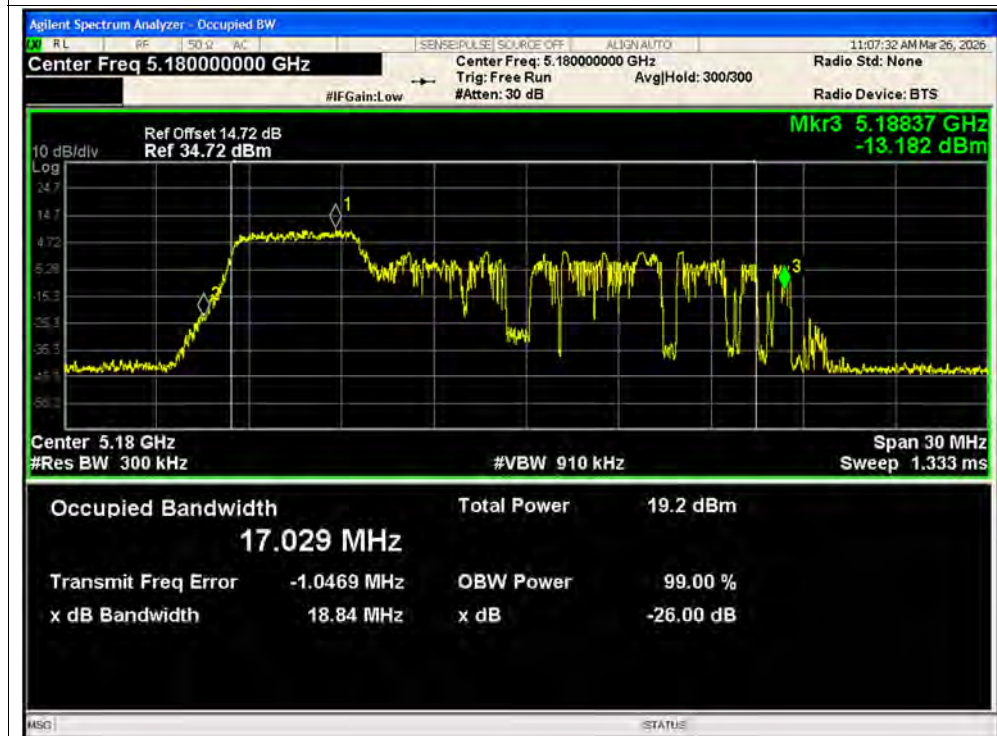
-26dB Bandwidth NVNT ax20 52@1 5180MHz Ant2 MIMO
