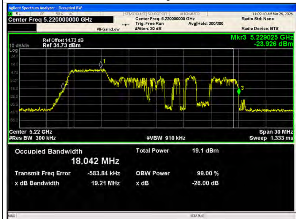
-26dB Bandwidth NVNT ax20 52@1 5220MHz Ant2 MIMO
