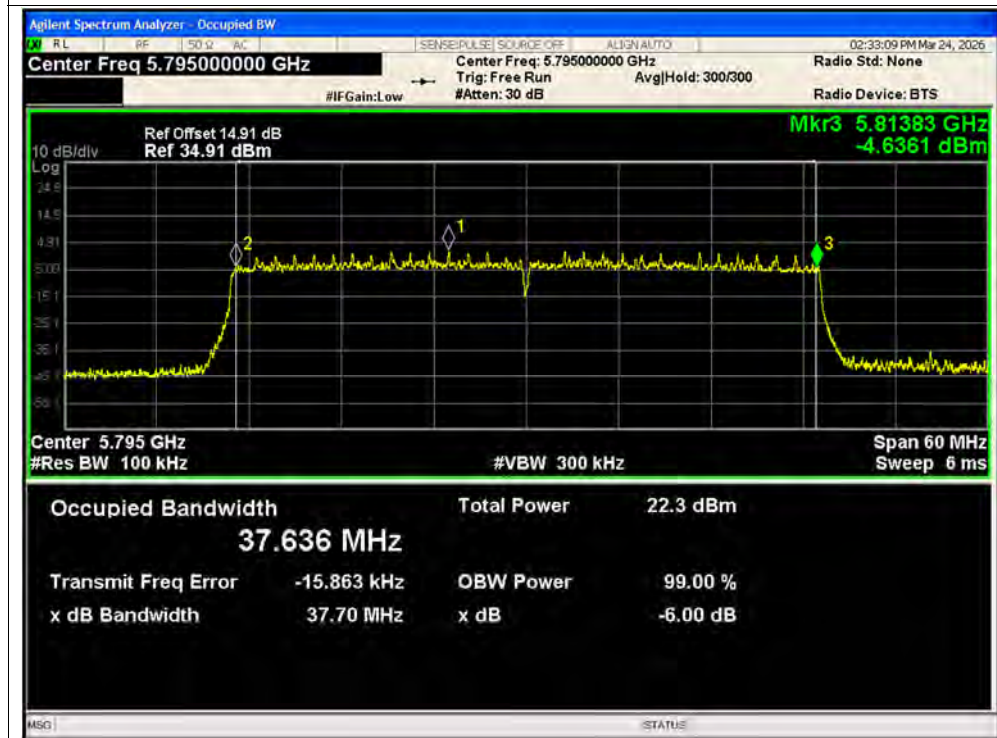
-6dB Bandwidth NVNT ax40 5795MHz Ant2 MIMO
