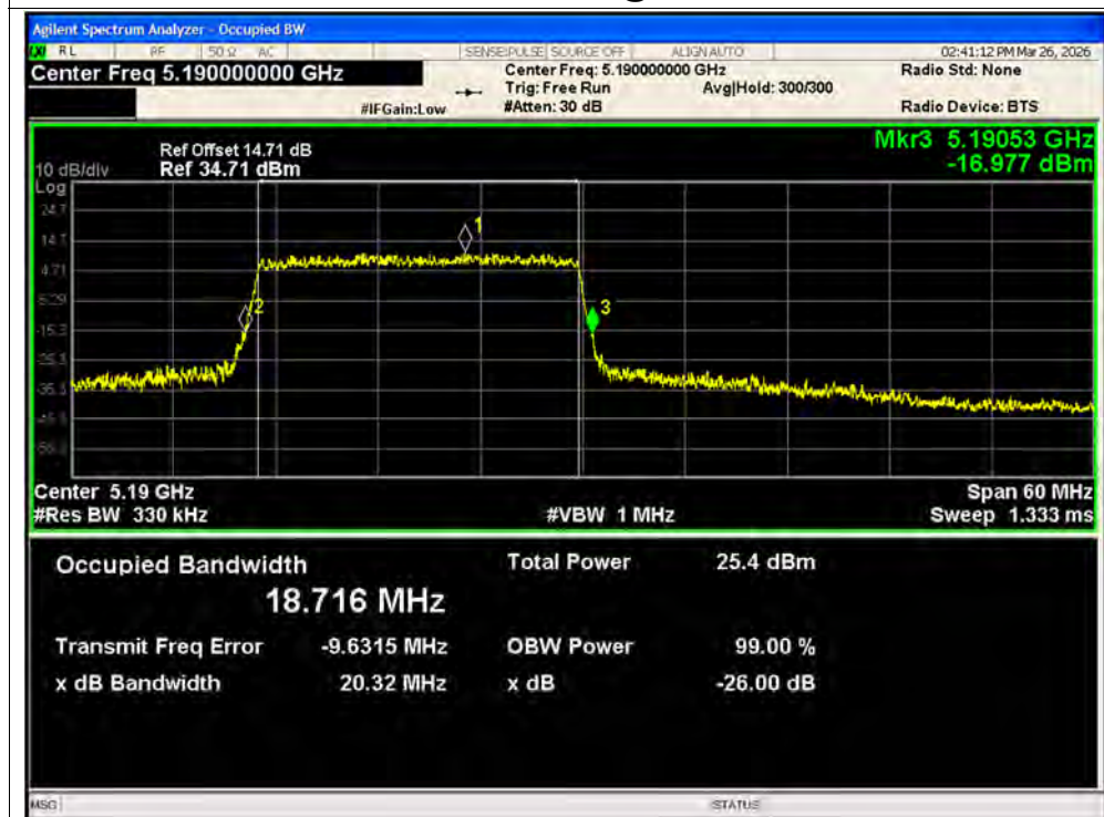
-26dB Bandwidth NVNT ax40 242@1 5190MHz Ant2 MIMO
