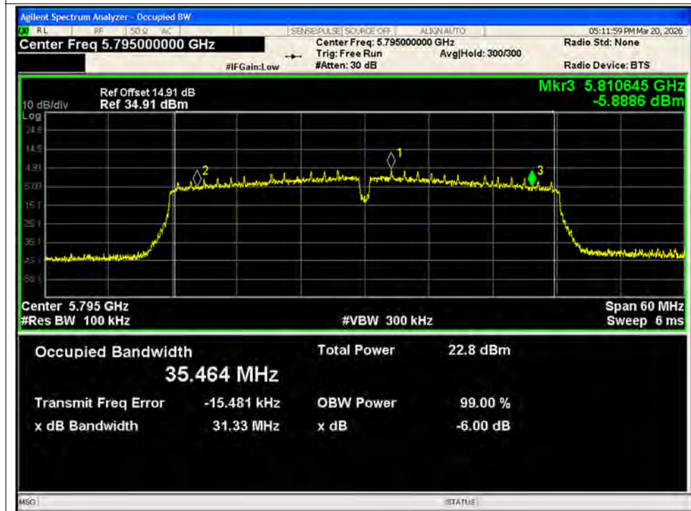
-6dB Bandwidth NVNT ac40 5795MHz Ant2 MIMO
