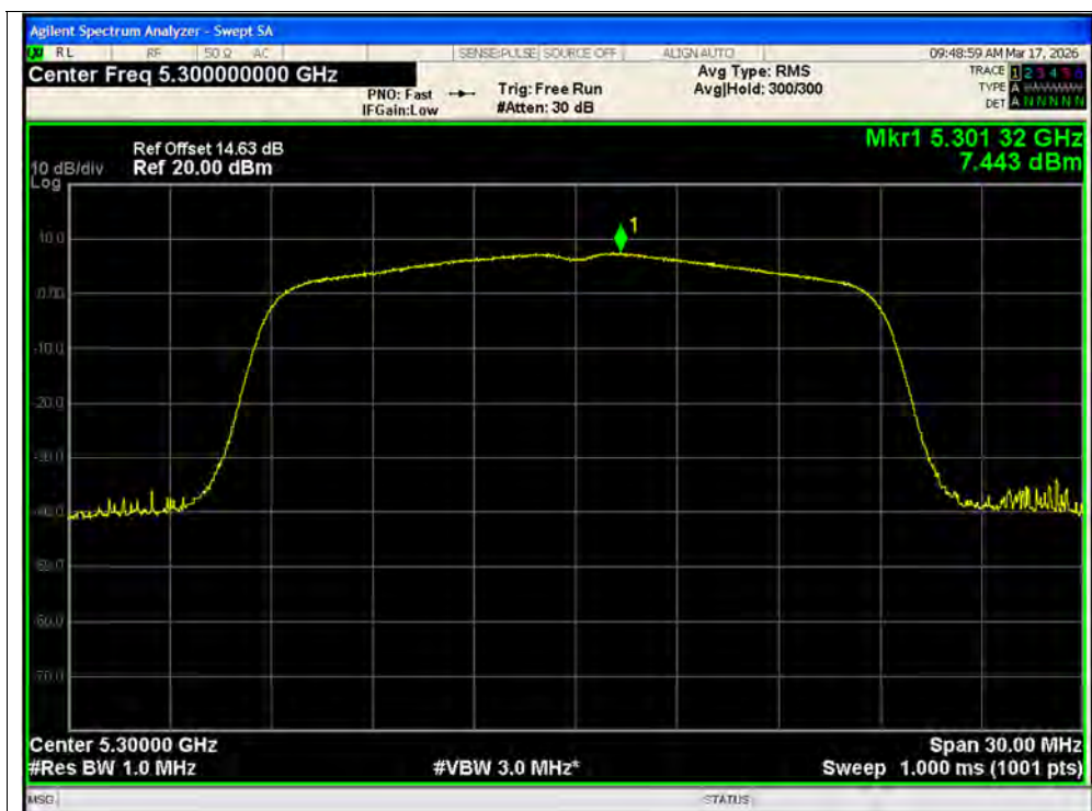
PSD NVNT ac20 5300MHz Ant1 SISO
