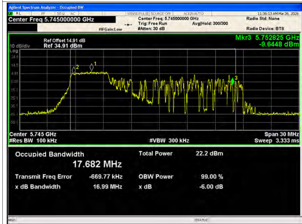
-6dB Bandwidth NVNT ax20 52@1 5745MHz Ant2 MIMO
