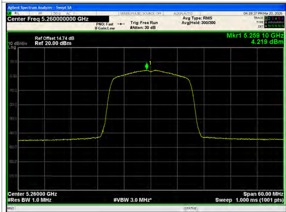
PSD NVNT ac20 5260MHz Ant2 MIMO
