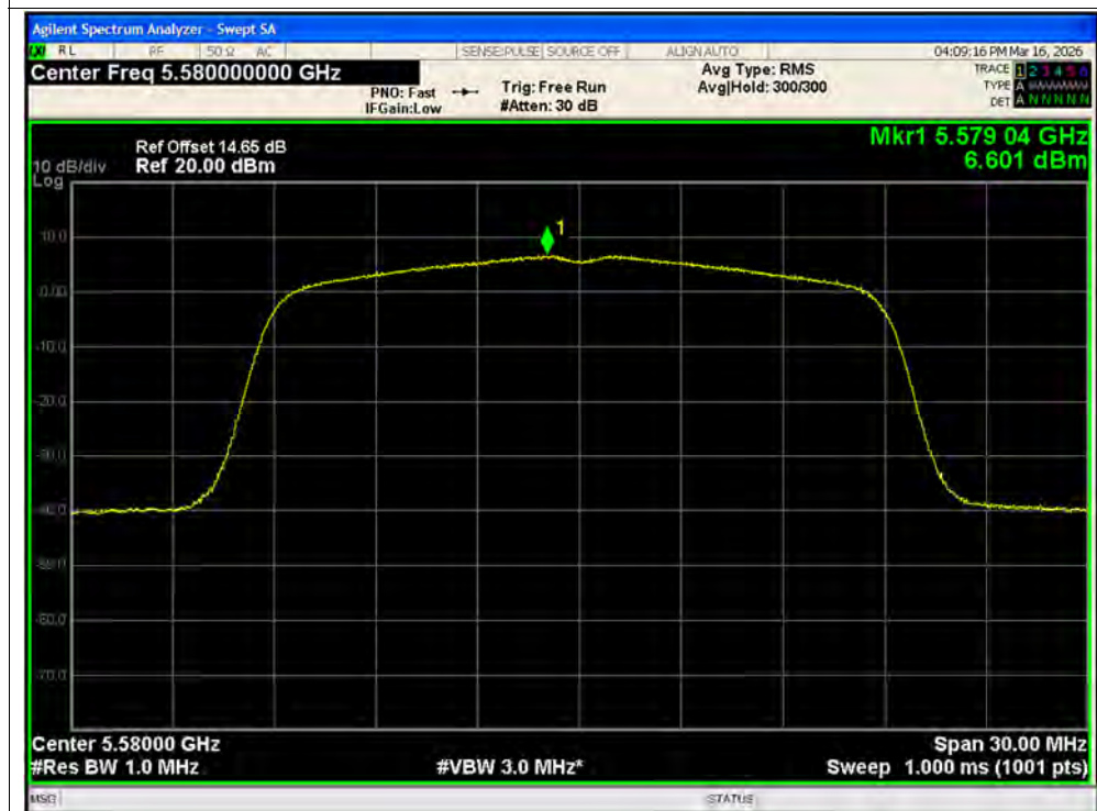
PSD NVNT n20 5580MHz Ant1 SISO
