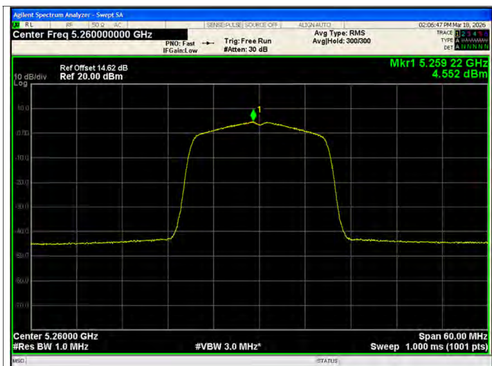
PSD NVNT n20 5260MHz Ant1 MIMO
