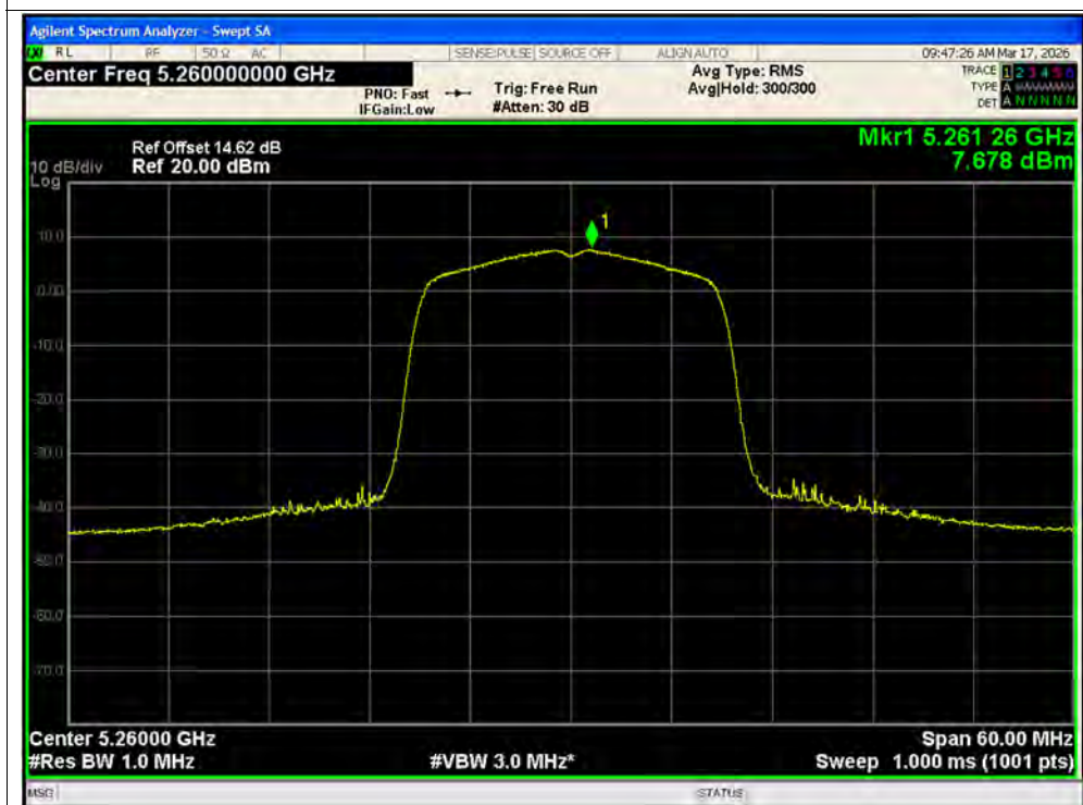
PSD NVNT ac20 5260MHz Ant1 SISO
