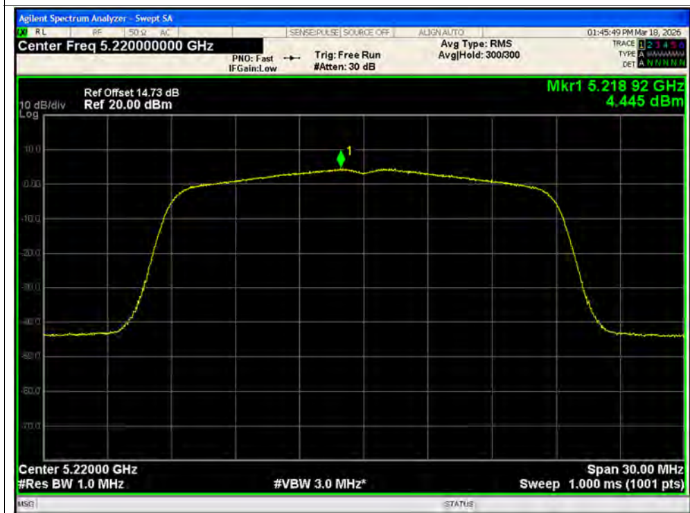
PSD NVNT n20 5220MHz Ant2 MIMO
