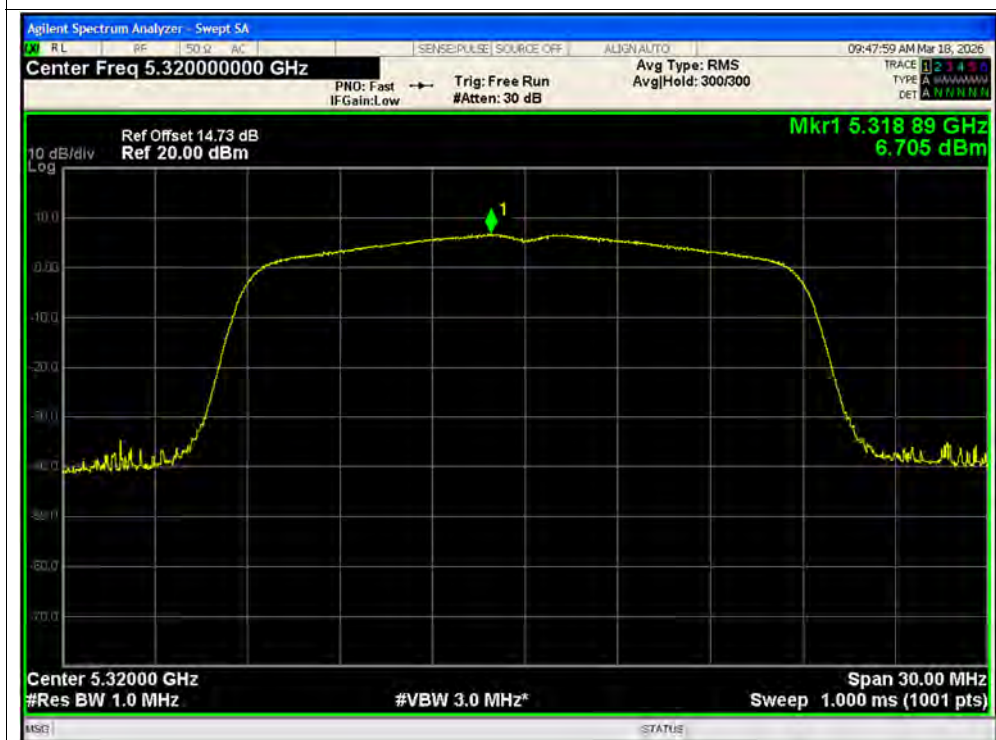
PSD NVNT ac20 5320MHz Ant2 SISO
