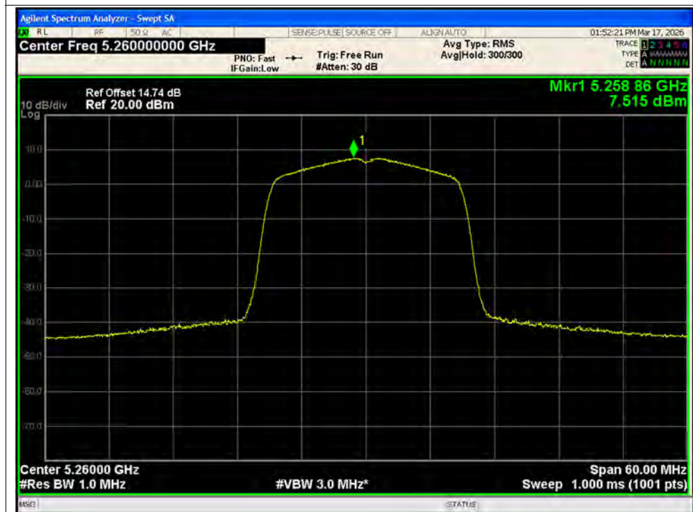
PSD NVNT n20 5260MHz Ant2 SISO
