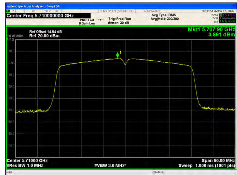
PSD NVNT n40 5710MHz Ant2 SISO
