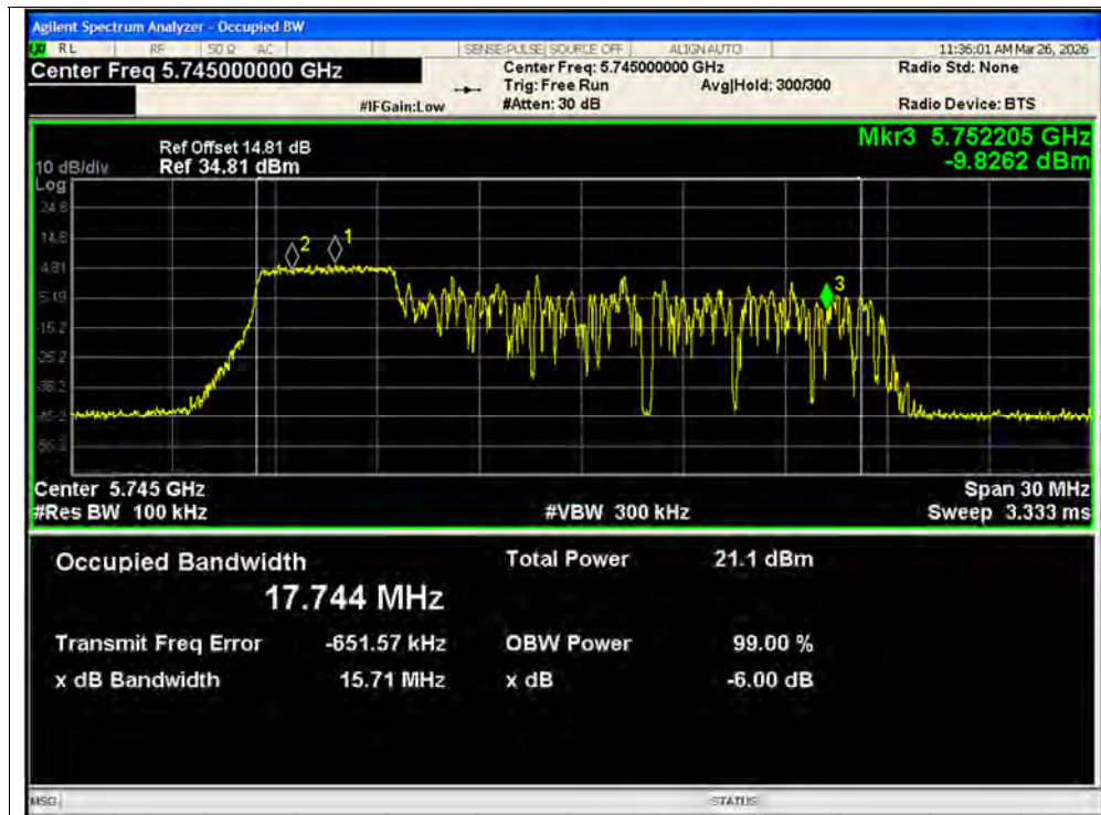
-6dB Bandwidth NVNT ax20 52@1 5745MHz Ant1 MIMO
