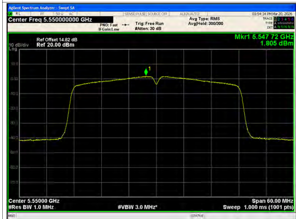
PSD NVNT n40 5550MHz Ant2 MIMO
