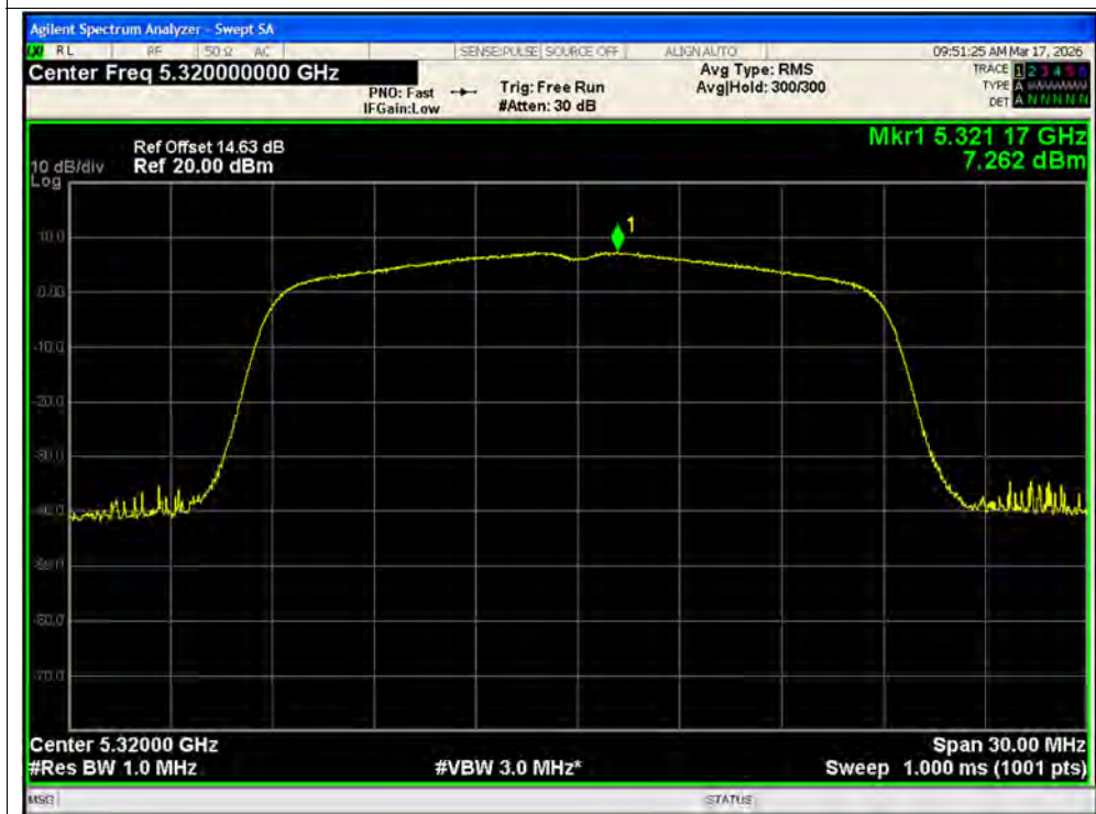
PSD NVNT ac20 5320MHz Ant1 SISO
