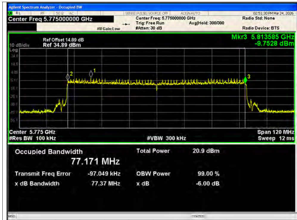
-6dB Bandwidth NVNT ax80 5775MHz Ant1 MIMO
