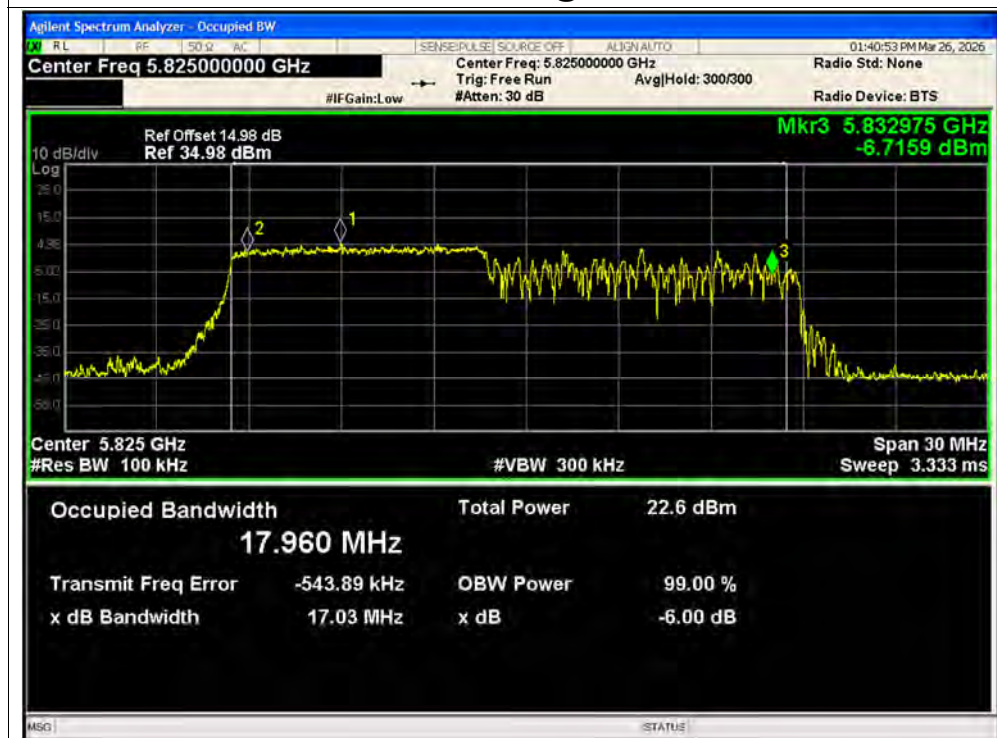
-6dB Bandwidth NVNT ax20 106@1 5825MHz Ant2 MIMO
