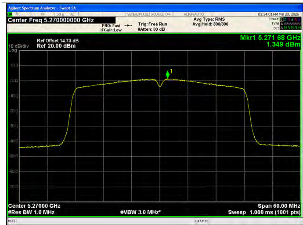
PSD NVNT n40 5270MHz Ant2 MIMO
