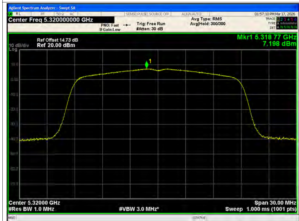
PSD NVNT n20 5320MHz Ant2 SISO
