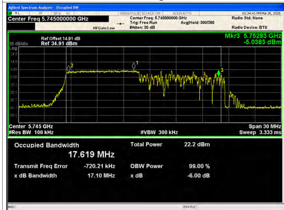
-6dB Bandwidth NVNT ax20 106@1 5745MHz Ant2 MIMO
