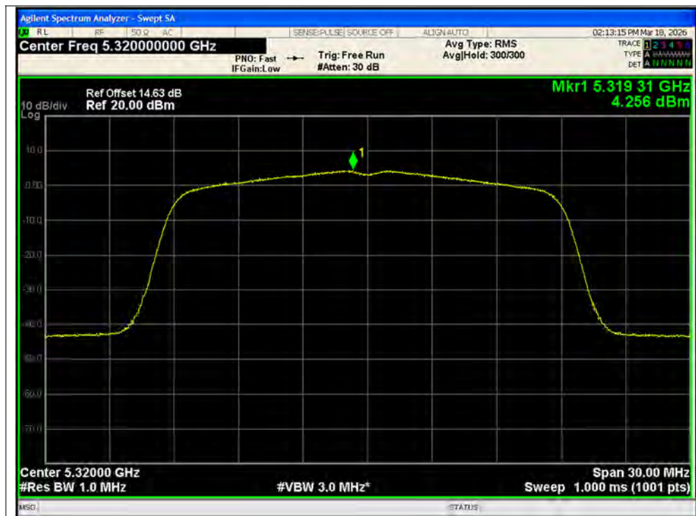
PSD NVNT n20 5320MHz Ant1 MIMO
