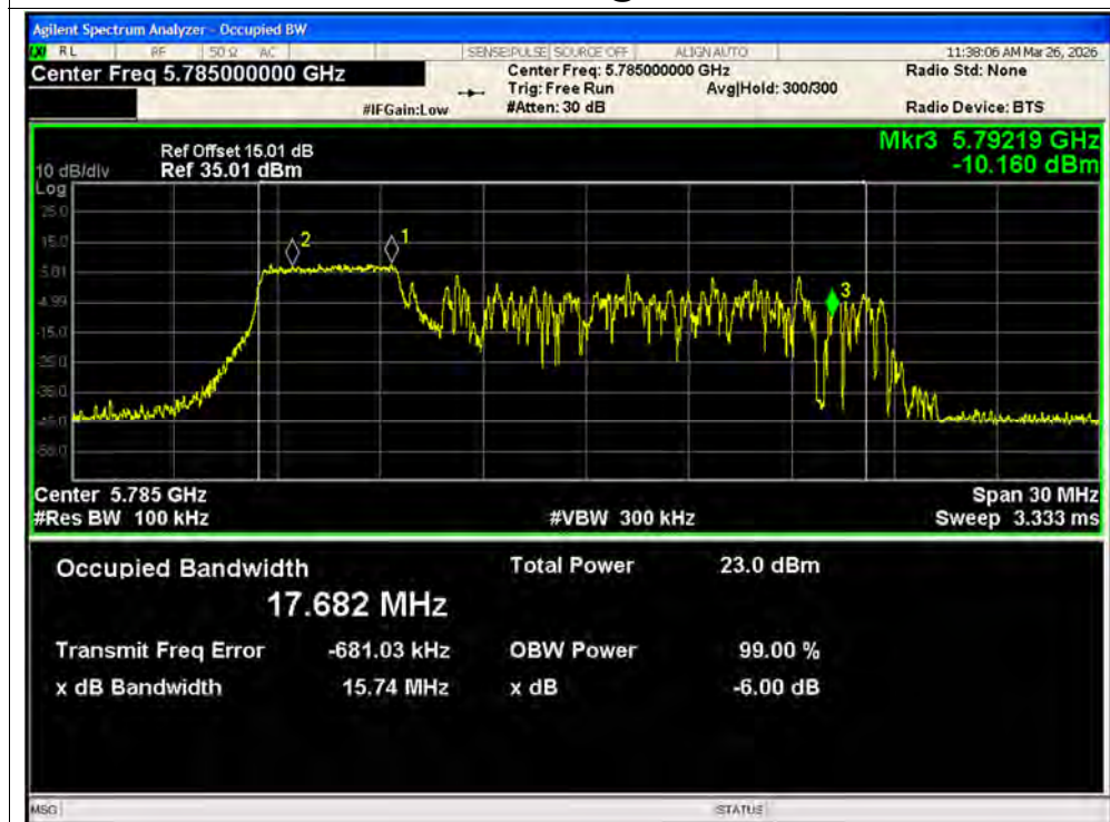
-6dB Bandwidth NVNT ax20 52@1 5785MHz Ant2 MIMO
