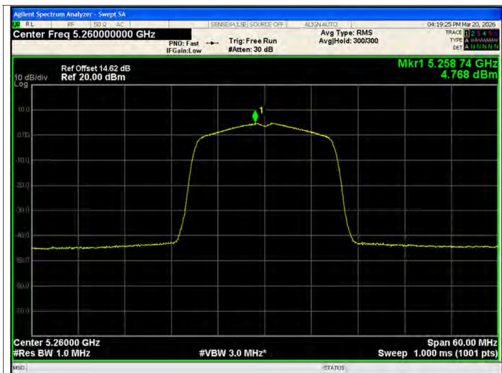
PSD NVNT ac20 5260MHz Ant1 MIMO
