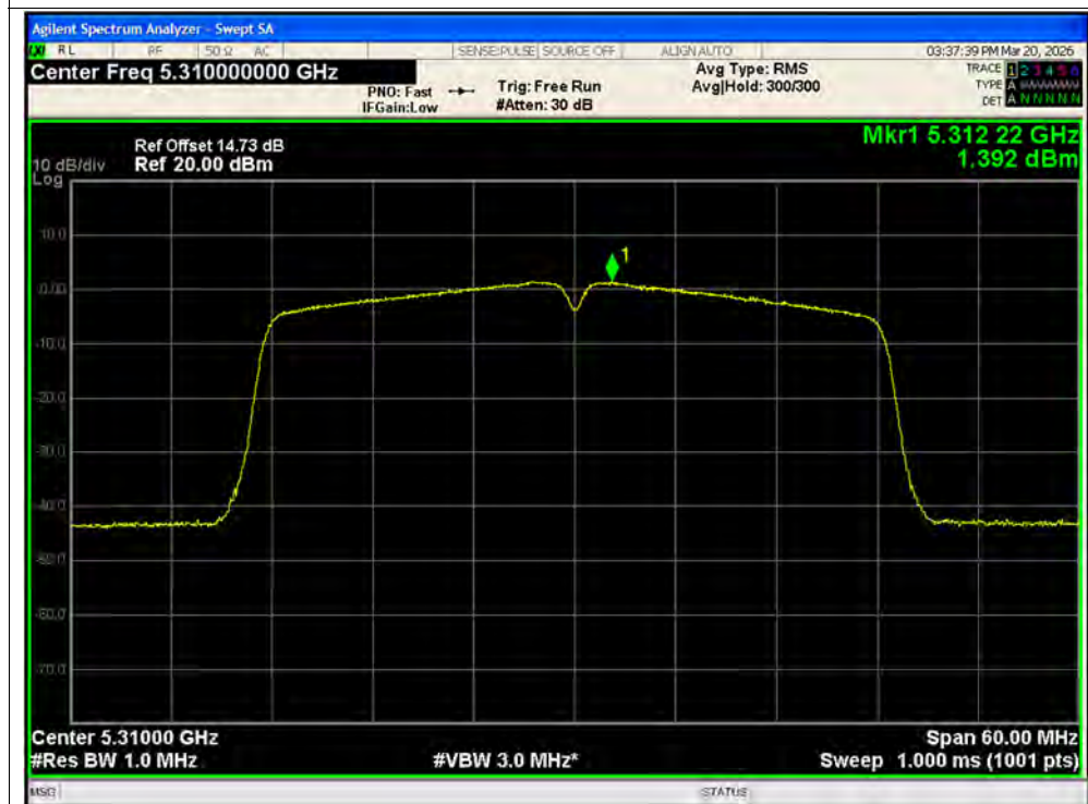
PSD NVNT n40 5310MHz Ant2 MIMO
