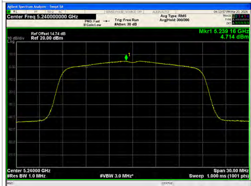
PSD NVNT ac20 5240MHz Ant2 MIMO
