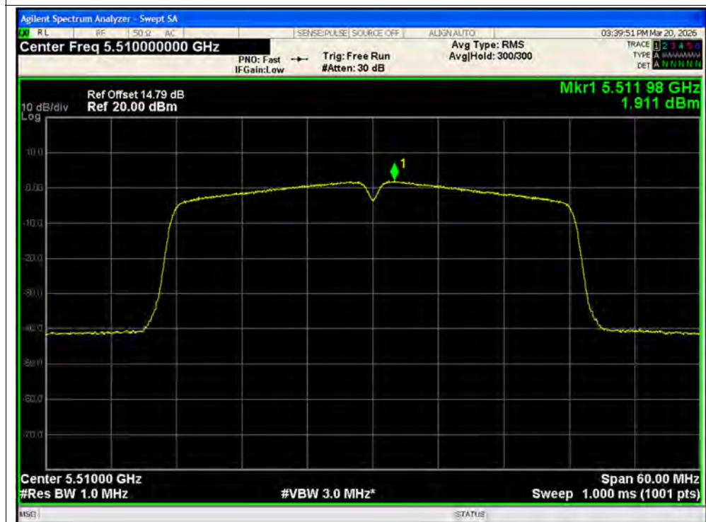
PSD NVNT n40 5510MHz Ant2 MIMO
