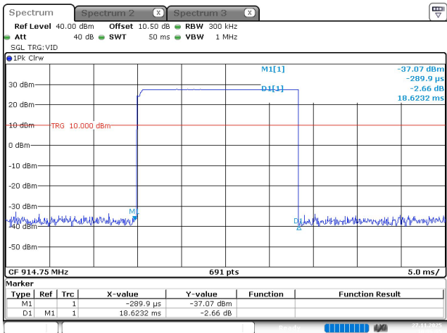
Pulse width=18.623ms
